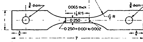
b Unstretched Tensile Test Specimen
