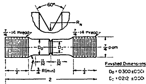
o Notched Tensile Test Specimen ( K_t = 3.0 )
