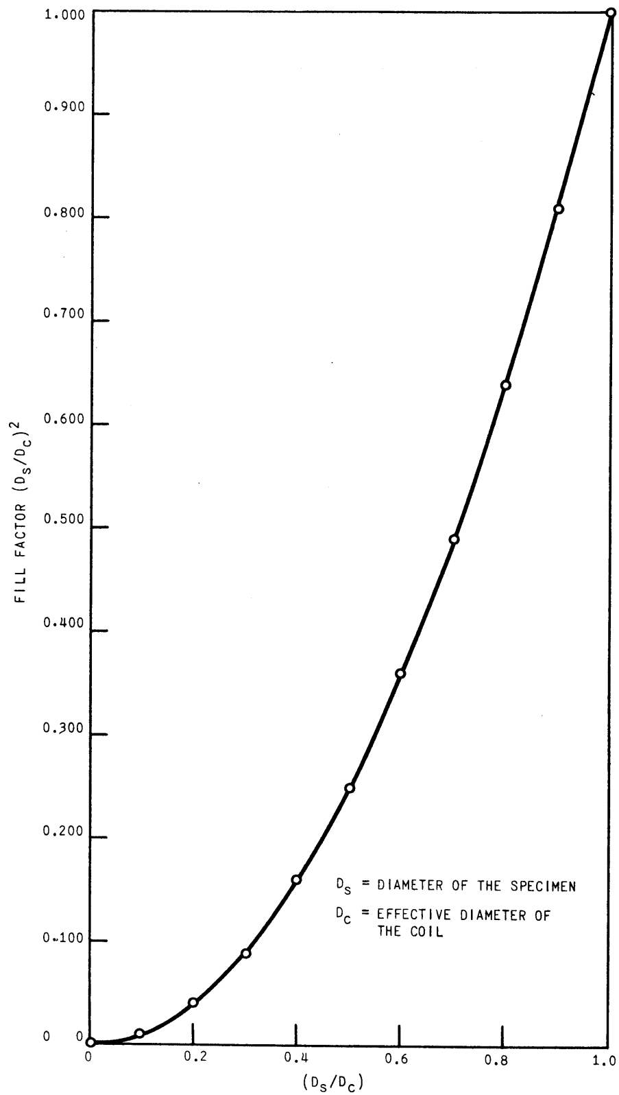
Figure A-3. FILL FACTOR VERSUS (D_s/D_c)^2
