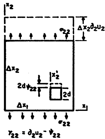
Figure 1. Typical components of relative stress \sigma_{ij} , displacement-gradient \partial_{iuj} , micro-deformation \psi_{ij} and relative deformation \gamma_{ij}
