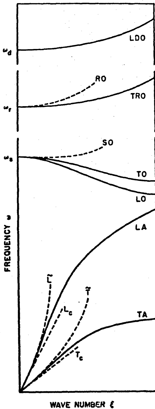
Figure 3. Sketch of possible configuration of real branches of dispersion curves.
