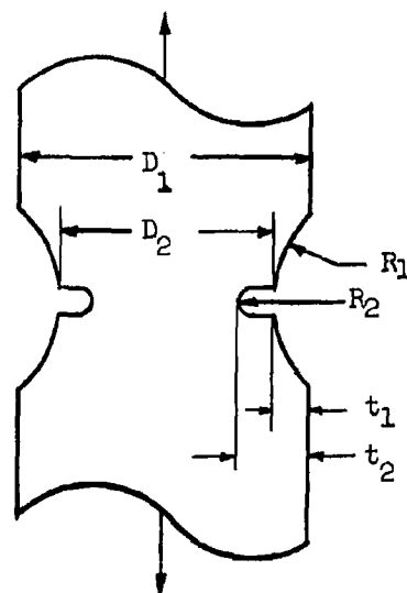
SPECIMEN CONFIGURATION
