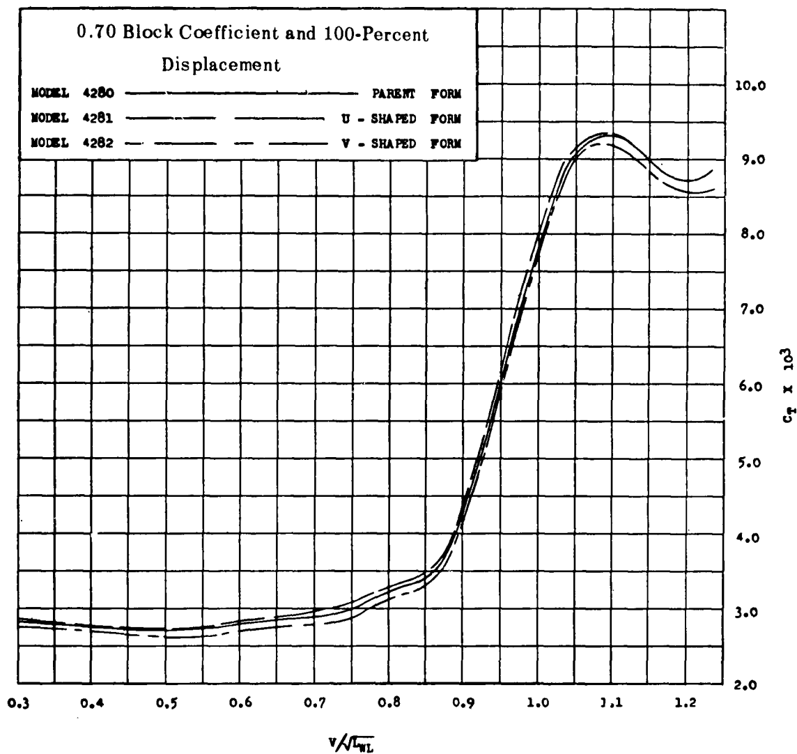
Figure 62 - Curves of Resistance Coefficient C_T to a Base of \frac{V}{\sqrt{L_{WL}}} for Series 60, 0.70 C_B Models
