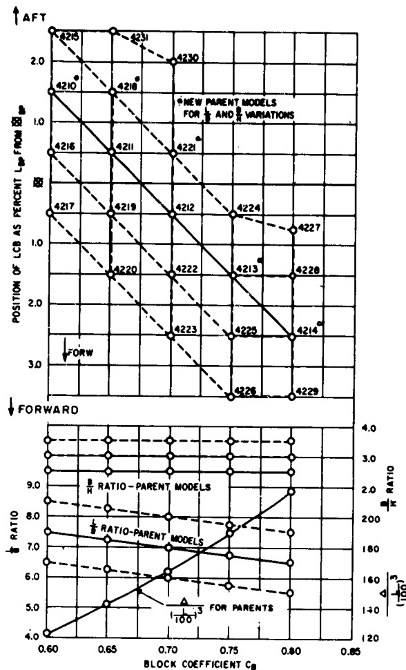
Figure 1 - Variation of Proportions etc., with C_B
