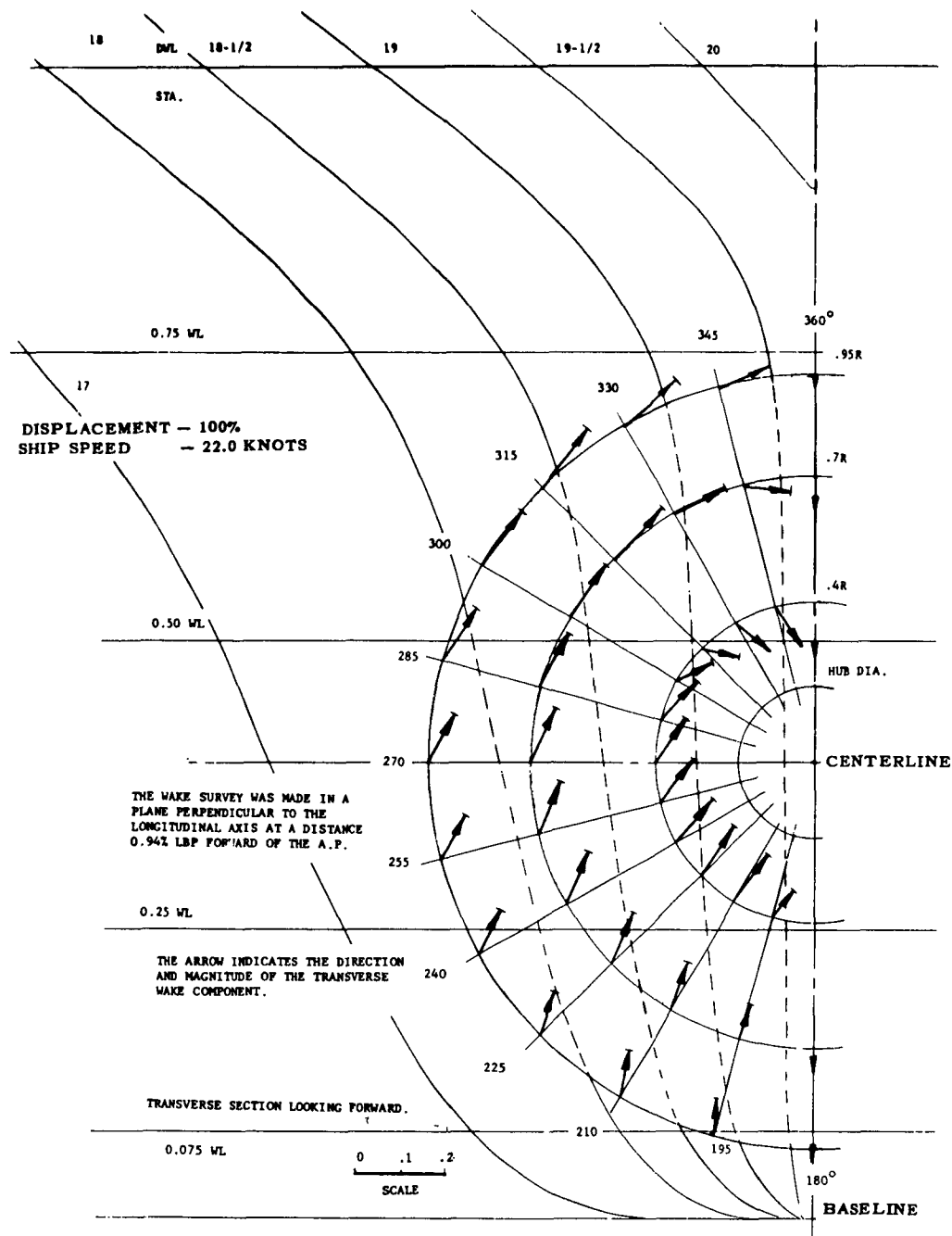
Figure 81 - Wake Diagram for Model 4210- C_B = 0.60
