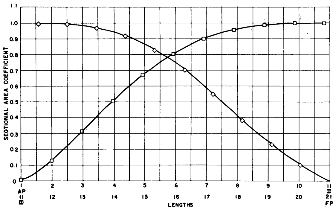
Figure D1 – Area Curves for Series 60 Equivalent of SCHUYLER OTIS BLAND
