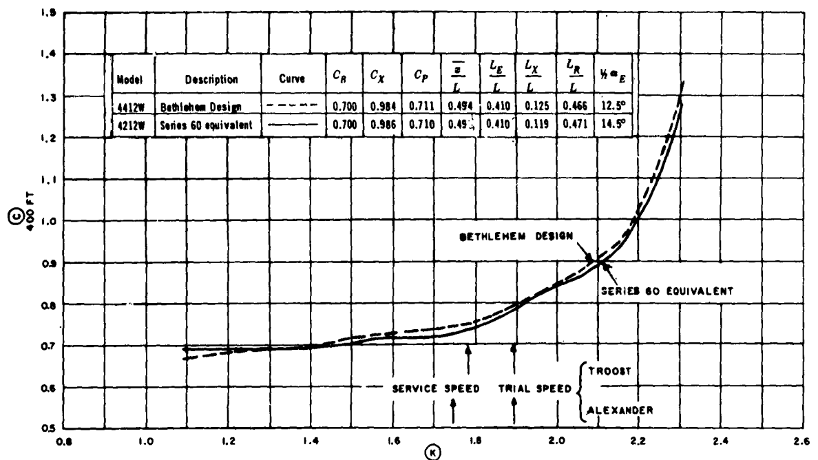
Figure 25d — Comparison, Series 60 and Bethlehem. 0.70 Design
