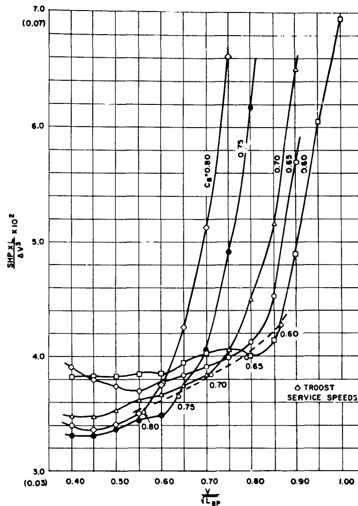
Figure 94 - \frac{SHP \cdot L}{\Delta V^3} on \frac{V}{\sqrt[6]{L}} for Series 60 Parents
