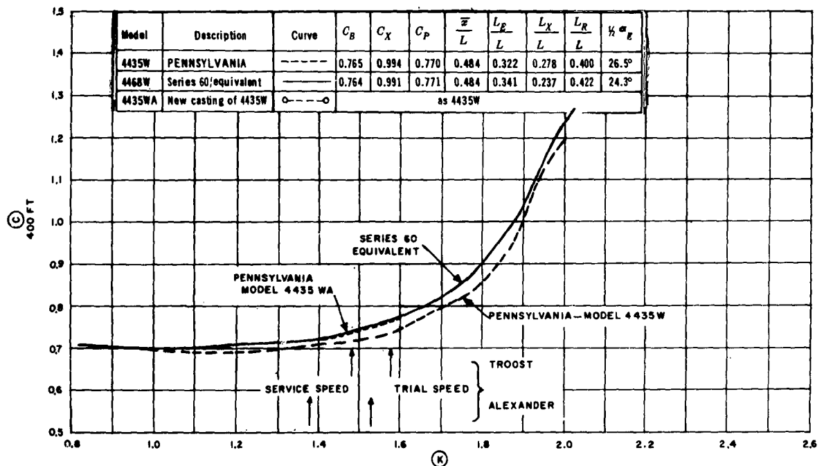
Figure 25e — Comparison, Series 60 and PENNSYLVANIA
