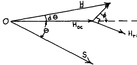
Figure IV.1. A vector diagram of the various fields in a typical experimental arrangement. H_{dc} is the external magnetic field, H_m is the modulation magnetic field, H_{rf} is the microwave magnetic field and S is the symmetry axis of the crystal exhibiting electron resonance.
