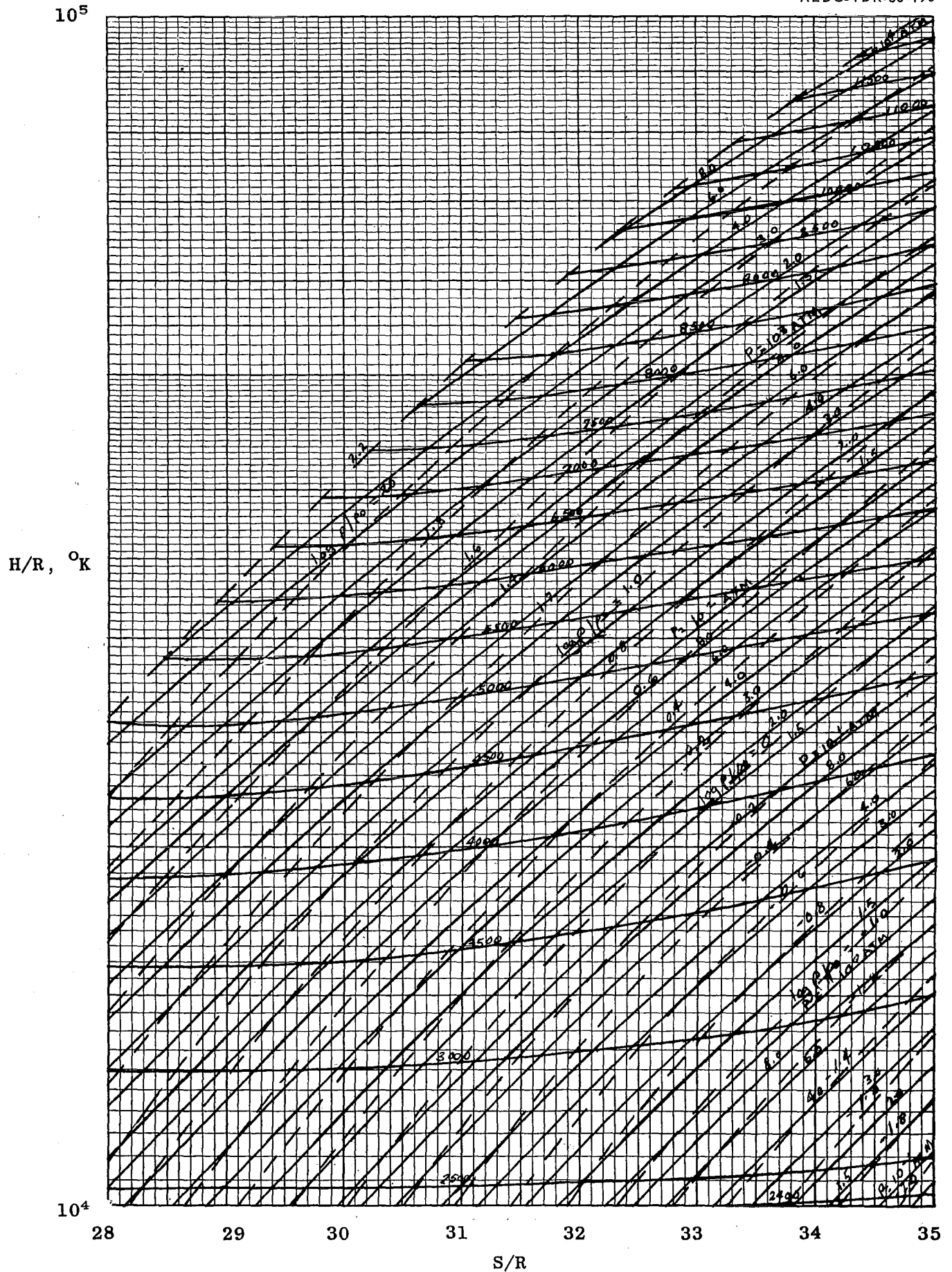
Fig. 7 Air Mollier Diagram
