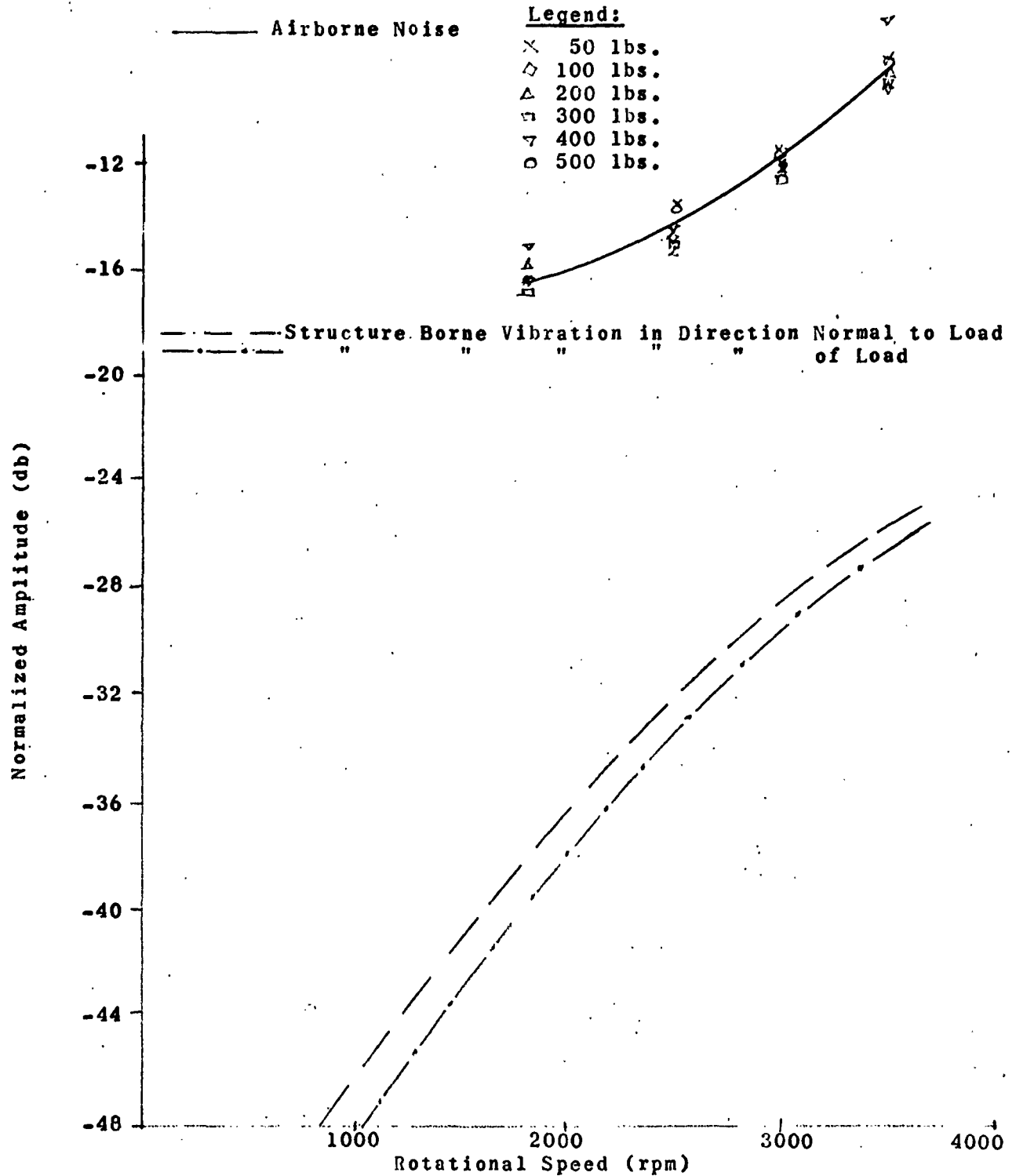
ENCLOSURE 25 . AMPLITUDE OF AIRBORNE NOISE (AND STRUCTURE BORNE VIBRATIONS) AS A FUNCTION OF RADIAL LOAD AND ROTATIONAL SPEED (6400-12800 cps FREQUENCY RANGE)
