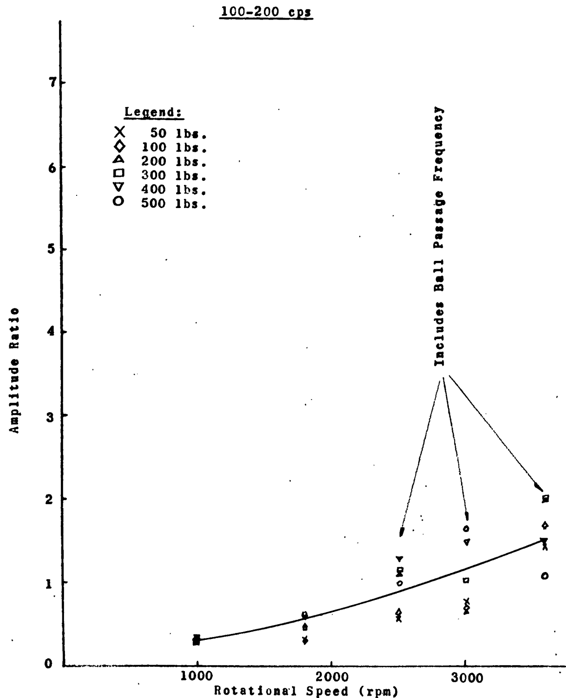
ENCLOSURE 10 STRUCTURE BORNE VIBRATION OF 6310 BEARINGS IN DIRECTION OF LOAD AS A FUNCTION OF RADIAL LOAD AND ROTATIONAL SPEED (100-200 cps FREQUENCY RANGE)
