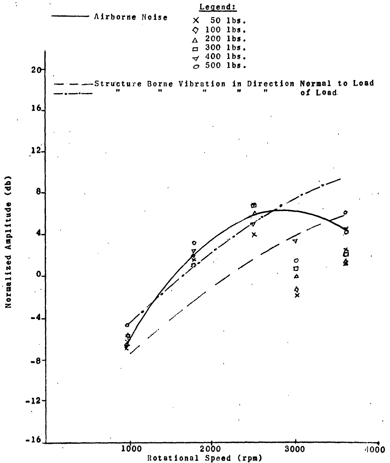
ENCLOSURE 20 AMPLITUDE OF AIRBORNE NOISE (AND STRUCTURE BORNE VIBRATIONS) AS A FUNCTION OF RADIAL LOAD AND ROTATIONAL SPEED (200-400 cps FREQUENCY RANGE)
