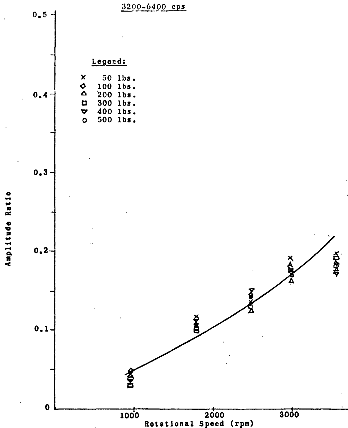
ENCLOSURE 7 STRUCTURE BORNE VIBRATION OF 6310 BEARINGS IN DIRECTION NORMAL TO LOAD AS A FUNCTION OF RADIAL LOAD AND ROTATIONAL SPEED (3200-6400 cps FREQUENCY RANGE)
