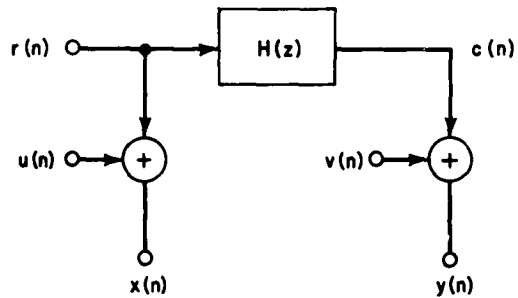
Fig. 1. The Model Assumed for Estimation of the Pulse Transfer Function
