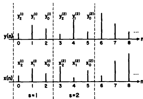
Fig. 2. Arrangement of the Observed Points for K = 2 .
