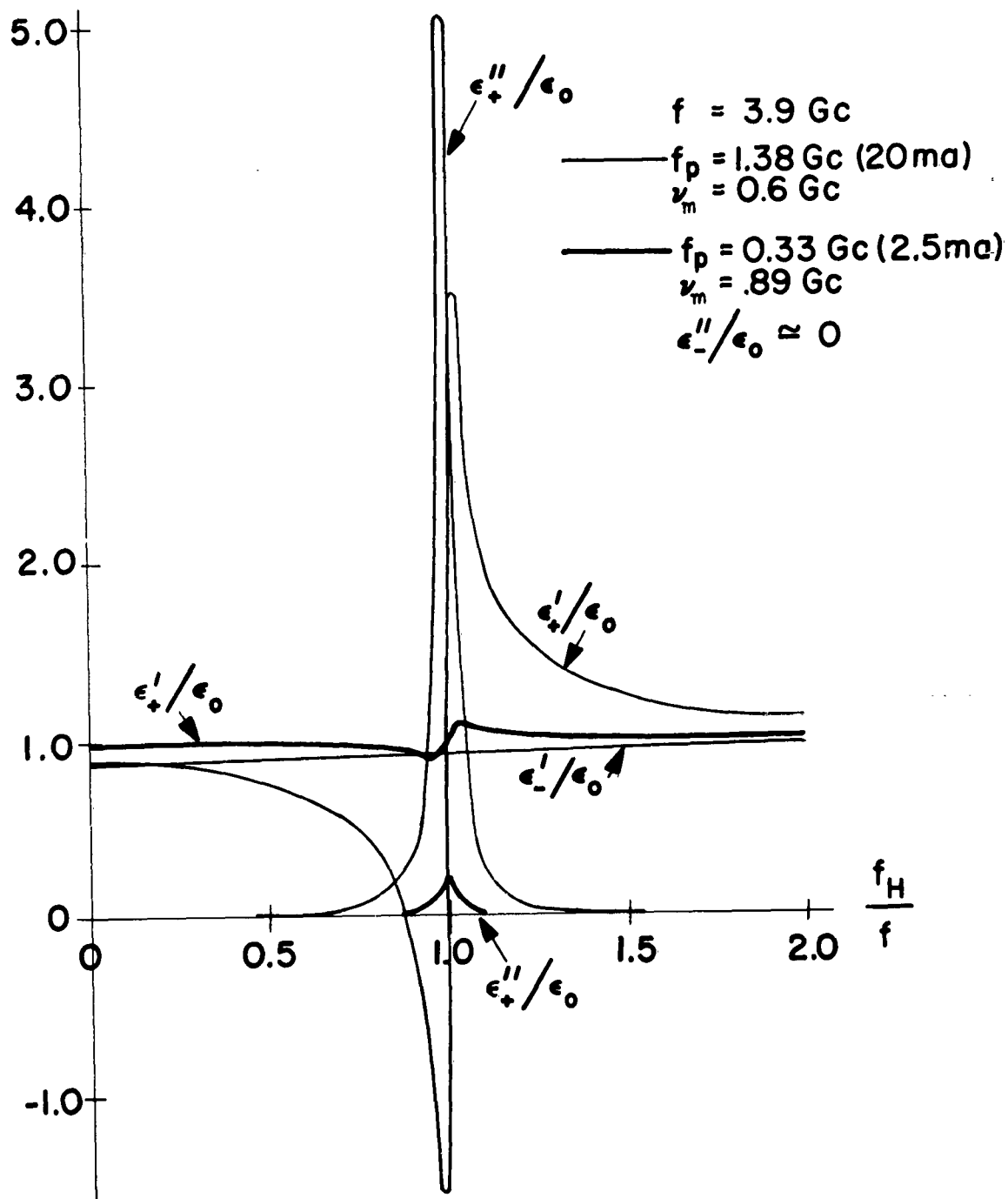
FIG. 3.16: RELATIVE PERMITTIVITY FOR ORDINARY AND EXTRAORDINARY WAVES AS A FUNCTION OF CYCLOTRON FREQUENCY
