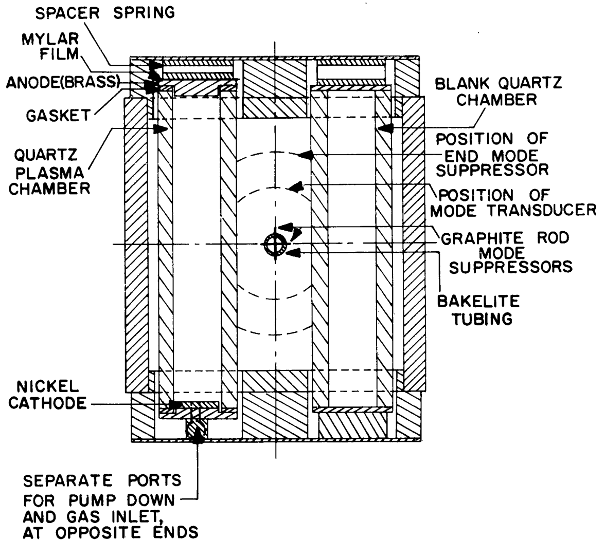
FIG. 3.2b: CROSS SECTION VIEW OF ISOLATOR
