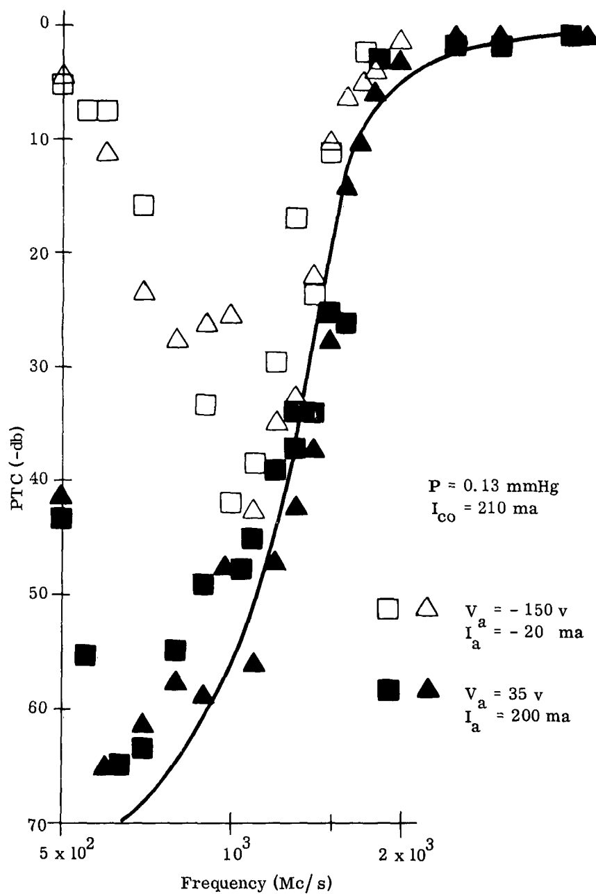
FIG. 2.7: POWER TRANSMISSION COEFFICIENT VS FREQUENCY IN ARGON DISCHARGE. SOLID LINE IS THEORETICAL CURVE FOR f_p = 1500 \text{ Mc} and \nu_m = 200 \text{ Mc} .
