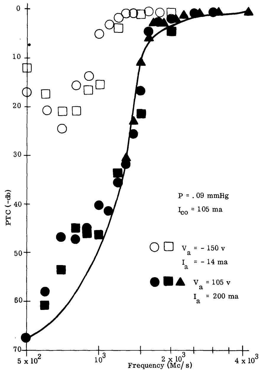
FIG. 2.9: POWER TRANSMISSION COEFFICIENT VS FREQUENCY IN NITROGEN DISCHARGE. SOLID LINE IS THEORETICAL CURVE FOR f_p = 1400 \text{ Mc} AND \nu_m = 150 \text{ Mc} .
