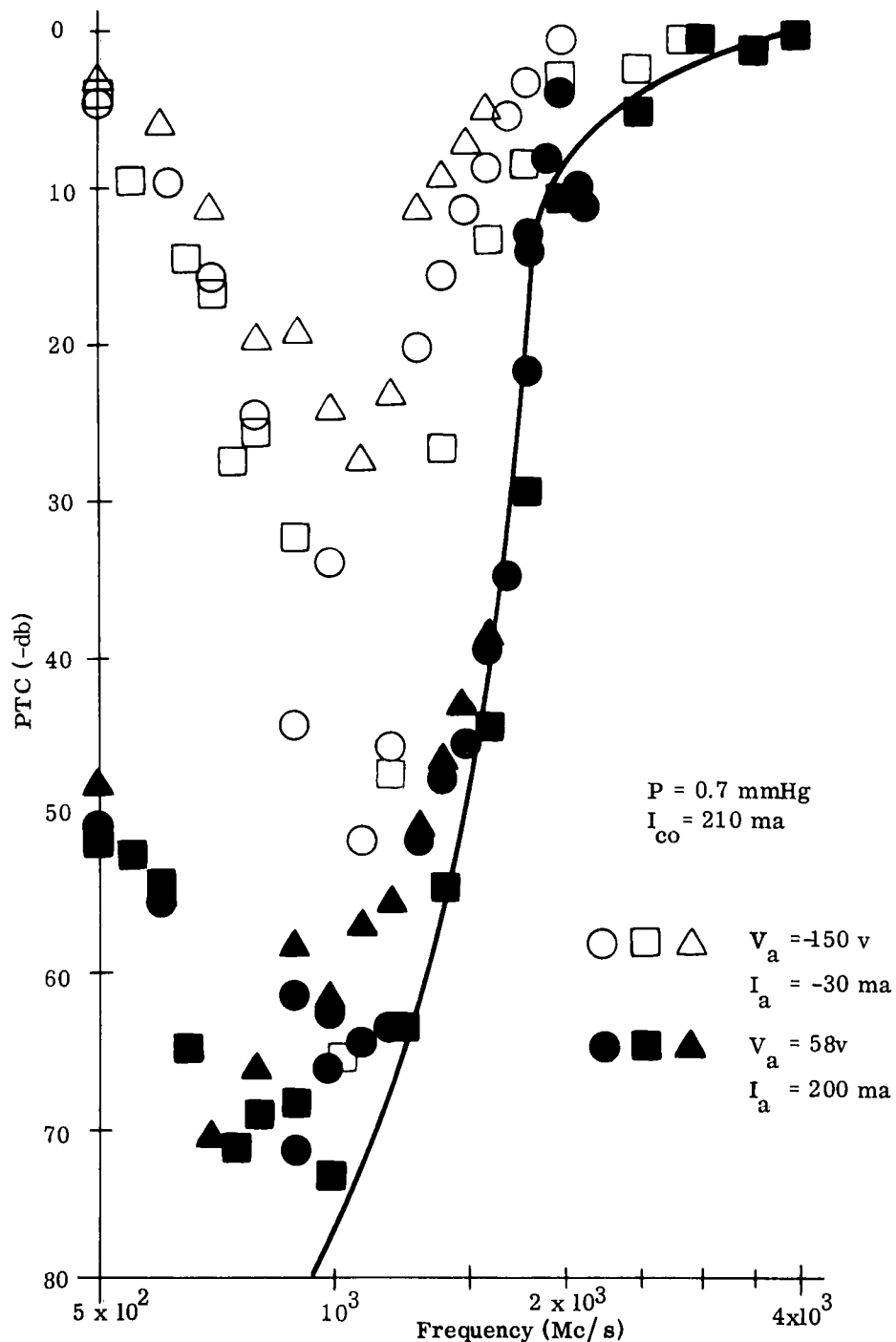
FIG. 2.8: POWER TRANSMISSION COEFFICIENT VS FREQUENCY IN HELIUM DISCHARGE. SOLID LINE IS THEORETICAL CURVE FOR f_p = 1800 \text{ Mc} AND \nu_m = 145 \text{ Mc} .
