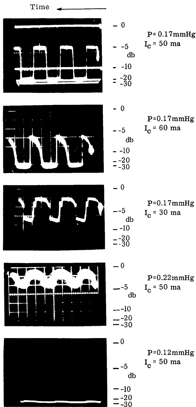
FIG. 2.16: STUDY OF 500 cps ENVELOPE IN 1000 Mc RF WITH NITROGEN DISCHARGE PRESSURE AND CATHODE CURRENT AS VARIABLES
