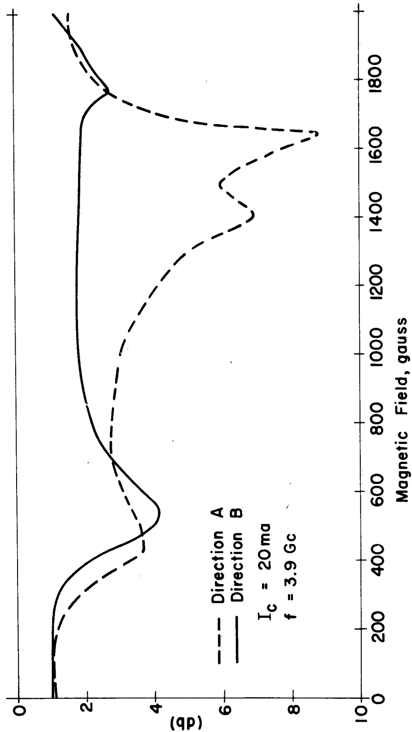
FIG. 3.15: POWER ABSORBED BY ISOLATION IN BOTH DIRECTIONS AS A FUNCTION OF MAGNETIC FIELD STRENGTH
