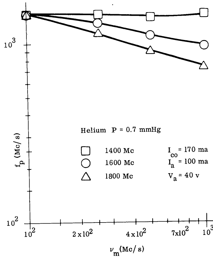
FIG. 2.10: SAMPLE f_p - \nu_n PLOT TO DETERMINE PLASMA FREQUENCY AND MOMENTUM TRANSFER COLLISION FREQUENCY FROM RF DATA
