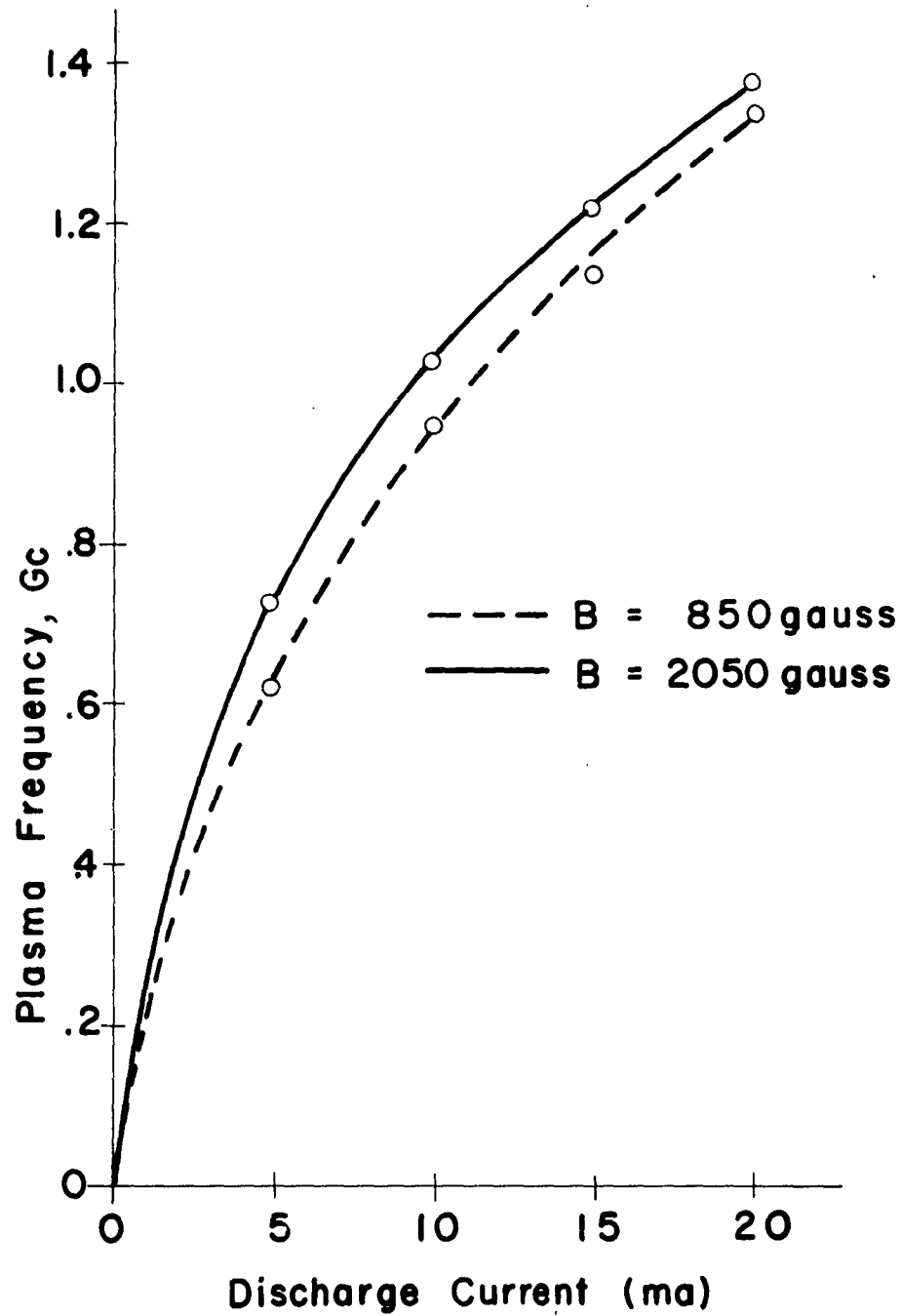
FIG. 3.5: ISOLATOR PLASMA FREQUENCY VS DISCHARGE CURRENT
