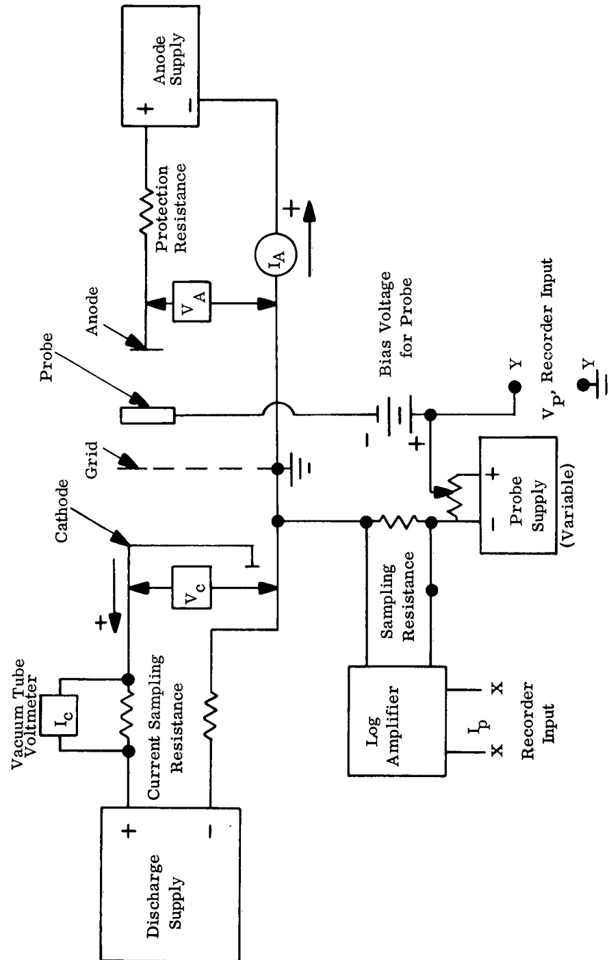
FIG. 2.6: CATHODE, ANODE AND PROBE SUPPLY CIRCUITS AND METERING ARRANGEMENTS
