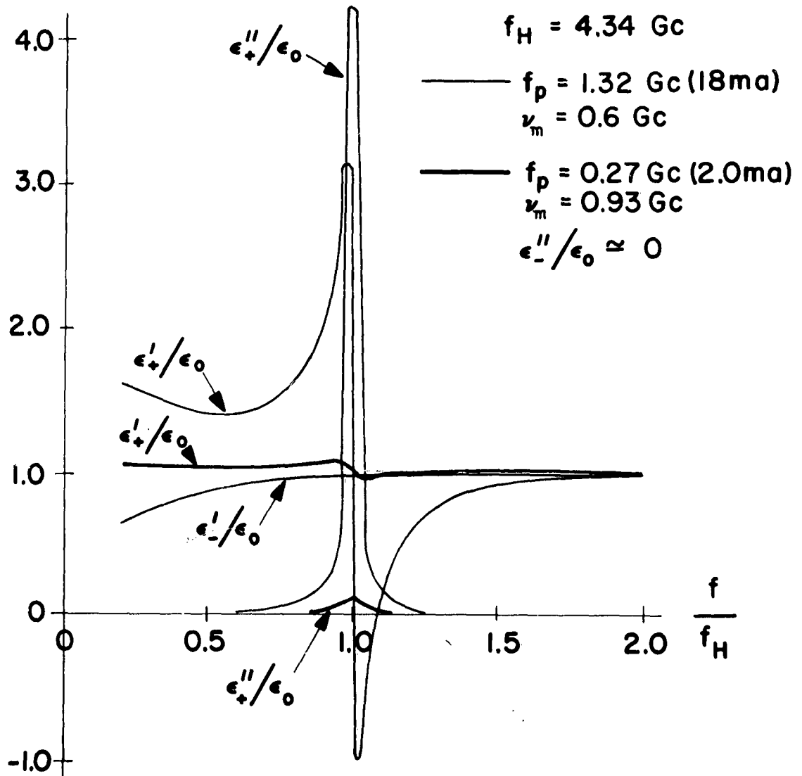
FIG. 3.17: RELATIVE PERMITTIVITY FOR ORDINARY AND EXTRAORDINARY WAVES AS A FUNCTION OF MICROWAVE FREQUENCY
