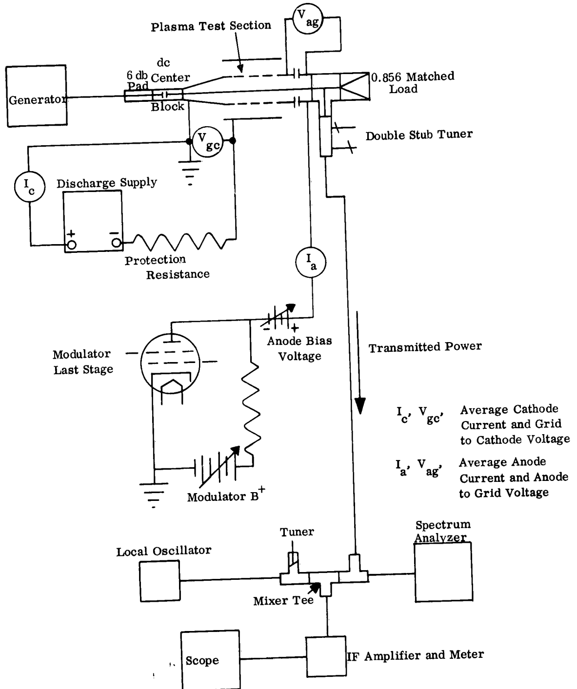
FIG. 2.12: CIRCUIT ARRANGEMENT
