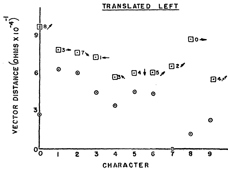
FIG. 41 RESULTS FOR HORIZONTAL CHARACTER TRANSLATION
