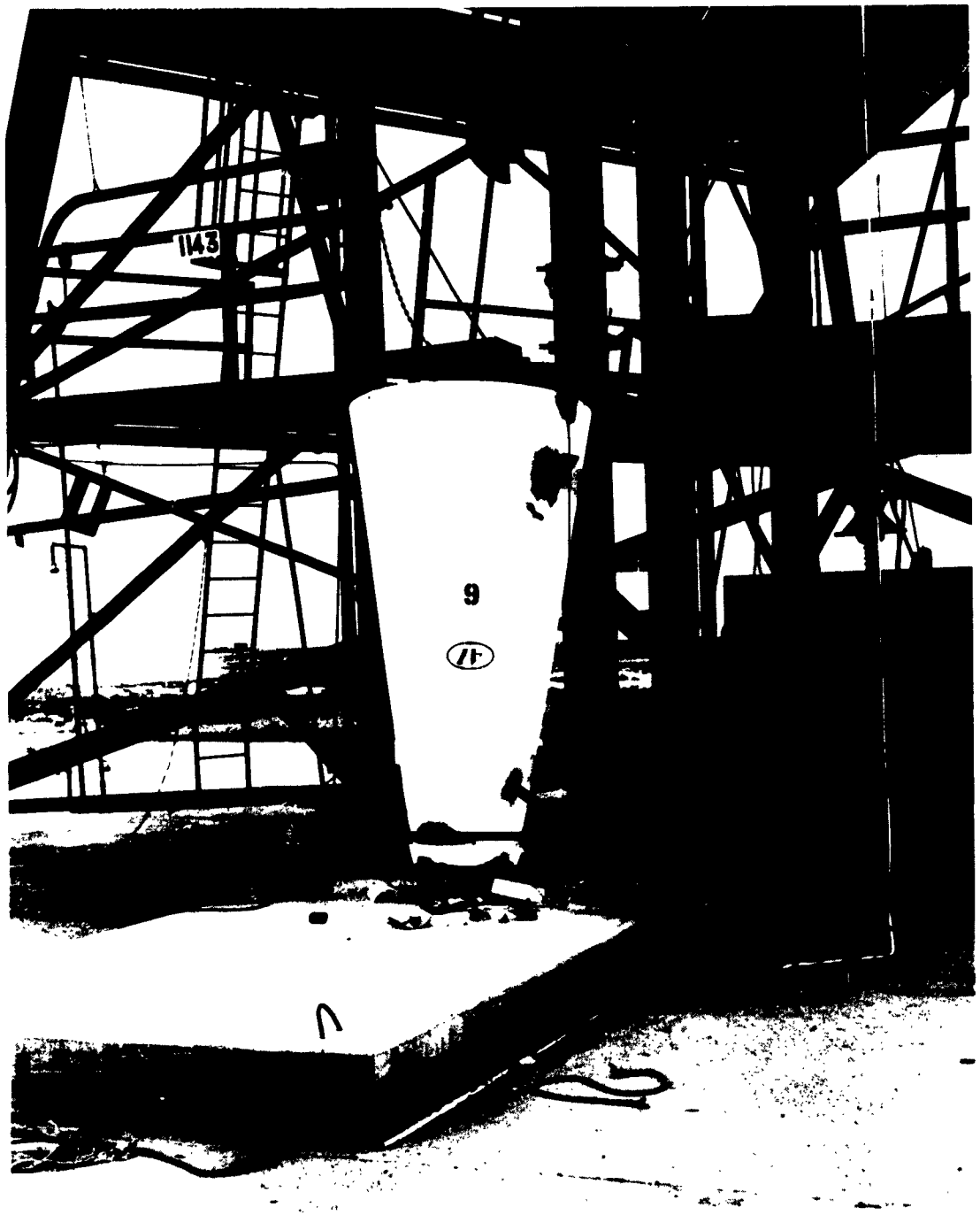
Figure 15. Reactor system -- post test
