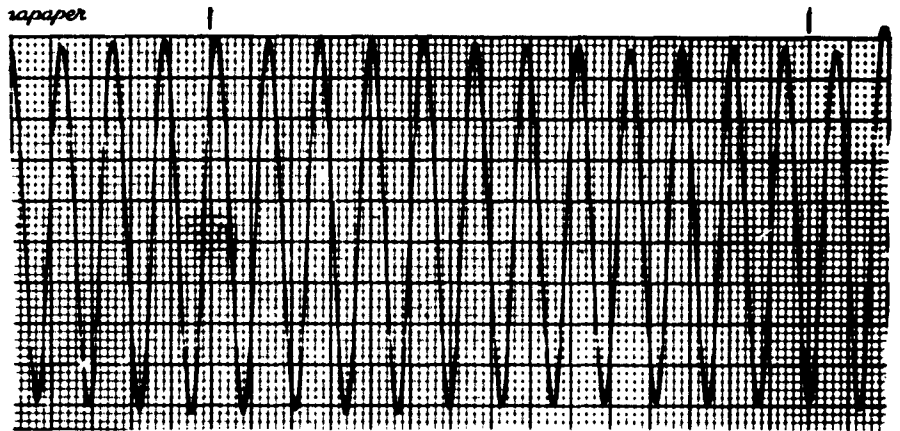
Fig. 3. — Output of the ferroelectric bolometer G-22, 2 mm \times 2 mm in size ; infrared signal approximately 7 \times 10^{-8} watt peak to peak, chopped at 3cps and a bandwidth \Delta f = 0.25 cps.
