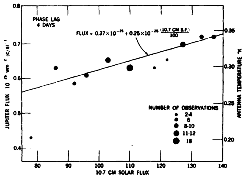
Fig. 3. — Least squares determination of the regression of Jupiter flux (at 1423 Mc) on solar activity. The Jupiter observational data were obtained with a maser radiometer attached to the Harvard 60-foot radio telescope.
