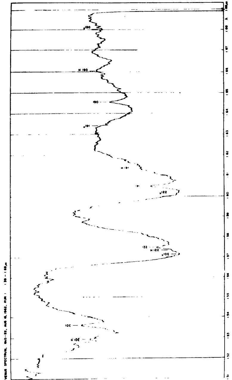
Fig. 7b. — Venus Spectrum, 1.39 — 1.69 \mu , Part 2.
