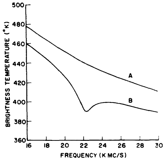
Fig. 5. — Theoretical microwave spectra of Venus computed assuming an atmosphere of CO_2 , N_2 , and H_2O , a surface temperature of 580^\circ K and a surface pressure of 30 atm. Curve A assumes an H_2O mixing ratio of 10^{-3} at the surface and decreasing linearly to zero at 33 km. Curve B assumes an H_2O mixing ratio of 10^{-3} to be uniform throughout the atmosphere.
