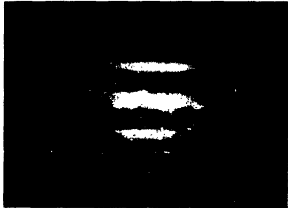
Fig. 3. Strips and blocks of dark matter emanating from dark nodes, moving polewards oppositely to the direction of rotation of the planet, spread along the axes of the cells and form the belts.
