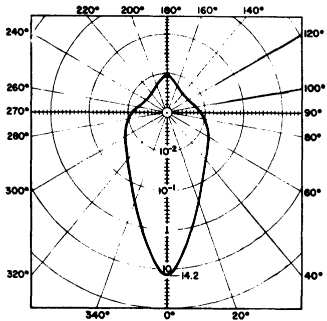
Fig. 5. — Phase function [\gamma(\cos \theta)] due to Deirmendjian
