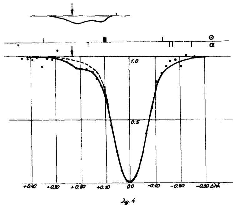
Figs. 2-4 show average profiles of the telluric lines 1, 2, 4-10 (in Fig. 2 and 3) and 1-4, 6-8 (Fig. 4).
