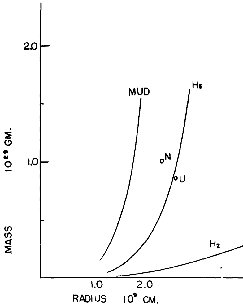
Fig. 1. — Theoretical mass-radius curves for planets composed of pure hydrogen, helium or mud. The small circles correspond to the empirical values for Uranus and Neptune
