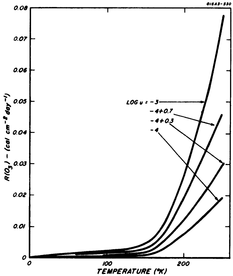
Fig. 3. — Extrapolated values of R(O_3) .
