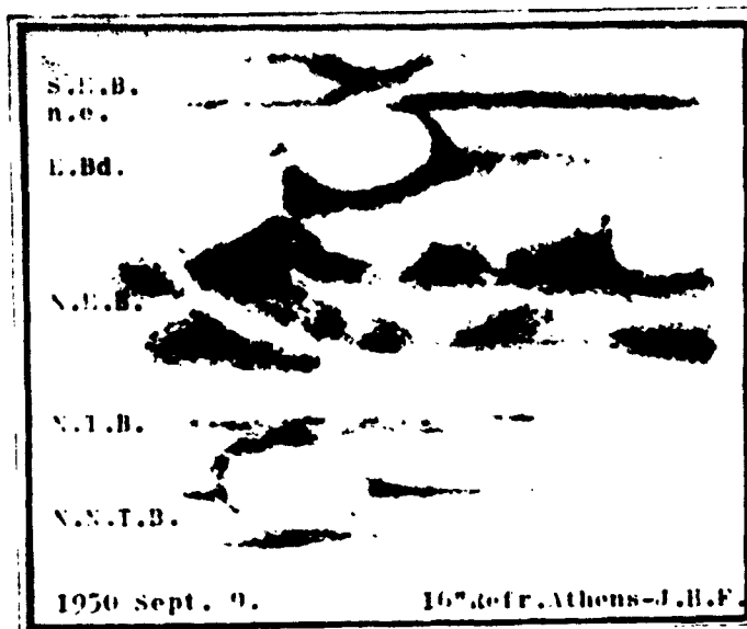
Fig. 5. Brilliant spots in ascending motion broke up the Equatorial Band and the N.N.T.B. Deviation of dark matter as a result of the action of such brilliant spots is obvious.
