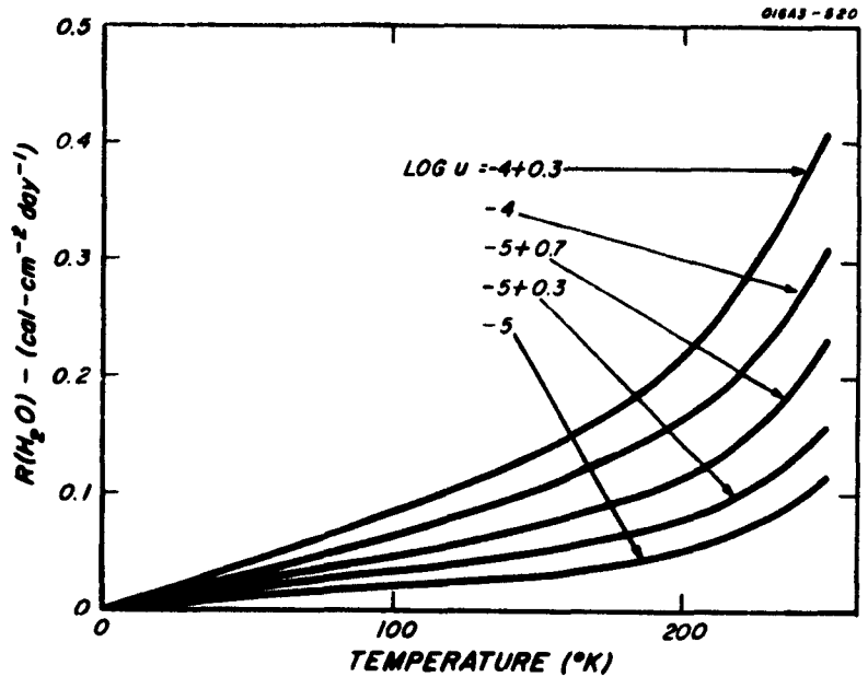
Fig. 2. -- Extrapolated values of R(H_2O) .
