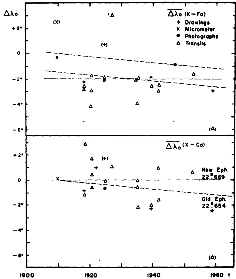
Fig. 8. — Mean longitude differences from provisional mean Fournier system (above) and mean Camichel system (below), all reduced to new ephemeris system, and corrected for phase effects (where applicable).
