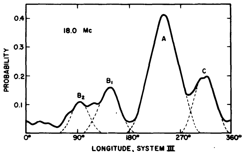
Fig. 1. — Smoothed probability profile for Jovian sources at 18 Mc/s. The longitude system used is the radiofrequency System III (Carr et al 1961).
