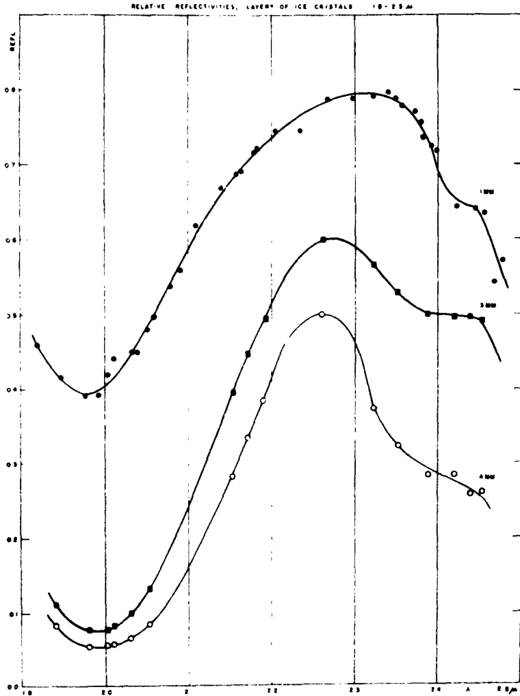
Fig. 4b. -- Reflectivities of layers of ice crystals 1 mm, 3 mm, and 4 mm thick, derived from Figure 4a. The shapes of the curves are fixed by the ratios measured from Figure 4a; the scales of the ordinates cannot be found from the measures and have been chosen somewhat arbitrarily.
