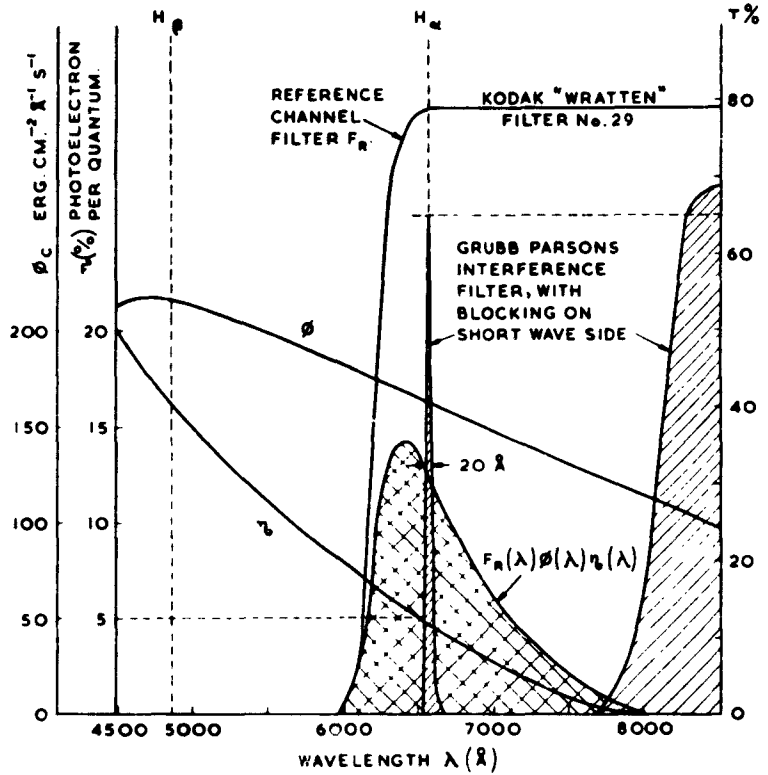
Fig. 2. — Spectral Distributions and Response Curves.
