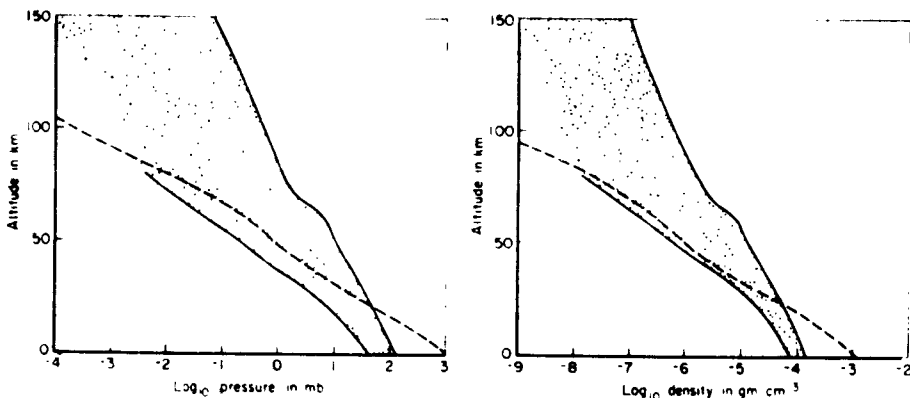
Variations of pressure and density extremes with altitude (Earth ARDC 1959 Model Atmosphere shown as dashed line)
