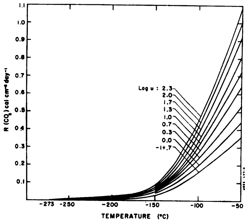
Fig. 1. — Extrapolated values of R(\text{CO}_2) .
