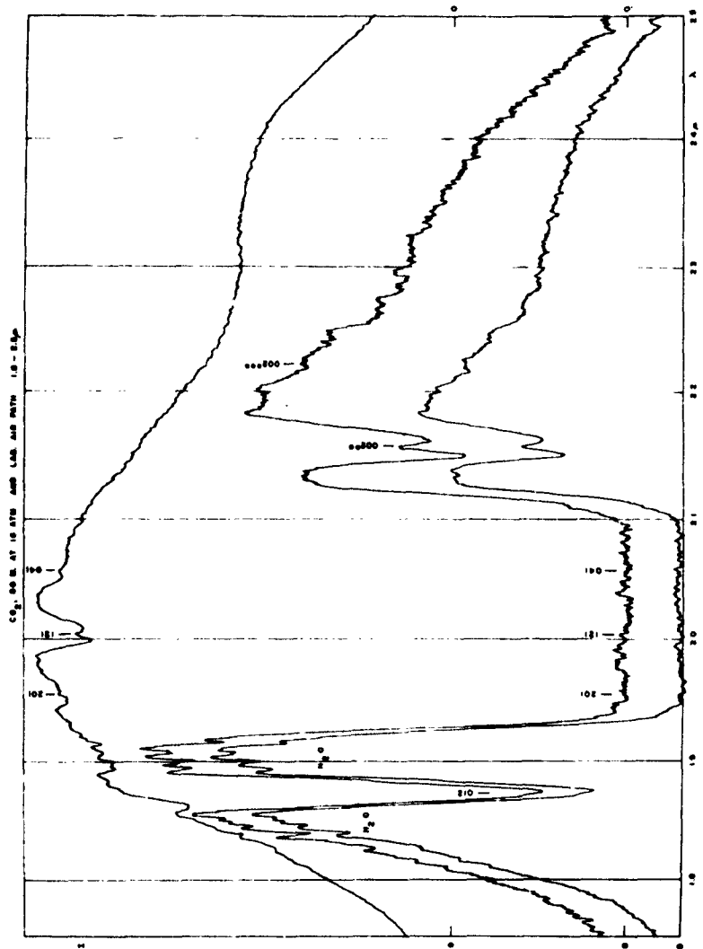
Fig. 11.— \text{CO}_2 Spectrum, 80 meter path at 16 atm., 1.8 — 2.5 \mu , Grating 2 \mu , filter \lambda > 1.8 \mu , cell 0.25 mm, slit 0.28 mm, \tau = 6 seconds. The \text{H}_2\text{O} and \text{CO}_2 absorptions contributed by the 4\frac{1}{2} meter air path in the laboratory and the spectrometer is shown in the upper curve. The zero intensity levels are indicated in the margins.
