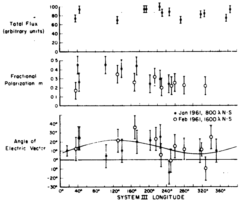
Fig. 3. — Polarization of the 960 mc/s radiation from Jupiter. Fractional polarization, and position angle of the electric vector measured relative to Jupiter's equator, as a function of the System III longitude of the central meridian.
