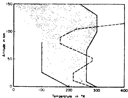
Variations of temperature extremes with altitude
