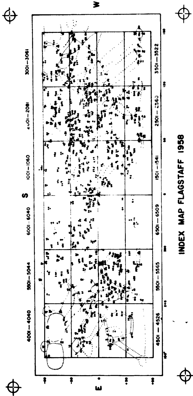
Fig. 5. — Index map of Flagstaff observations, 1958 (546 points).
