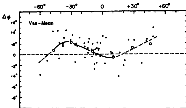
Fig. 10. — Example of systematic latitude differences vs. longitude.
