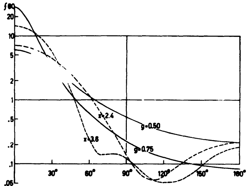
Fig. 3. — Dashed curves : Total intensity scattering diagram for droplets with m = 1.33 and two values of the size parameter x = 2\pi a/\lambda . Solid curves : Henyey-Greenstein phase function for g = 0.5 and 0.75 .
