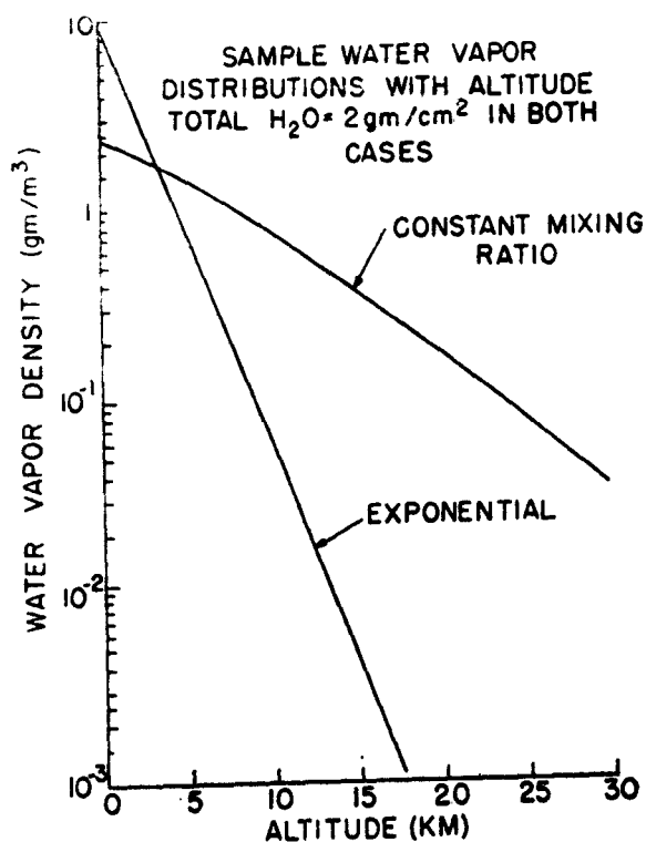
Fig. 1. — Sample vertical distributions of H 2 O.
