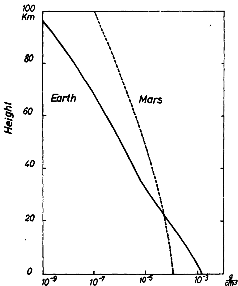
Fig. 2. — Air density profiles
