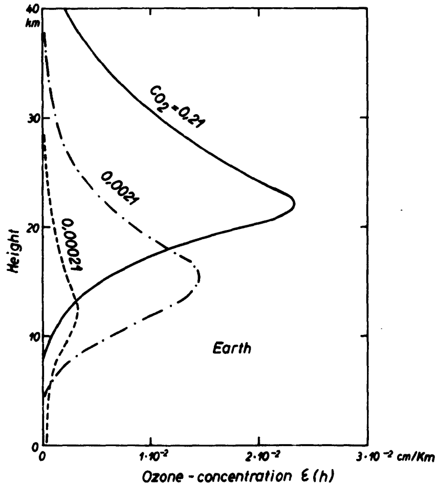
Fig. 3. — Vertical ozone profiles on Earth
