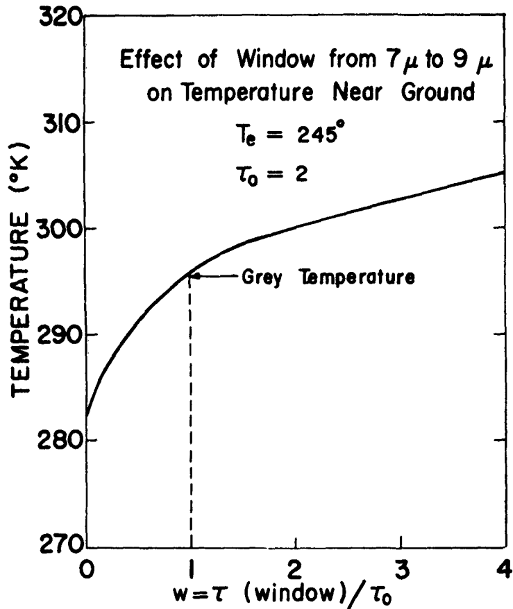
Fig. 5. — Similar to Figure 4 except that T_e and \tau_0 are chosen to approximate conditions for the earth. The relative optical depth was permitted to go above one, making the « window » an « absorption band ».
