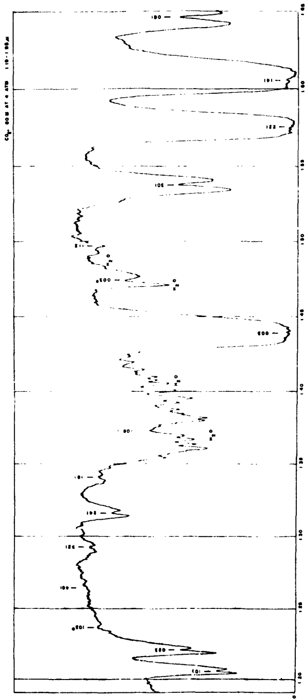
Fig. 9. — CO 2 Spectrum, 80 meter path at 4 atm., 1.10—1.95 μ, grating 1.6 μ, filter 2540, cell 0.25, slit 0.3 mm, τ=6 seconds. The CO 2 is contaminated with water vapor. The zero level 1.85 — 1.95 μ is raised by second-order 0.92 — 0.97 μ passing the 2540 filter.
