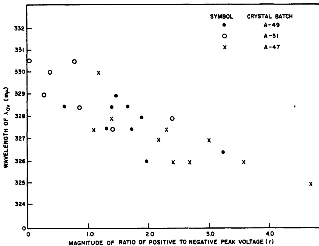
Fig. 14 Relation Between \lambda_{OV} and r
