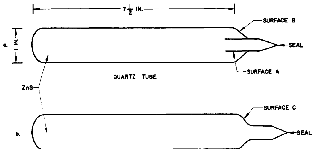
Fig. 2 Crystal Growing Tubes
