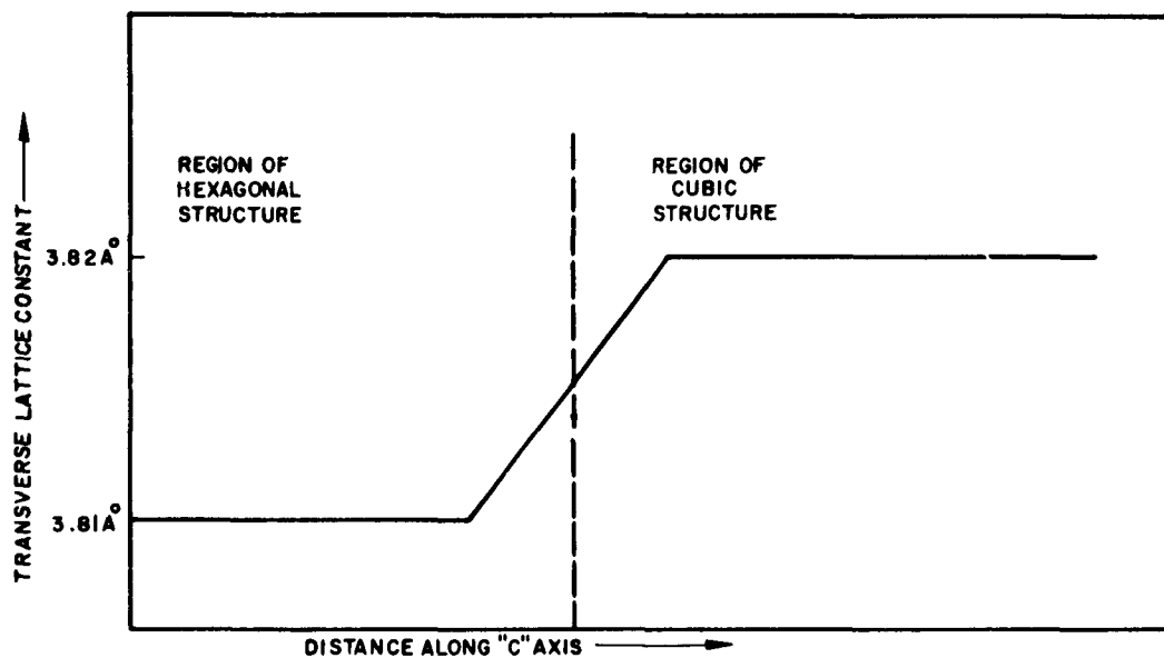
Fig. 7 Variation of Lattice Constant in Vicinity of Structure Change
