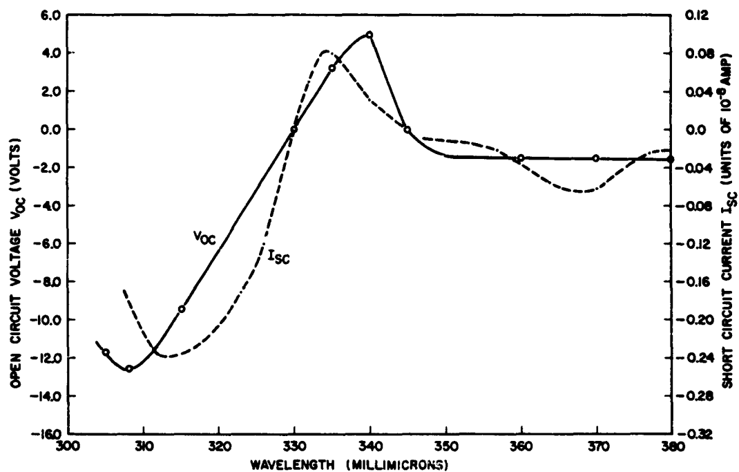
Fig. 1 Spectral Dependence of Anomalous Photovoltaic Effect
