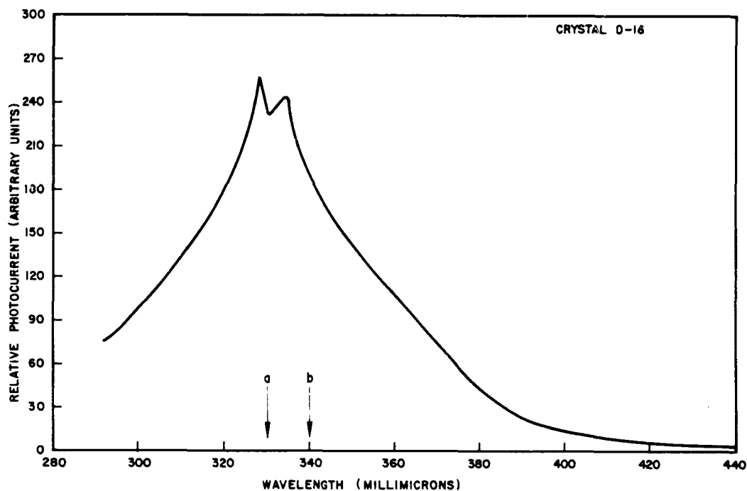
Fig. 10a Photoconductivity in a Mixed ZnS Crystal
