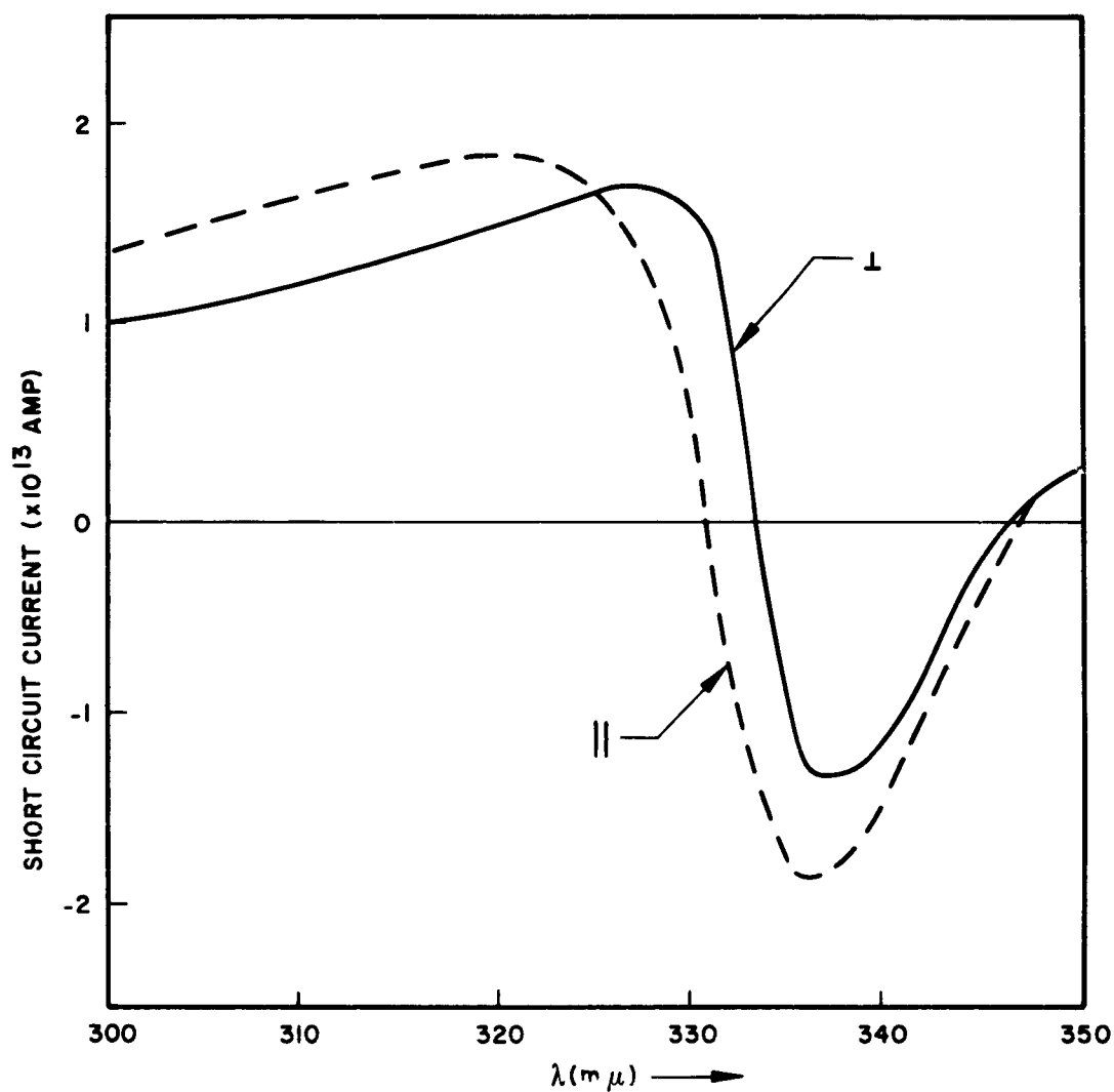
Fig. 11b Effect of Polarized Light on Photovoltaic Current
