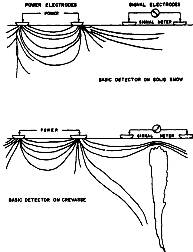
Figure 38. Schematic illustration of the way a "dishpan" electrical crevasse detector works. (After Cook, ref. 5; and U. S. Army TRAG, ref. 28)
