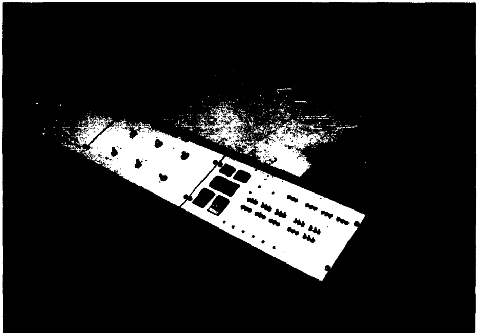
Figure 1.3. Plotter used with Sketchpad. A digital and analog control system makes the plotter draw straight lines and circles either under direct control of the TX-2 or off-line from punched paper tape.
