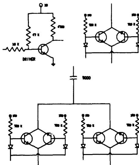
FIGURE 9.11. CIRCUIT DIAGRAMS
