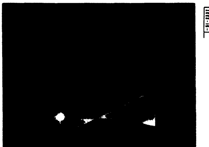
Figure 9.3. Three-bar linkage. The paths of four points on the central link are traced. This is a 15-second time exposure of a moving Sketchpad drawing.
