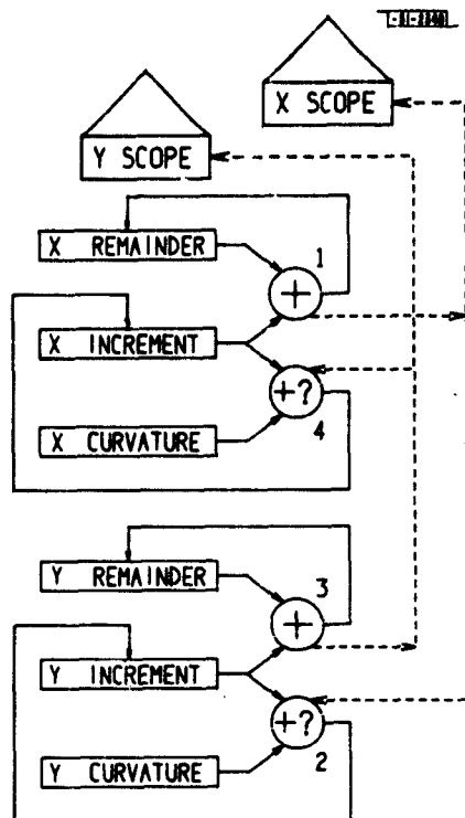
FIGURE E.2. DDA FOR UPRIGHT CONICS
