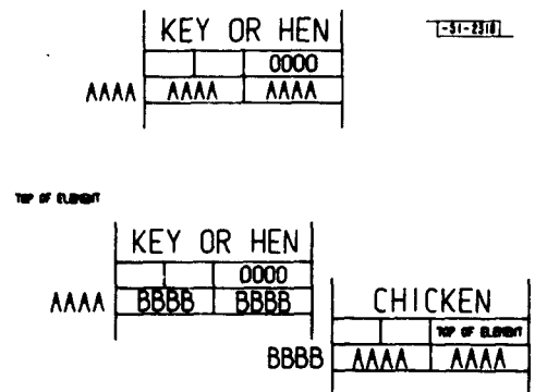
FIGURE 3.4. ZERO AND ONE MEMBER RINGS
