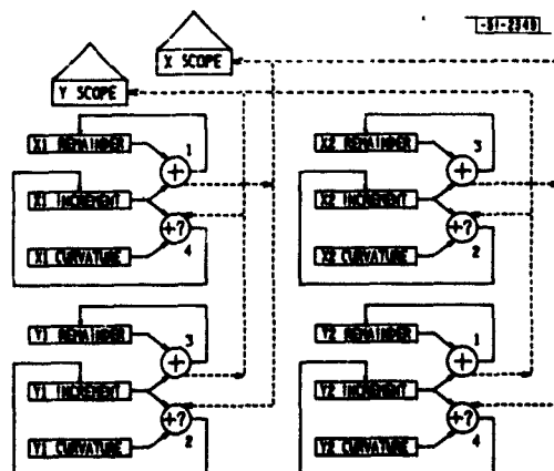
FIGURE E.3. DDA FOR THE GENERAL CONIC
