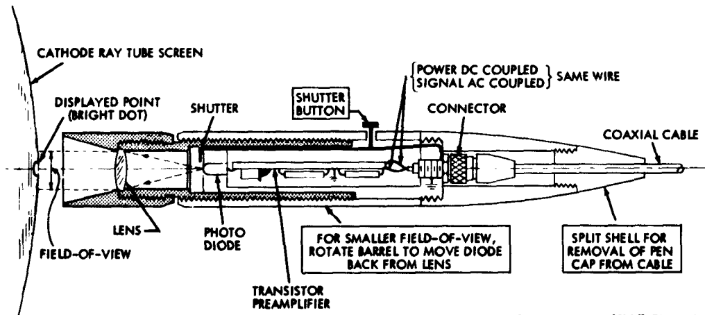
Figure 4.2. Construction of light pen. This drawing was made by conventional methods.
