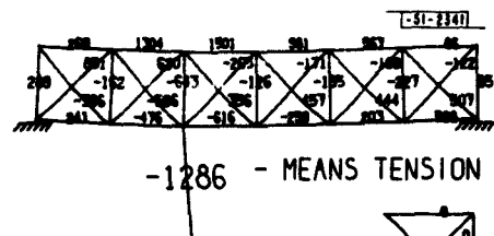
FIGURE 9.6. TRUSS UNDER LOAD
