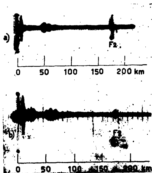
Fig. 4 - Echoes observed about noon (December, 1960) in the station A, when the pulses were emitted from Torrecchiarruccia, on 4.1 Mc/s. The record a was taken with a calm sea; the record b, with a rough sea, the receiver sensitivity being 12 dB lower than for record a. The distance scale gives the difference between echo and direct pulse paths, divided by 2. The first echo, corresponding to an equivalent distance of 10 Km, is due to Giglio's island.
