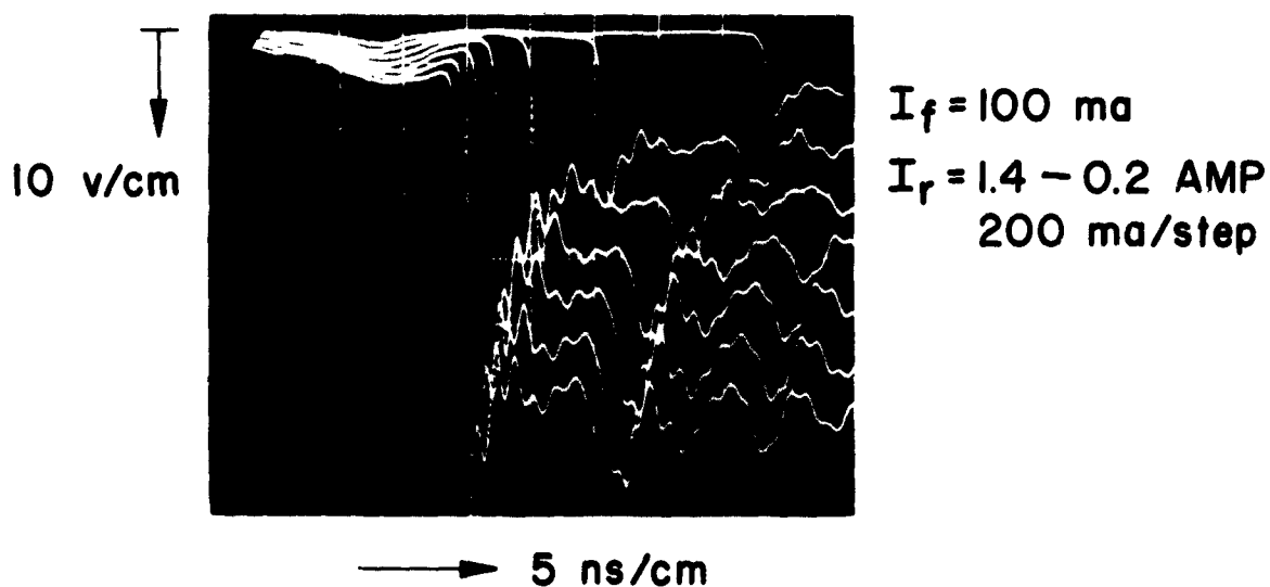
Fig. 10. Small-area diode storage and transition times
