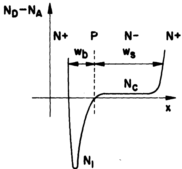
Fig. 4. Doping profile
