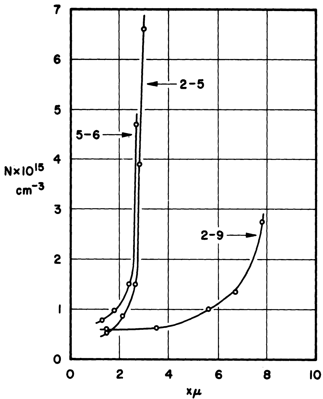
Fig. 7. N^- region doping density vs. distance
