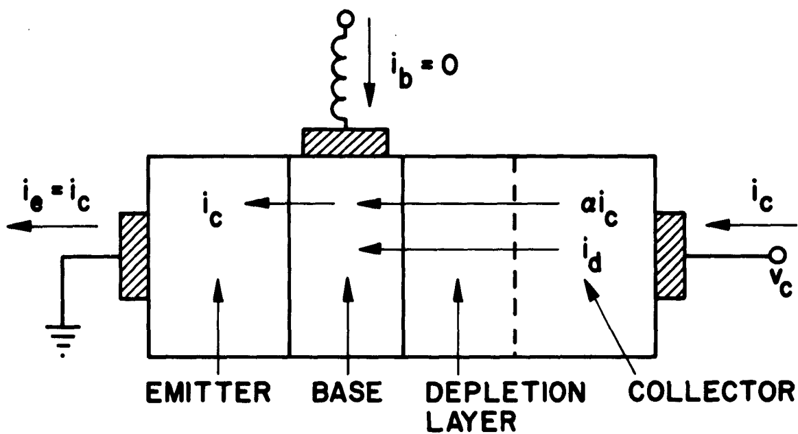
Fig. 1. Basic transit-time diode
