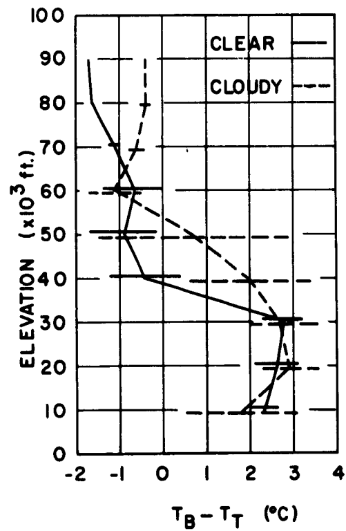
FIGURE 20 DIFFERENCE BETWEEN TEMPERATURE INSIDE BALLOON AT BOTTOM ( T_B ) AND TOP ( T_T ) FOR NIGHT-TIME CLEAR AND CLOUDY CONDITIONS (Horizontal lines represent \pm one standard deviation)
