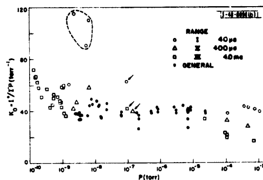
(b) The open Nottingham gauge, N2.
