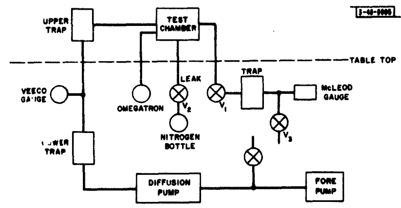
Fig. 3. Layout of vacuum system.
