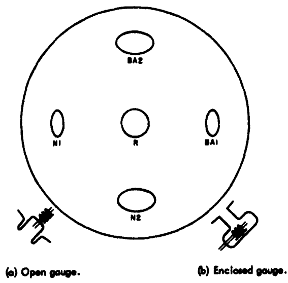
Fig. 2. Arrangement of the gauges.
