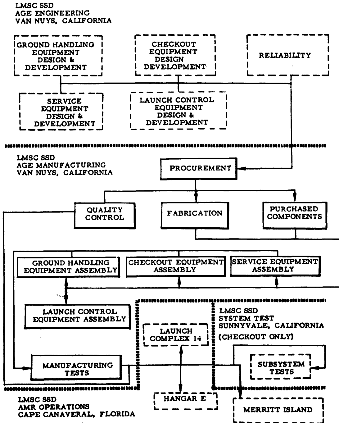
Figure 8-3 AGE Manufacturing
