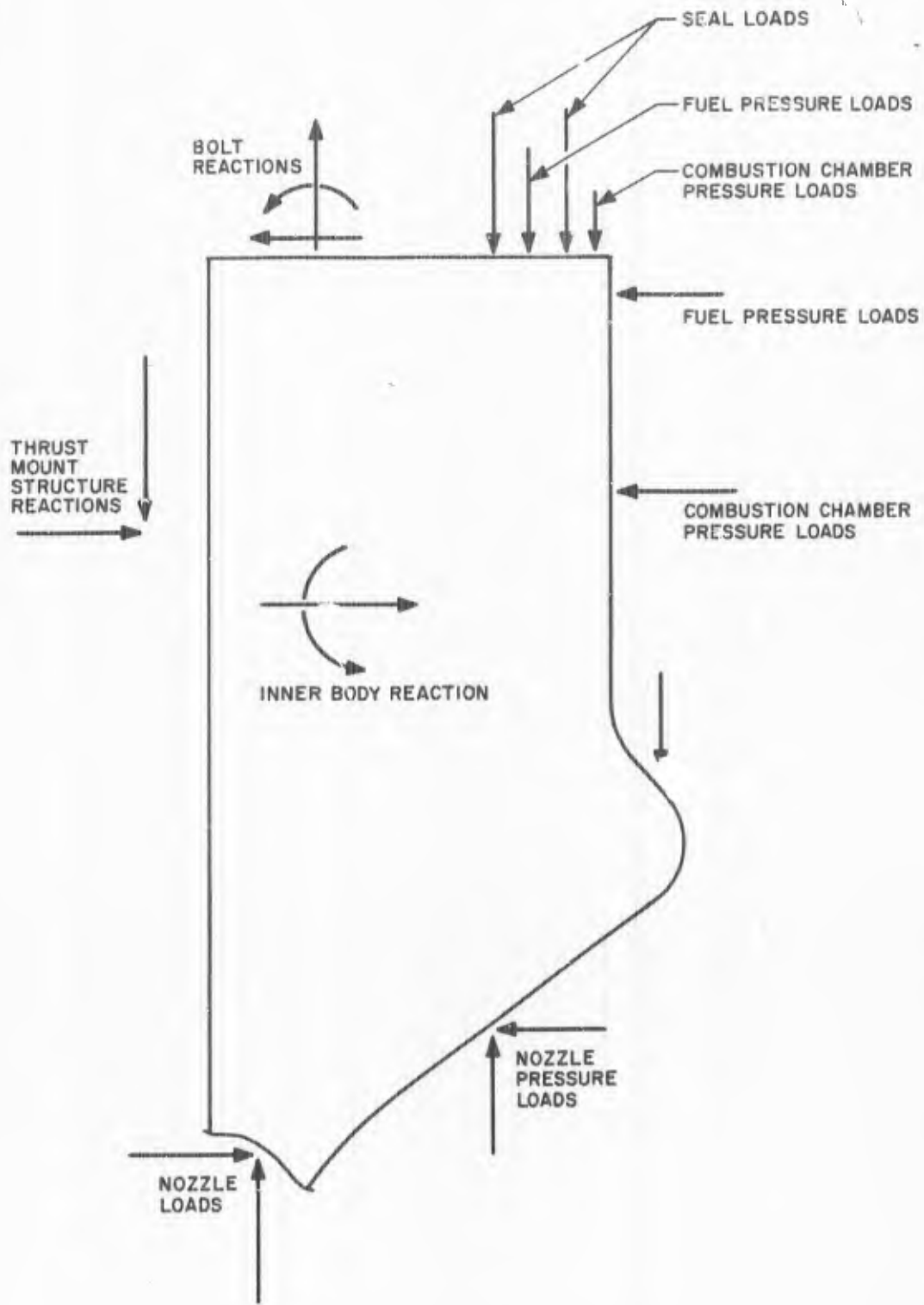
Figure 25. Forces Acting on Inner Body
