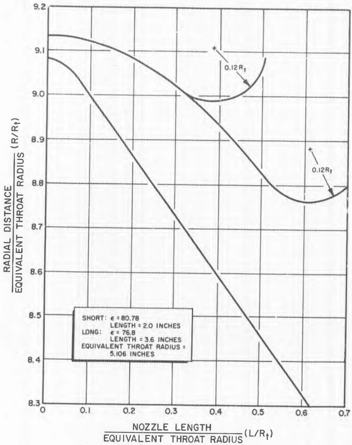
Figure 30. ADP Shroud Length Comparison
