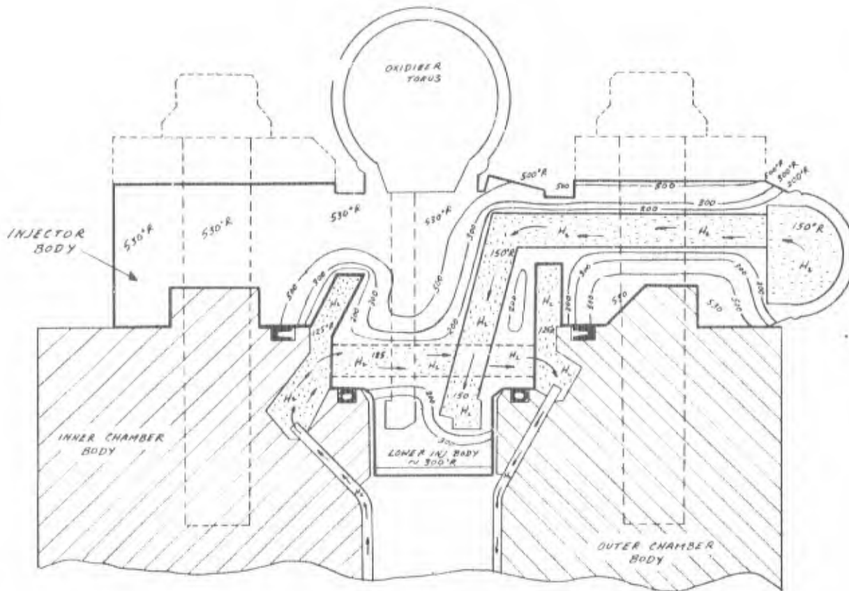
Figure 4/4. Approximate Injector Body Isotherm Distribution After a 5-Second Hydrogen Chillover
