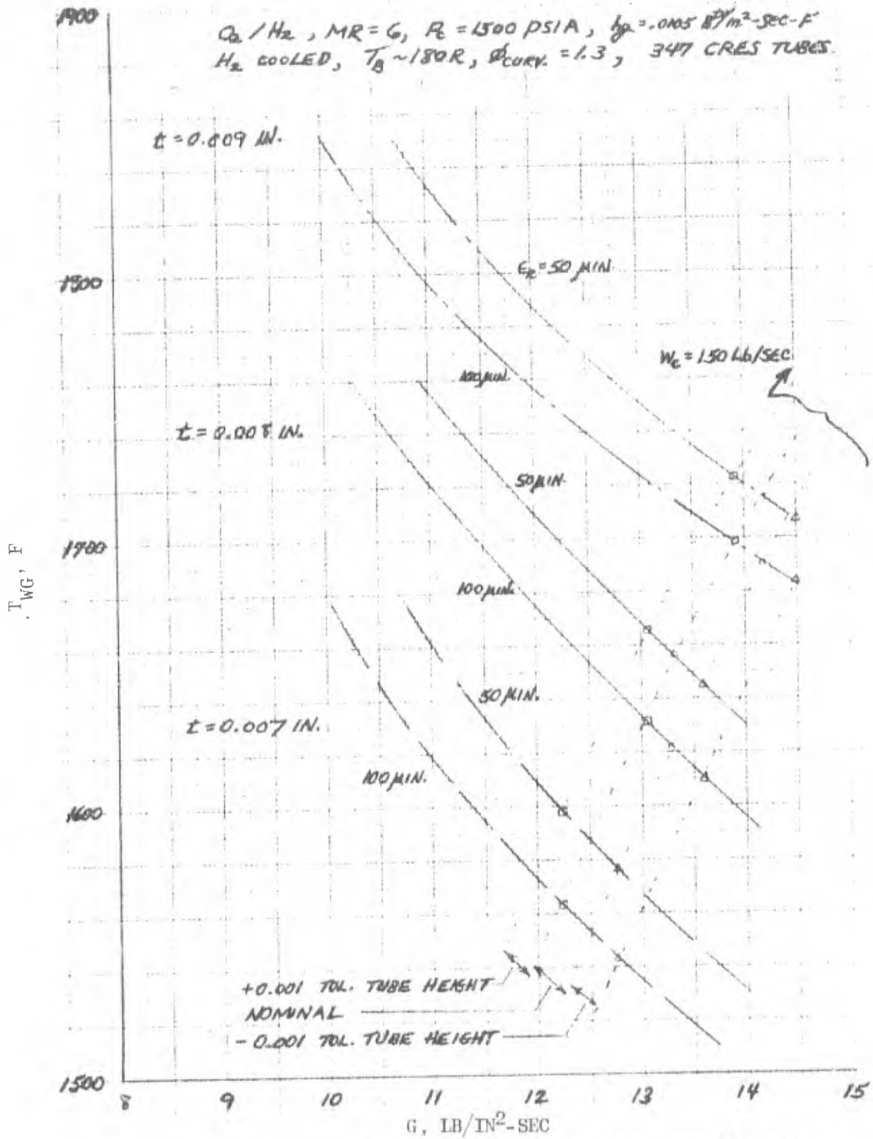
Figure 43. Effect of Tube Tolerances and Coolant Mass Velocity on Gas Wall Temperature
