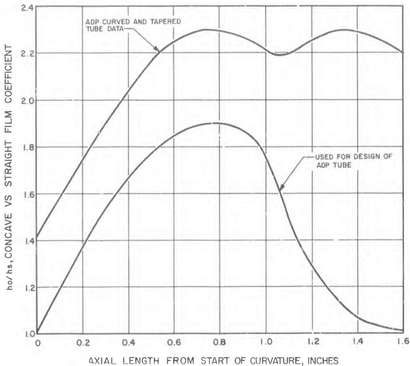
Figure 42. Comparison of Film Coefficient Enhancement Factor used for ADP Design with ADP Tube Experimental Results
