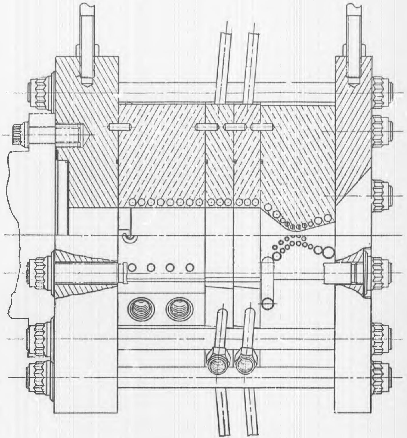
Figure 18. 2.5K Solid-Wall Thrust Chamber
