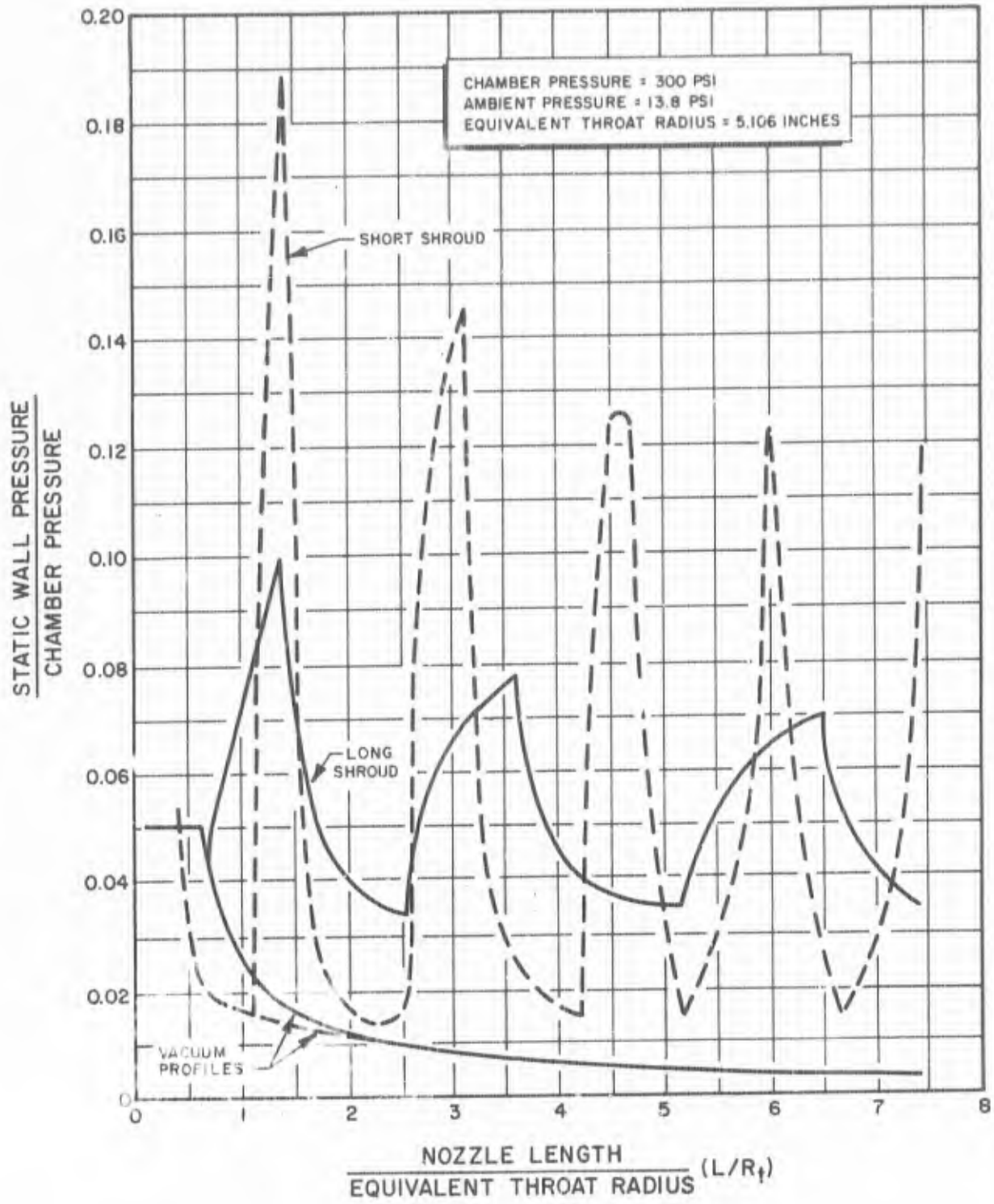
Figure 34. ADP Sea Level Centerbody Spike Wall Pressure Profiles
