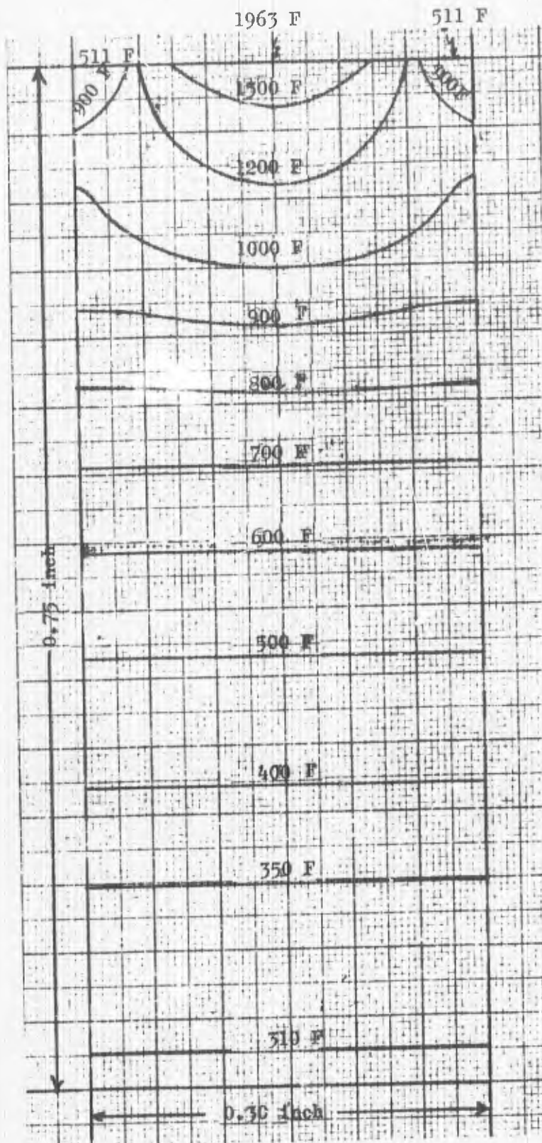
Figure 23. Wall Temperature Distribution in Throat of ADP Water Film-Cooled, Solid-Wall Chamber After 0.72 Second
