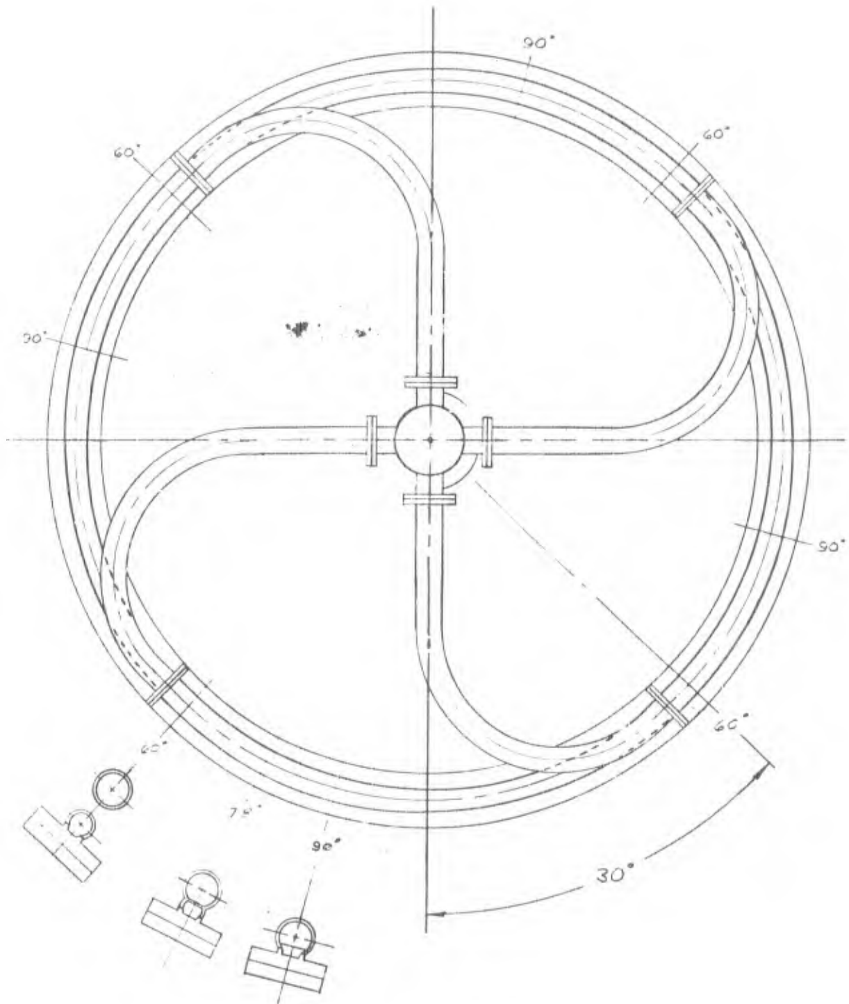
Figure 46. Oxidizer Manifold Cold Flow
