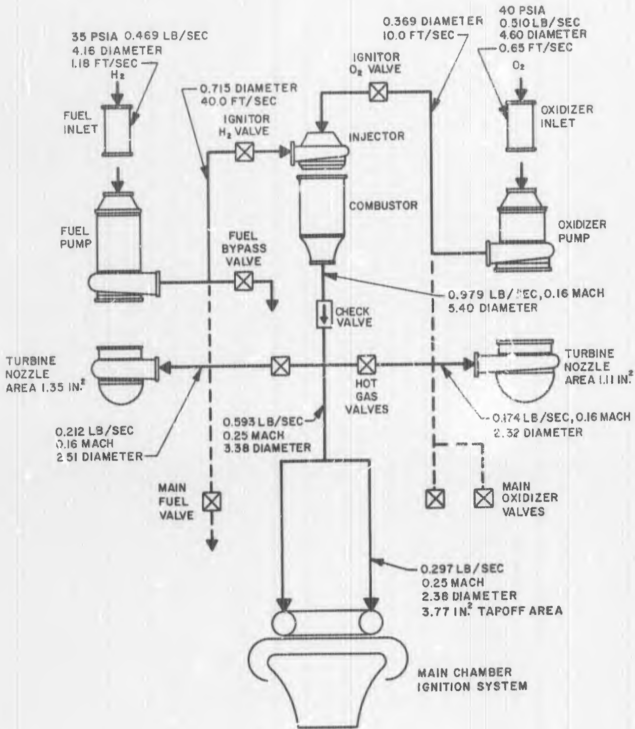
Figure 17. Igniter Hot-Gas Subsystem
