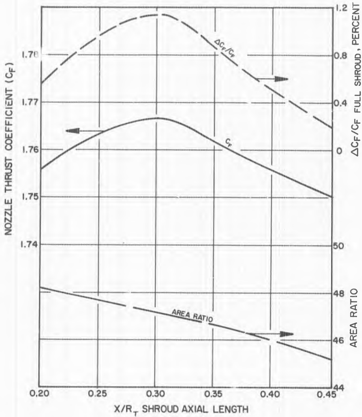
Figure 31. Performance vs Shroud Length
