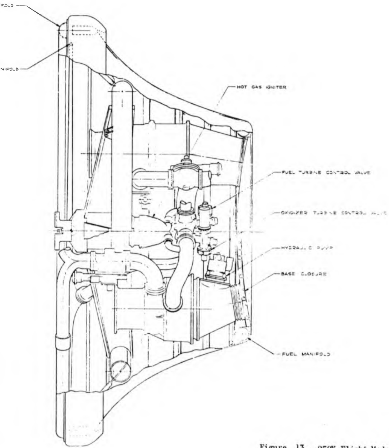
Figure 13. 250K Flight Module (100 inch diameter)
