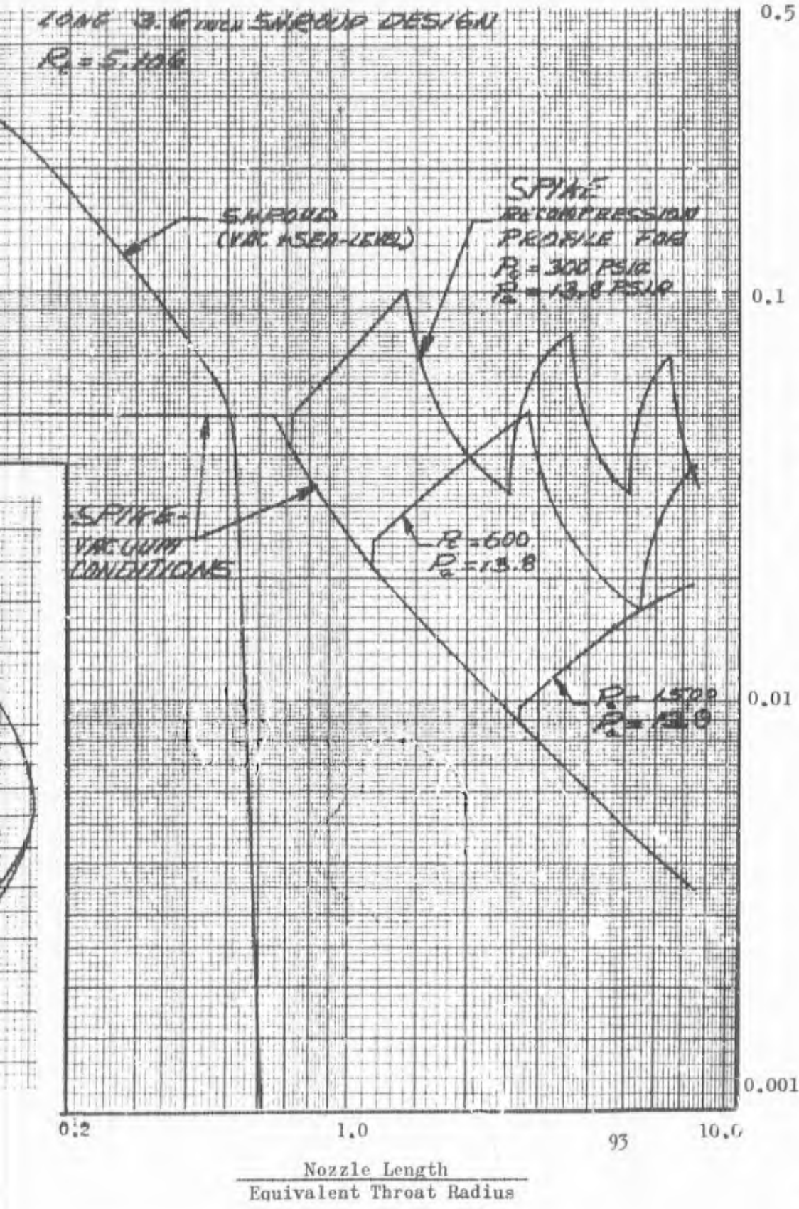
Figure 32. Shroud and Spike Pressure Profiles
