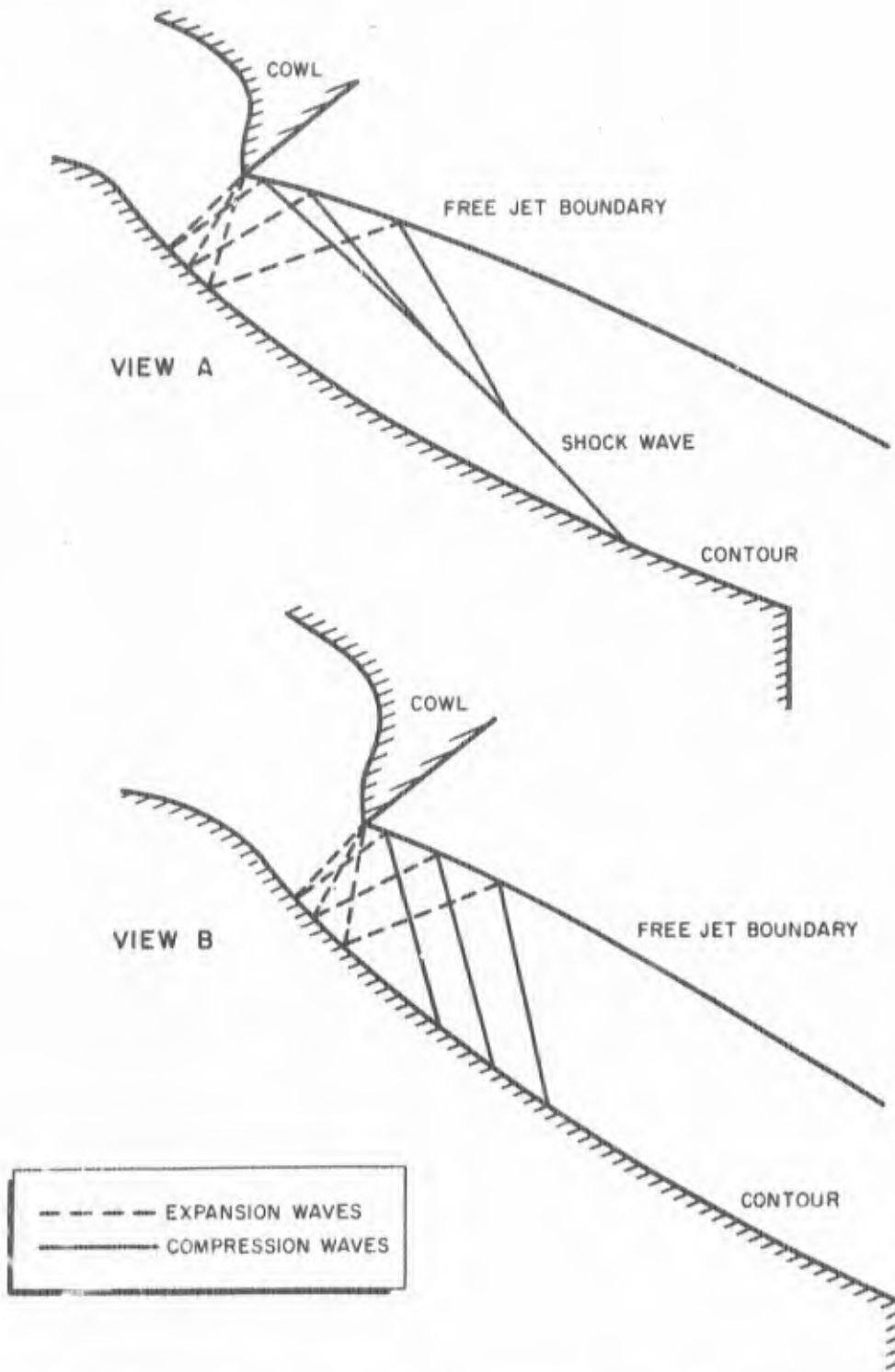
Figure 35. Expansion and Compression Waves in Aerodynamic Spike Nozzle Flow Field Analysis
