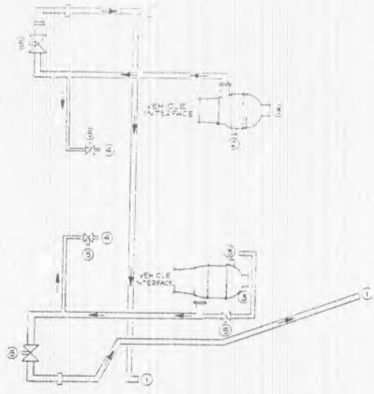
② - PROPELLANT FEED SUBSYSTEM
