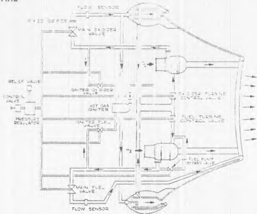
DEMONSTRATOR MODULE SYSTEM SCHEMATIC
