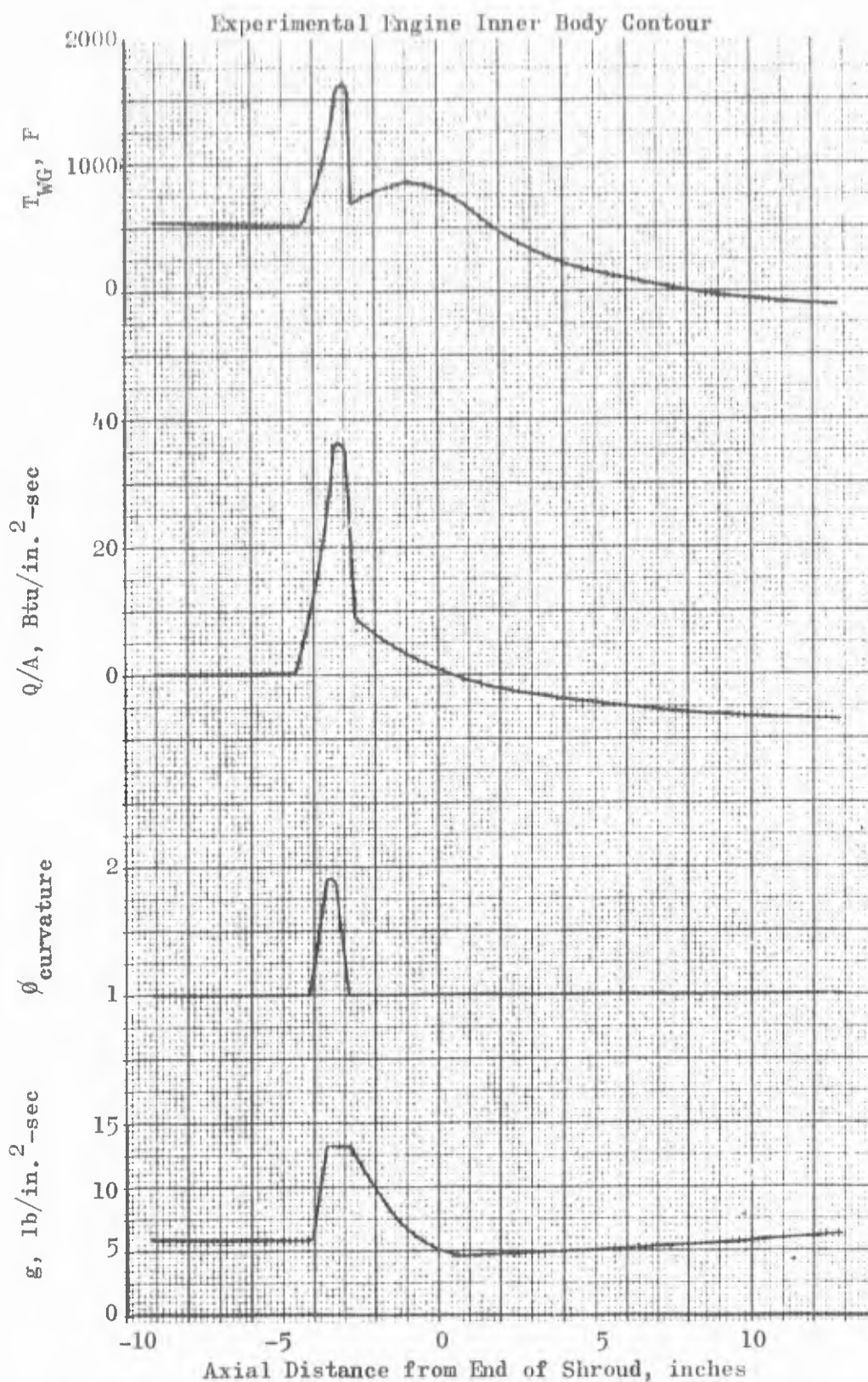
Figure 37. Gas-Side Wall Temperature, Heat Flux, Curvature Enhancement, and Coolant Mass Velocity Profiles, ( O_2/H_2 , P_c = 1500 psia, MR = 6.0 , W_c = 150 lb/sec)
