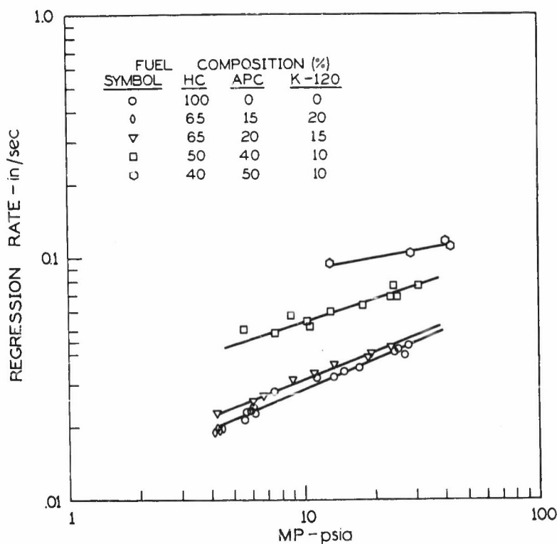
Fig. 4 Effect of ammonium perchlorate content on regression rate of hybrid fuels.
