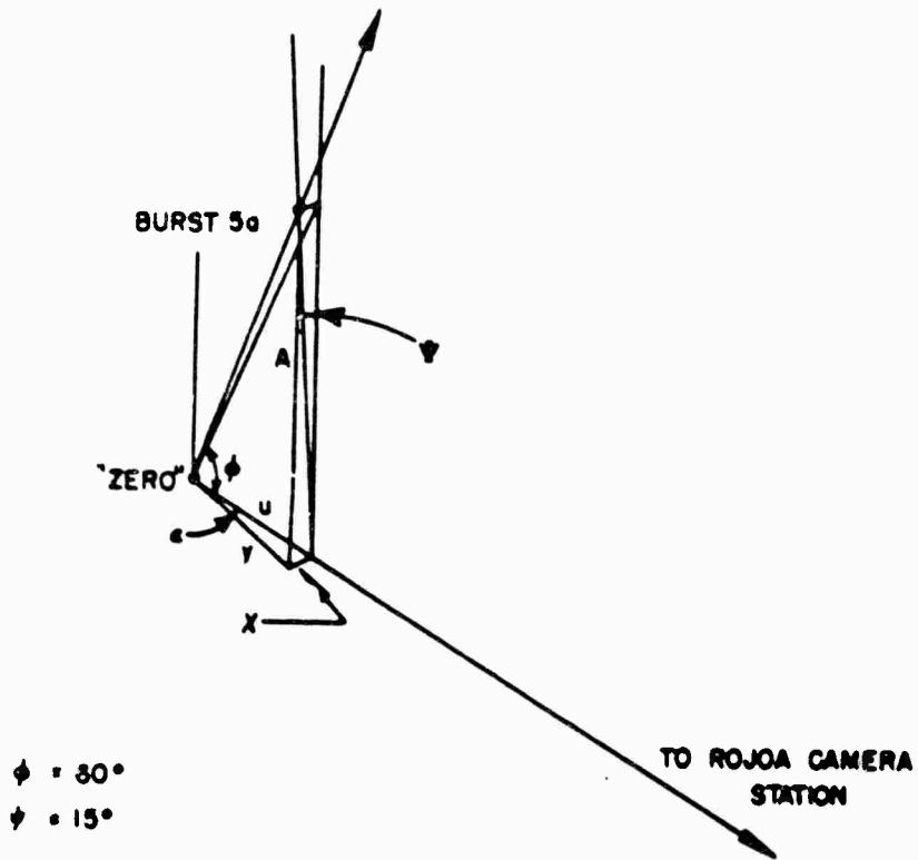
Fig. 8.1—Position of gun burst 5a.
