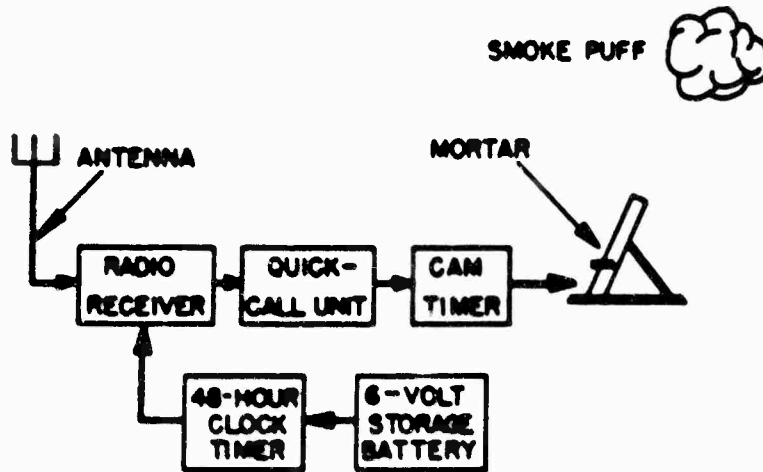
Fig. 24—Ball radio firing system (EG&G photograph).
