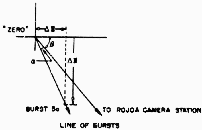
Fig. P 9—"Zero" and burst 5a in plan.
