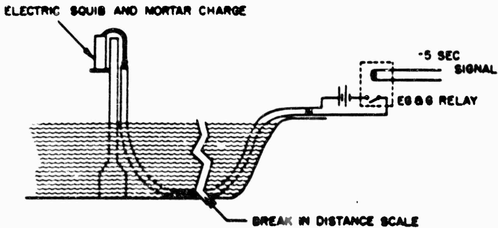
Fig. 2.2 — Reef mortar firing system.
