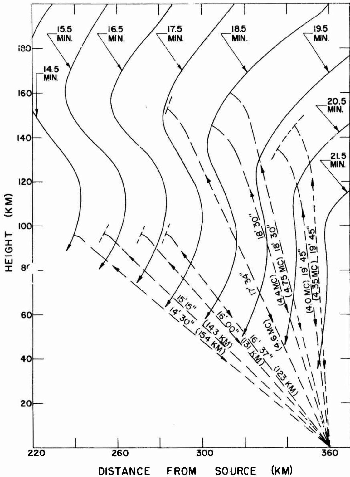
Fig. 3.7—Reflection, at the theoretical sonic-wave front in the E and F 1 regions, of oblique radio rays emanating from the ionosphere recorder, King day. (The short dashed lines represent the front at times from H hour corresponding to the plotted radio rays.)
