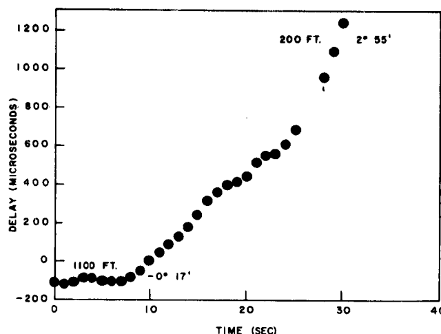
Fig. 6 - Plot of observed delay vs time for run with Mk 37 torpedo
