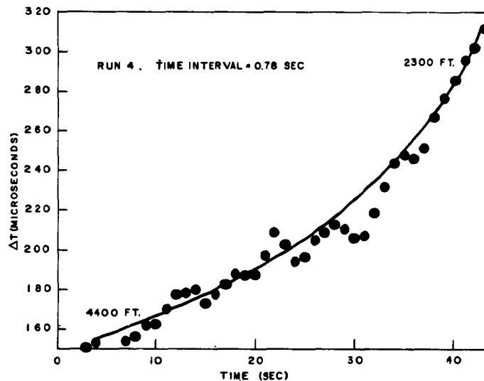
Fig. 5 - Plot of observed values of \Delta T vs time, showing effects believed to be caused by multipath interference
