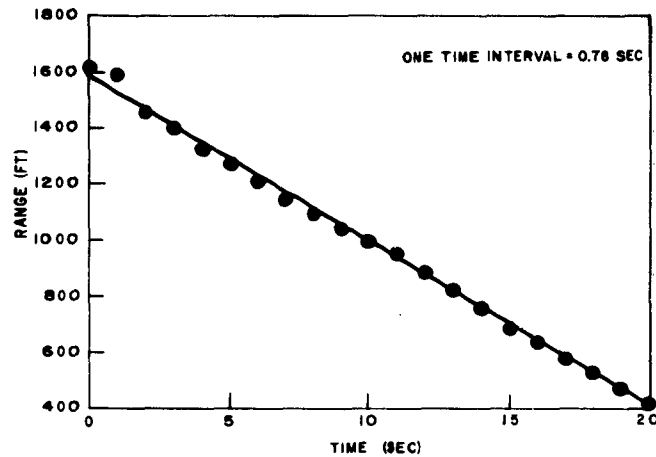
Fig. 4 - Plot of range (in feet) vs time for run 3
