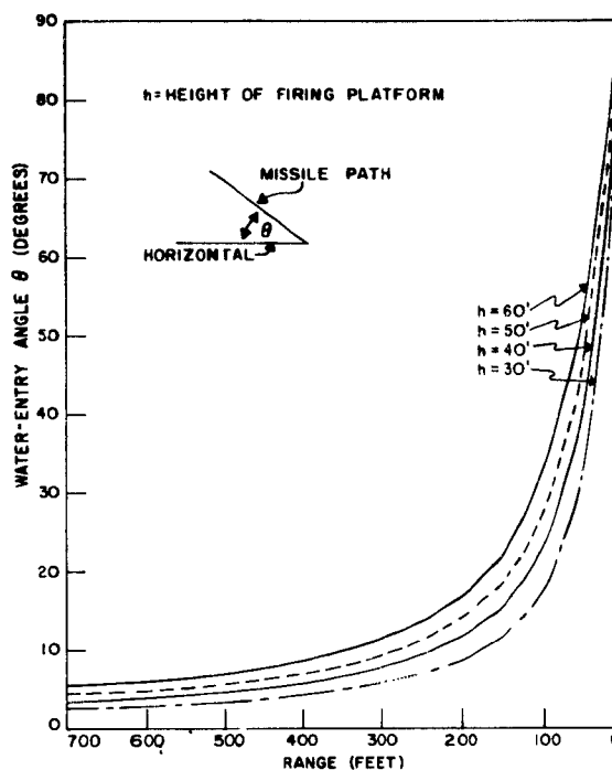
Fig. 7 - Water-entry angle vs range and height of firing platform
