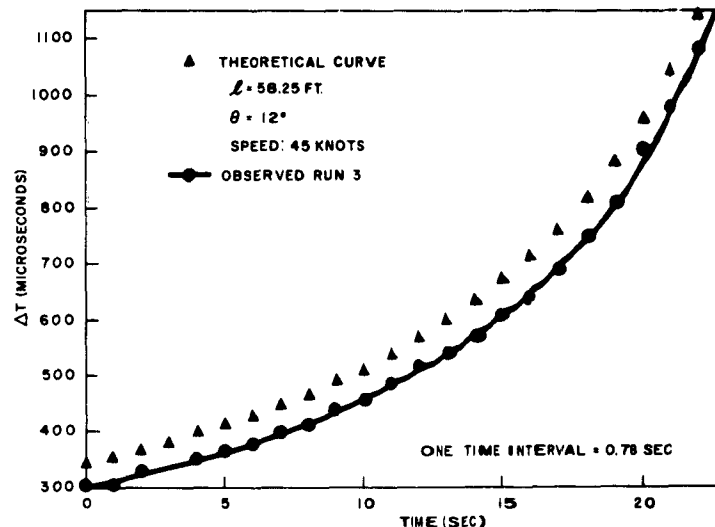
Fig. 3 - Comparison between computed and observed values of \Delta T vs time for run 3
