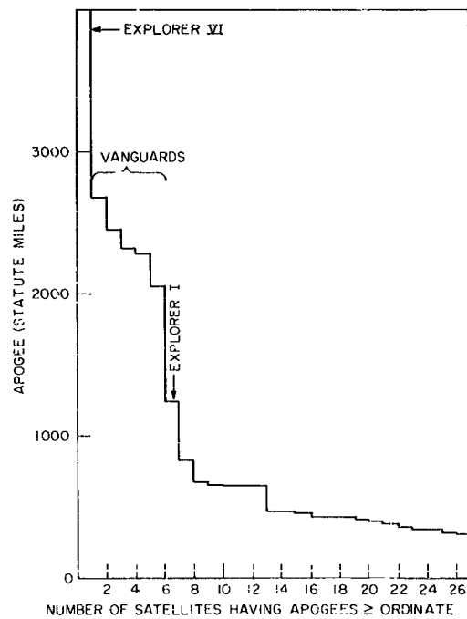
Fig. 13 - Distribution of apogee heights for satellites as of September 1960
