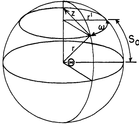
Figure 3. Diagram for Gore Width of Sphere
