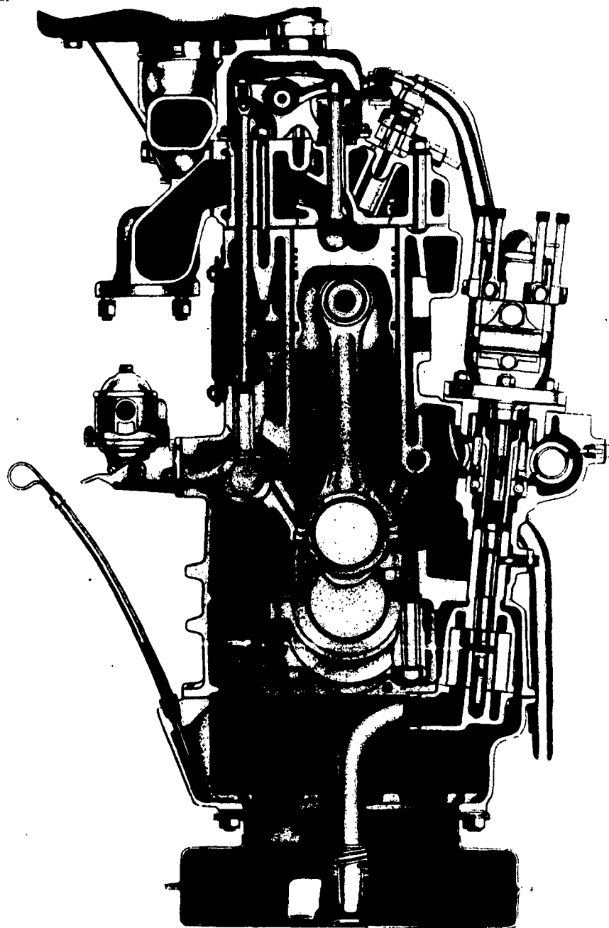
CROSS SECTIONAL VIEW PERKINS SIX '354' ENGINE.
