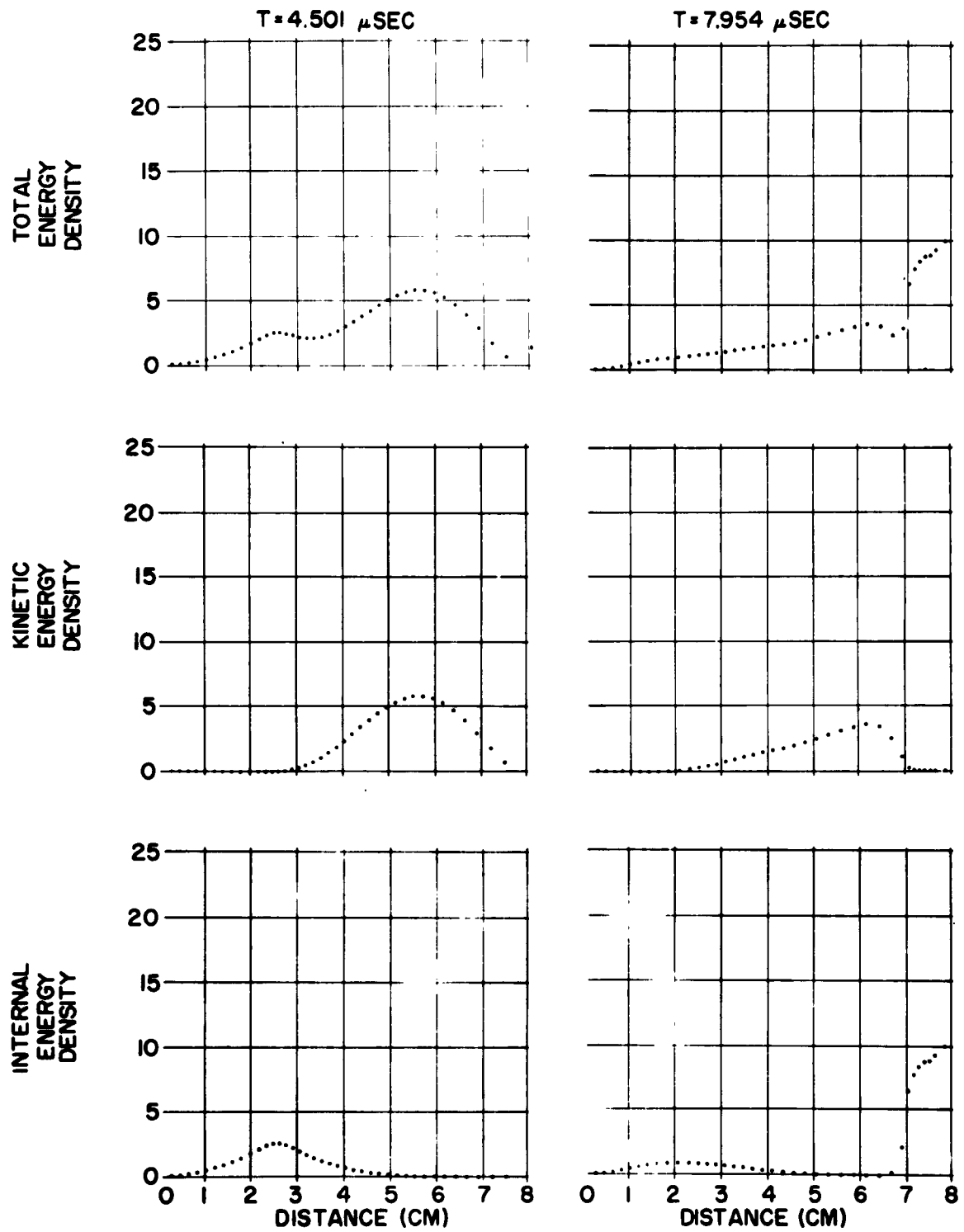
FIG. 10 ENERGY DENSITY (ENERGY / VOLUME \times 4\pi R^2 , IN UNITS OF MEGABAR - CM 2 ). WALL AT 8.0 CM, GAMMA = 2.682. AREA UNDER CURVE EQUALS ENERGY IN UNITS OF MEGABAR - CM 3 . 1-LB PENTOLITE
