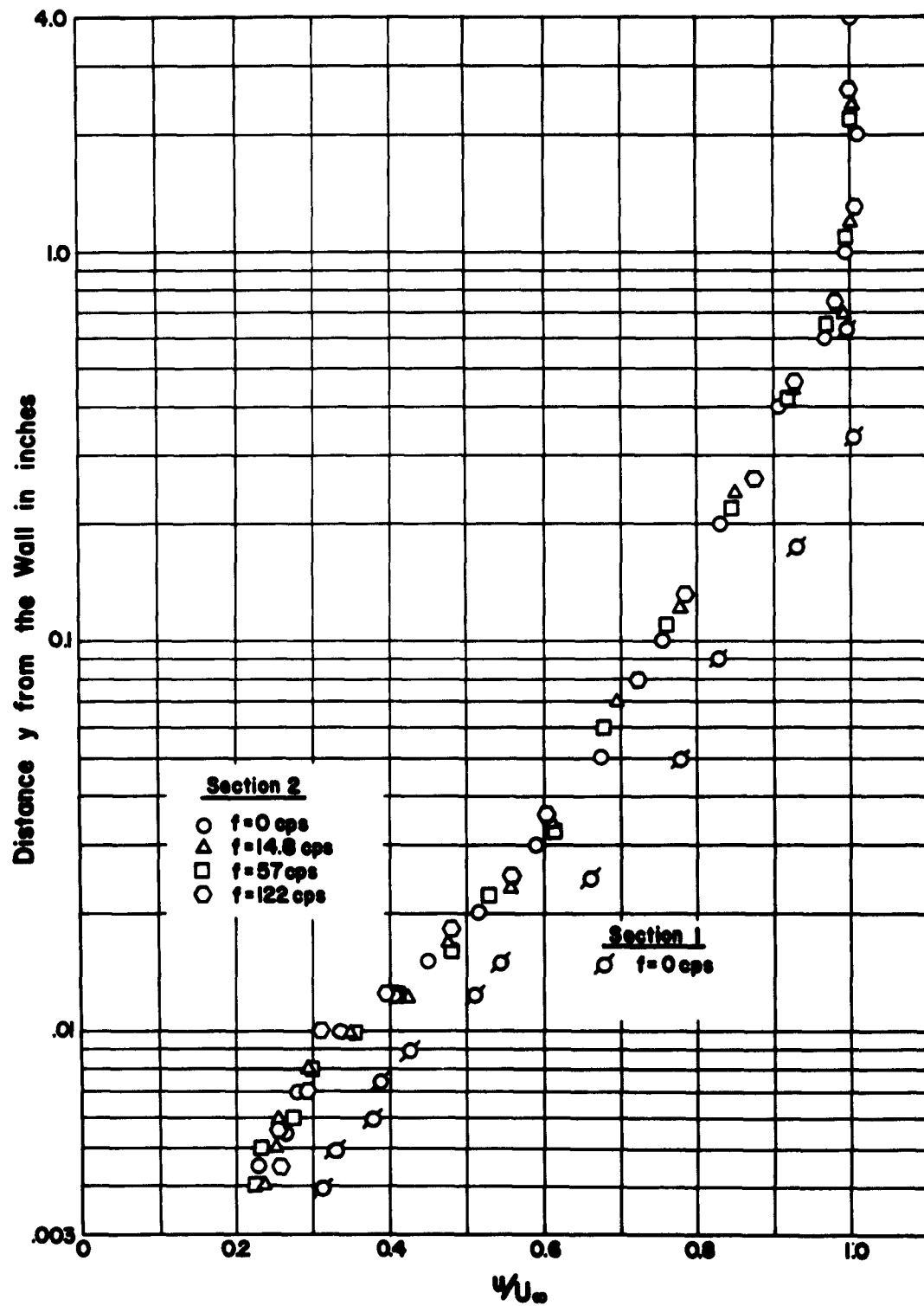
Fig. 10 - Boundary Layer Velocities, U_{\infty} = 2.4 fps
