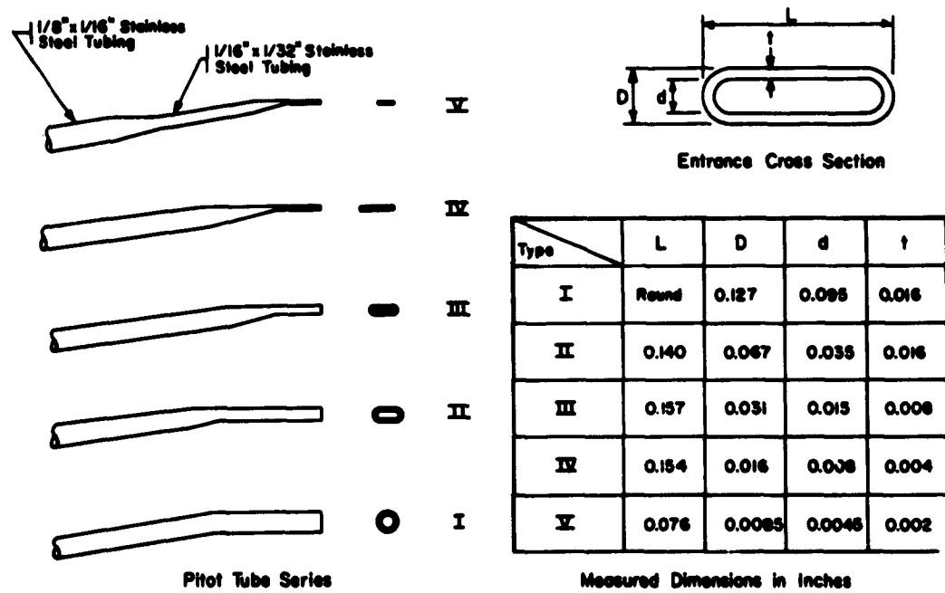
Fig. 6 - Boundary Layer Pitot Tubes and Assembly
