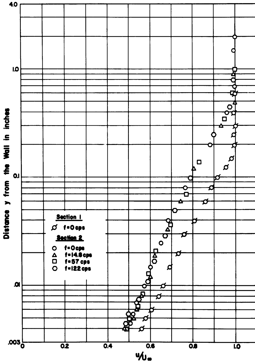
Fig. 12 - Boundary Layer Velocities, U_\infty = 15 fps
