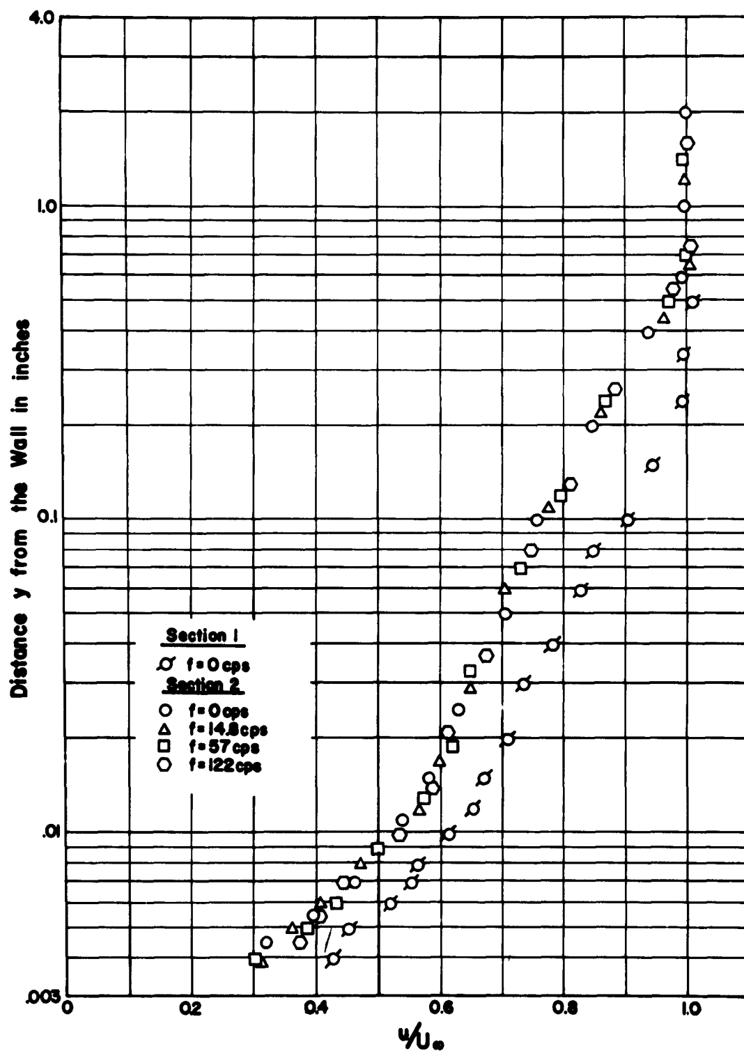
Fig. 11 - Boundary Layer Velocities, U_\infty = 6.0 fps
