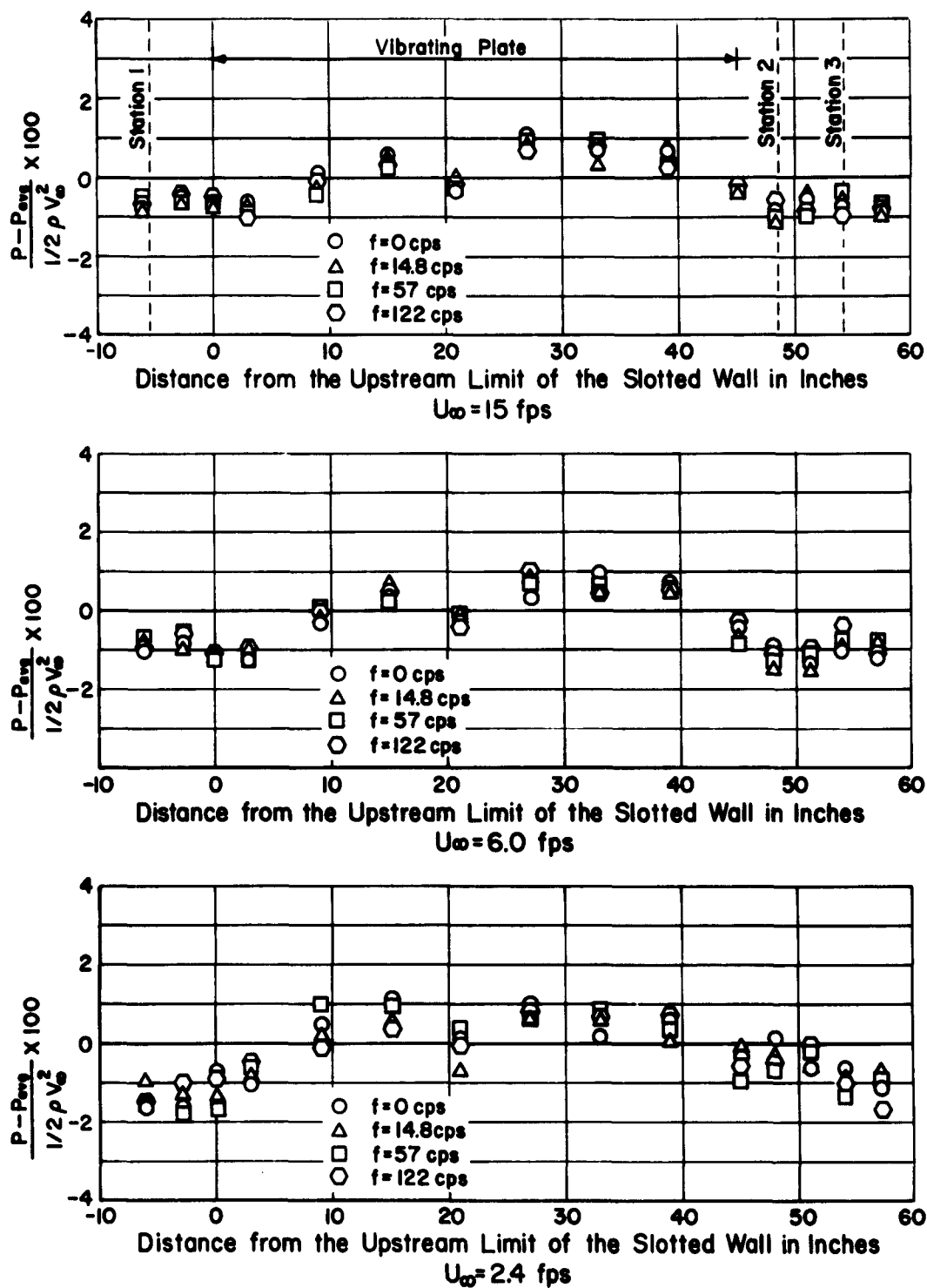
Fig. 9 - Measurements of the Longitudinal Pressure Gradient
