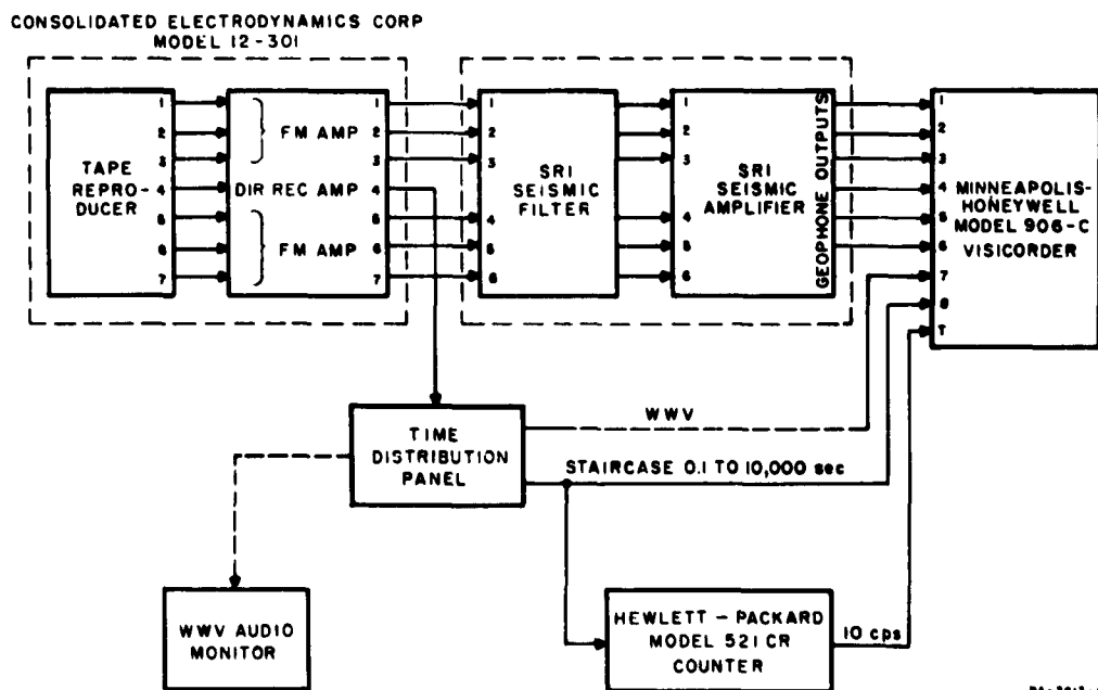
(b) PLAYBACK INSTRUMENTATION
