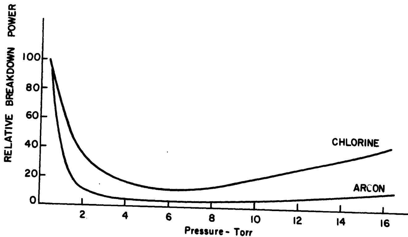
FIGURE 7B BREAKDOWN POWER VS PRESSURE
