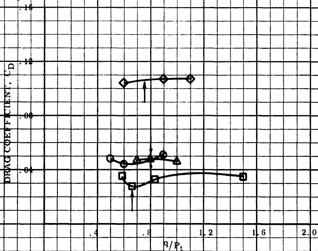
Figure 35 . Change of drag coefficient with increasing forward speed. Comparison of nose shapes, h/D = .035 , \alpha = 0^\circ
