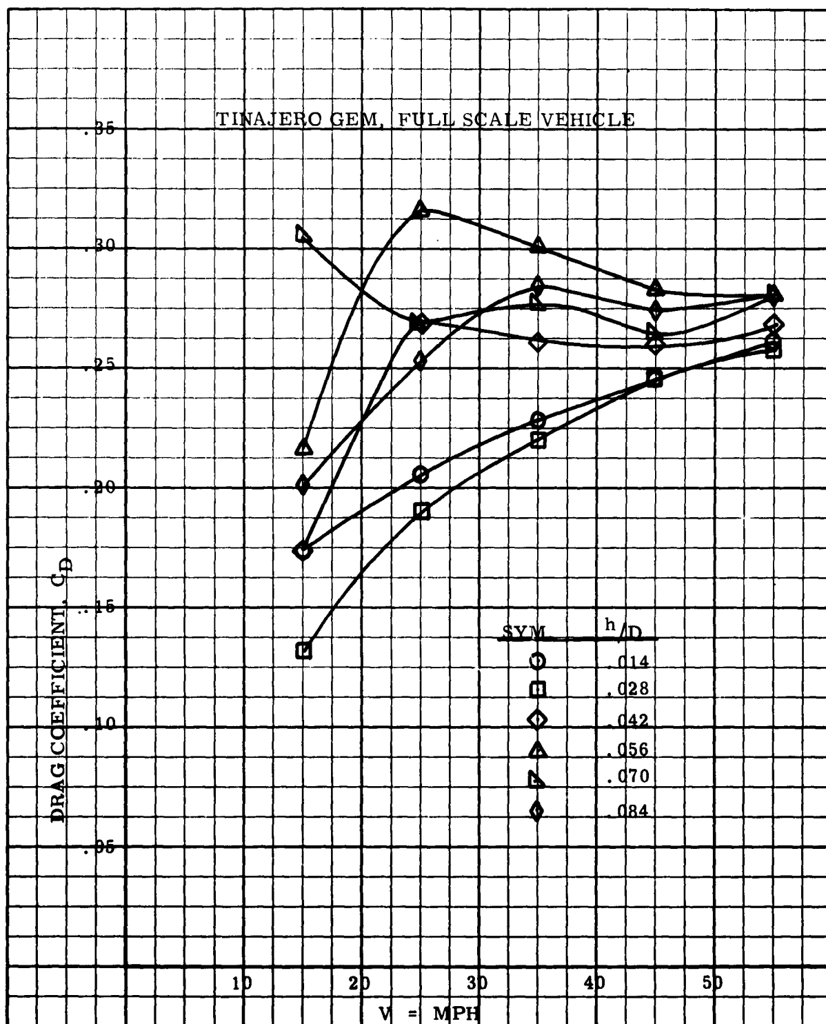
Figure 60 Drag coefficient vs. velocity, full scale vehicle, power off, \alpha = 0^\circ . Comparison of h/D ratios.
