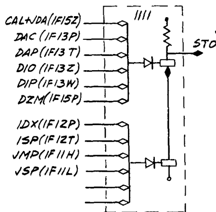
FIG. 5.10 - MODIFICATIONS TO PDP-I AND TRAP BREAK SYSTEM
