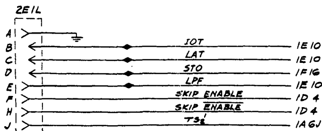
FIG. 5.11 - INTERCONNECTING WIRING
