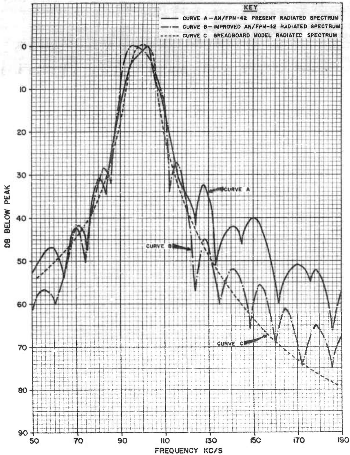
FIGURE 13 LORAN-C SPECTRUM
