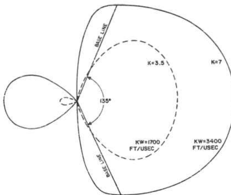
FIGURE 31 CONSTANT GEOMETRIC ACCURACY CONTOURS
