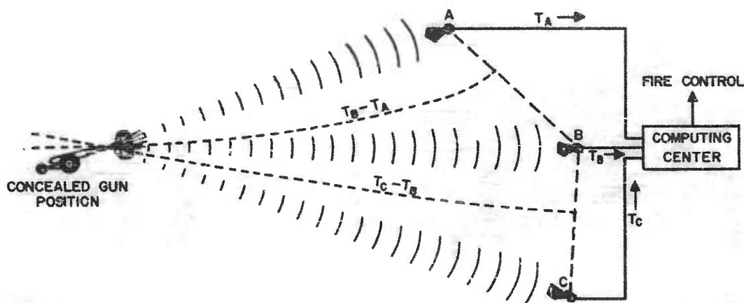
FIGURE 1 A HYPERBOLIC AUDIO LOCATION SYSTEM
