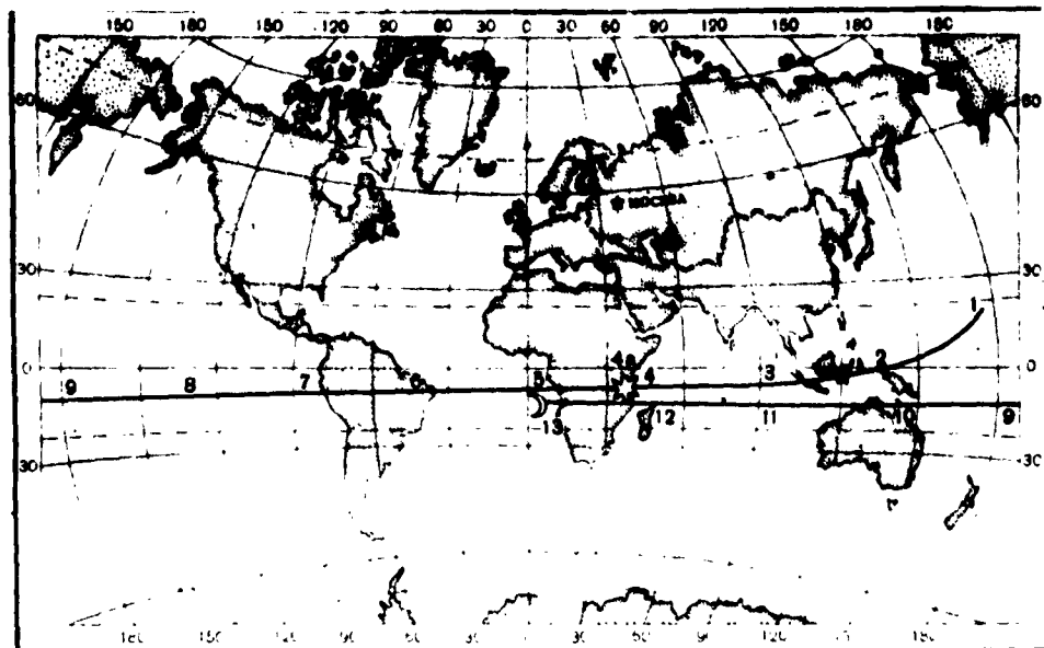
Fig. 104. Route of the Second Soviet Cosmic Rocket on the surface of the Earth
