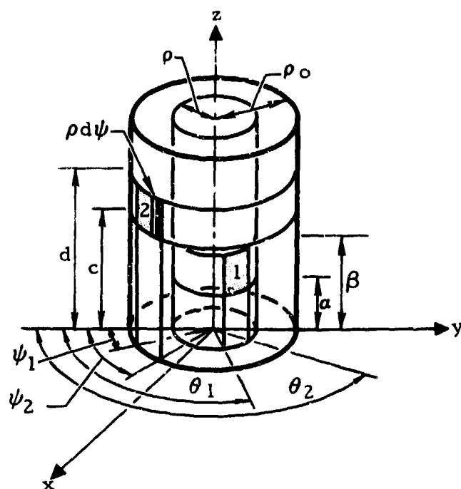
Figure 65. Nodes on Concentric Cylinders
