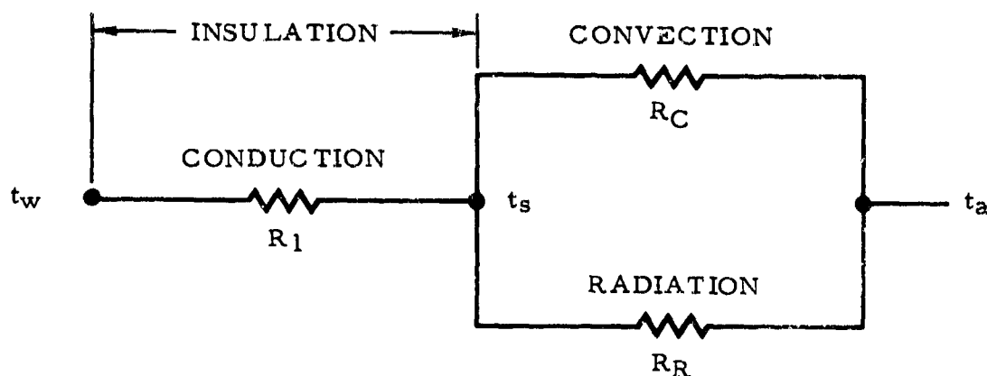
Figure 47. Thermal Network for Insulated Wire
