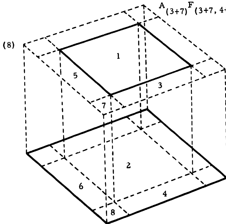
Figure 76. Diagrams of Configuration Factor Algebra (Sheet 2 of 2)
