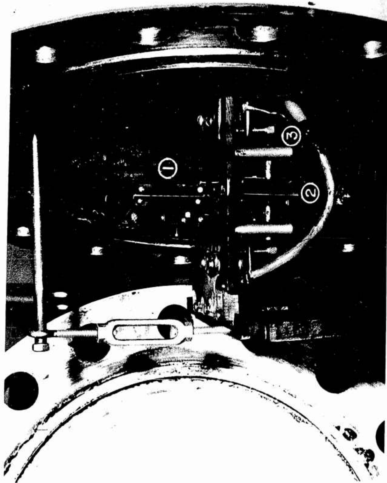
Fig. 2. Exploding Wire Mount - 1., 2. upper and lower slits, 3. wire holder.
