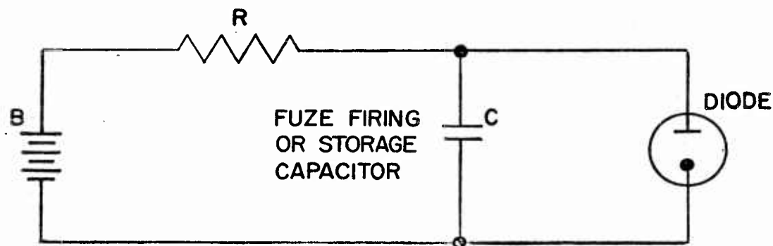
Figure 1. Basic diode nuclear proofing circuit.
