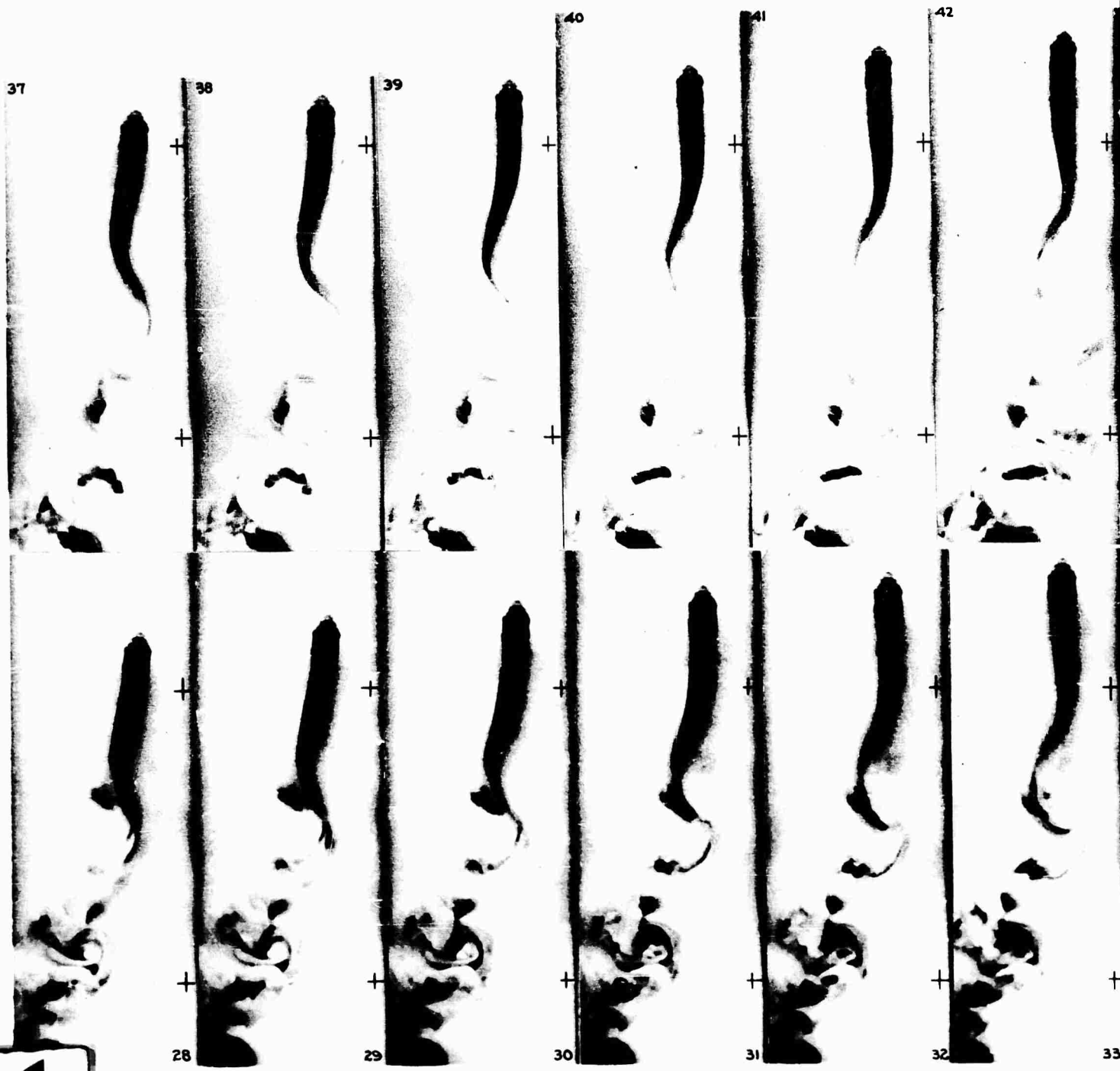
FIG. 11. Run II Continued. This is not a Karman
