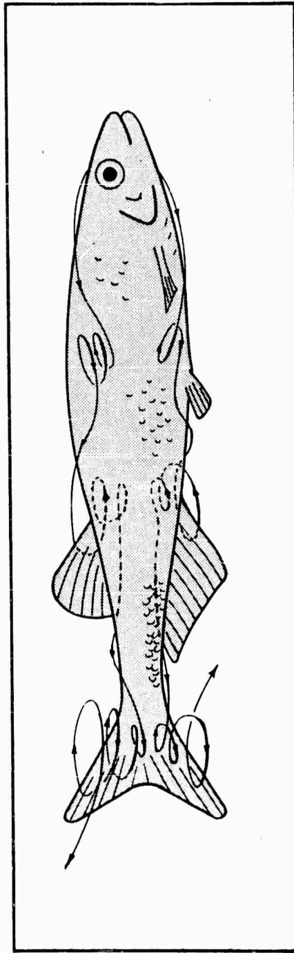
FIG. 37. Possible Hourglass Vortex Structure, Spiraling Away From Fish Center.
