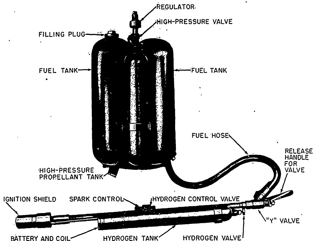
FIGURE 1. M1A1 portable flame thrower.
