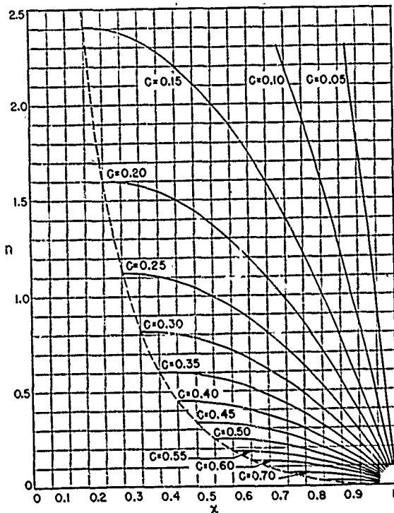
FIGURE 5. Values of n = \frac{1 - 2c + 2cx - x^2}{2c} .
