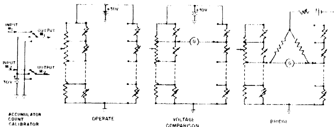
Fig. 16.14 Block diagram of accumulator calibrator unit
