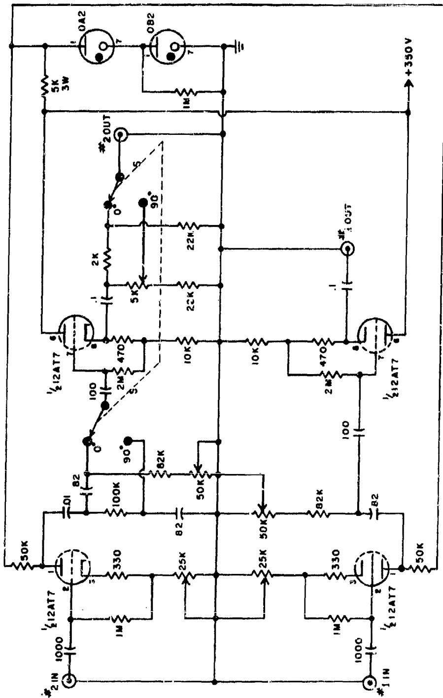
Fig. 14.28 20-kc amplifiers and phase shifters, schematic circuit diagram
