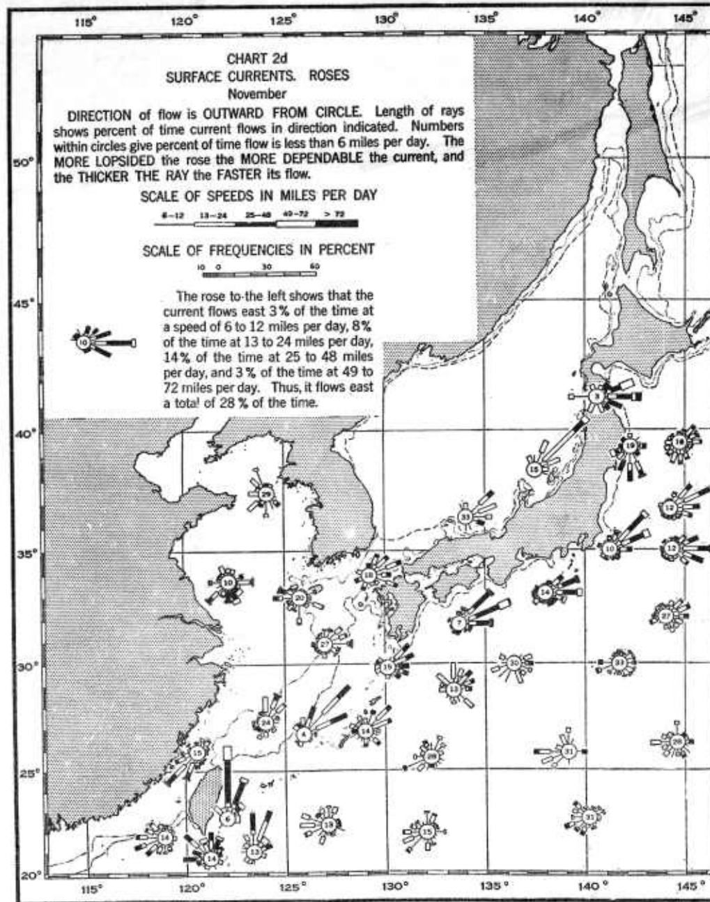
FIGURE 3. A part of Chart 2d from the Submarine Supplement to the Sailing Directions, Japanese Empire Area, H. O. Pub. No. 281, illustrating surface currents by means of roses.
