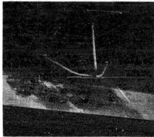
FIGURE 8. Thermocouple of the Model OCO bathythermograph installed at the level of the bilge keel.
