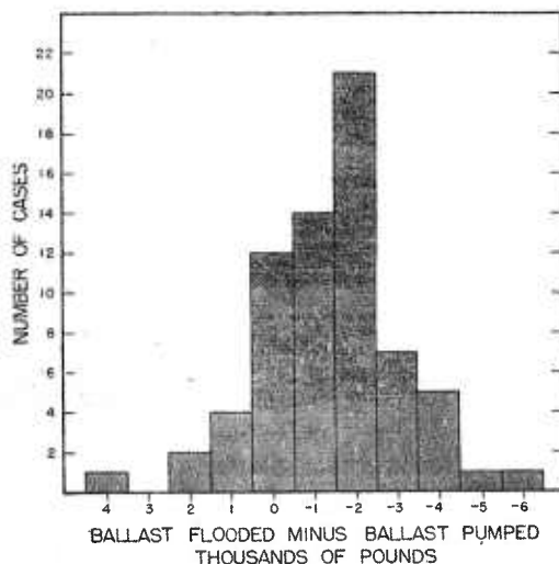
FIGURE 1. Frequency distribution of difference between ballast change on descent and on subsequent ascent by submarines in service. Ordinate—number of cases; abscissa—class intervals of 1,000 lb difference.
