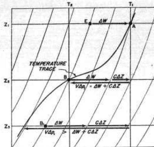
FIGURE 14. Use of graphical method to determine depth at which a submarine may come to trim when ballast is flooded in.
