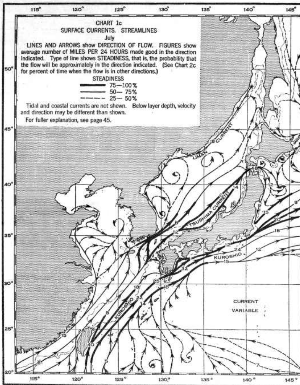
FIGURE 2. A part of Chart 1c from the Submarine Supplement to the Sailing Directions, Japanese Empire Area, H. O. Pub. No. 231, illustrating surface currents as streamlines.
