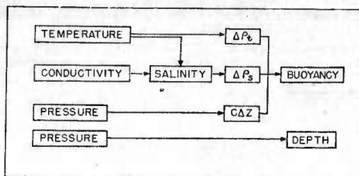
FIGURE 16. Arrangement of components of model CXJC buoyancy recorder.
