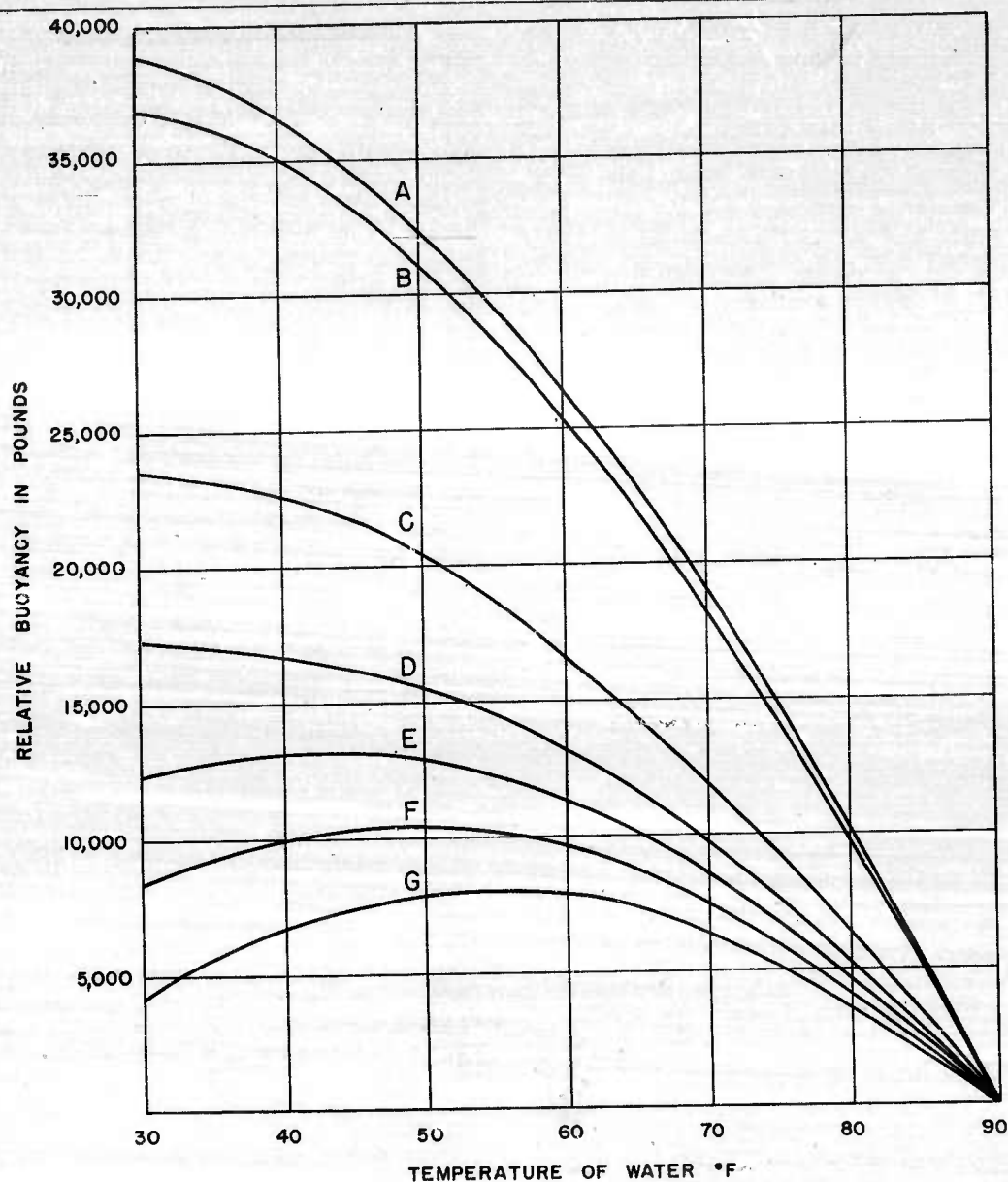
FIGURE 4. Effect of temperature on the buoyancy of a submarine of 2,100 tons submerged displacement:
