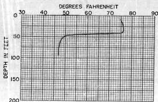
FIGURE 6. Exceptionally strong negative temperature gradient recorded by bathythermograph of a U. S. submarine in the Yellow Sea in September.
