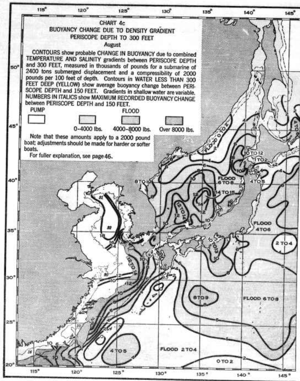
FIGURE 5. A part of Chart 4c from the Submarine Supplement to the Sailing Directions, Japanese Empire Area, H. O. Pub. No. 231, illustrating buoyancy change due to density gradient between periscope depth and 300 feet.
