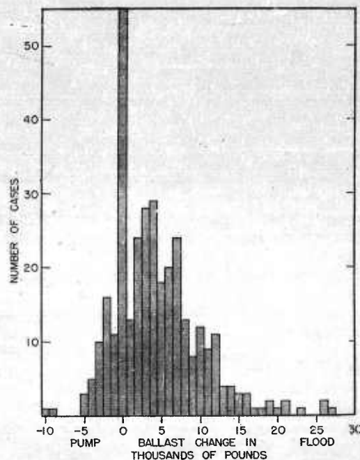
FIGURE 2. Frequency distribution of ballast changes made in deep dives by fleet-type submarines in service.
