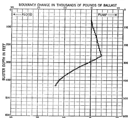
FIGURE 20. Chart used in model CXJC buoyancy recorder showing simulated buoyancy trace. Reduced to \frac{1}{2} natural size.
