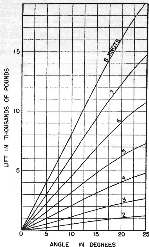
FIGURE 2. Vertical force developed by bow planes, assuming total area of 124 square feet, as function of their angle and the speed.
