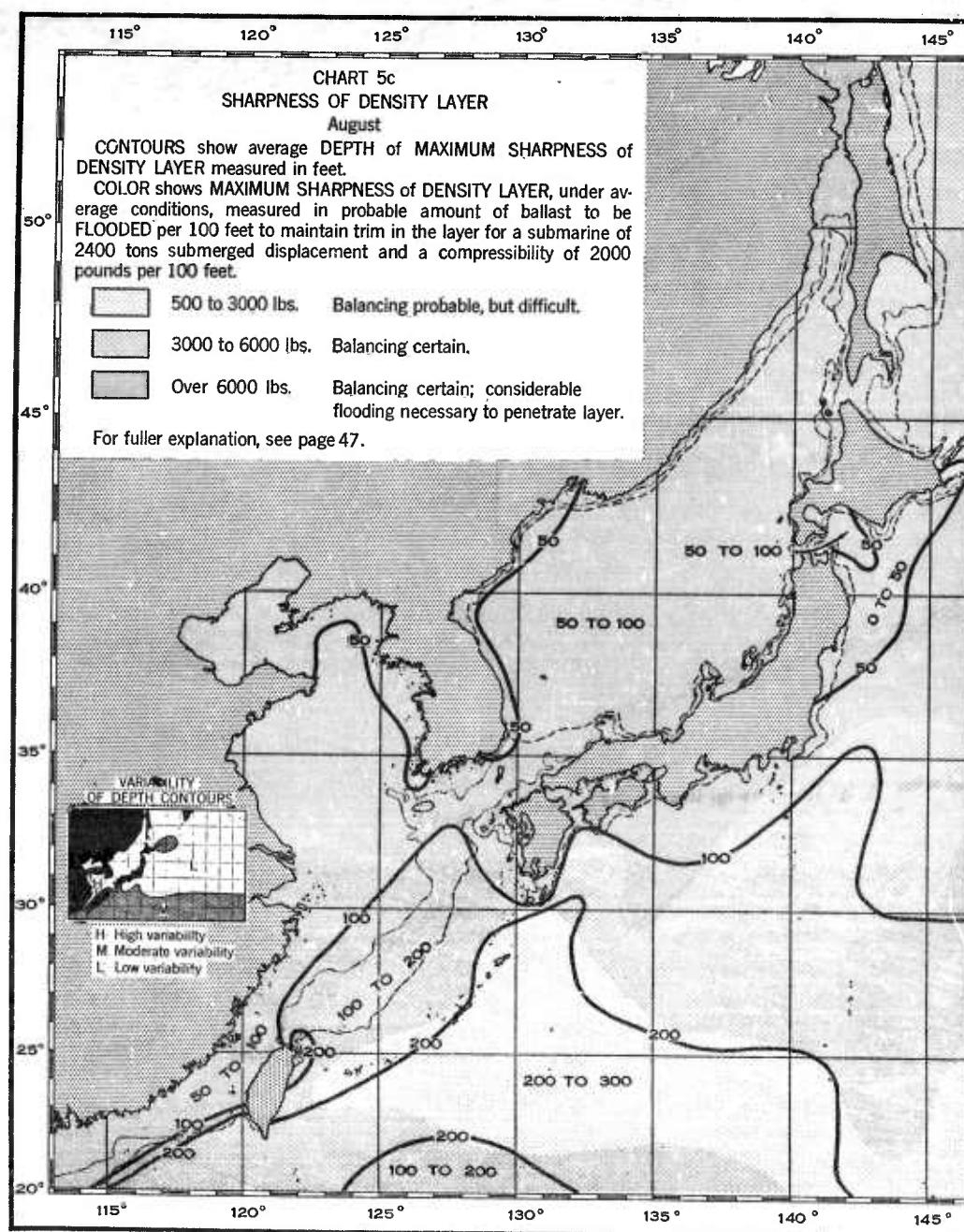
FIGURE 3. A part of Chart 5c from the Submarine Supplement to the Sailing Directions, Japanese Empire Area, H. O. Pub. No. 231, illustrating sharpness of the density layer.
