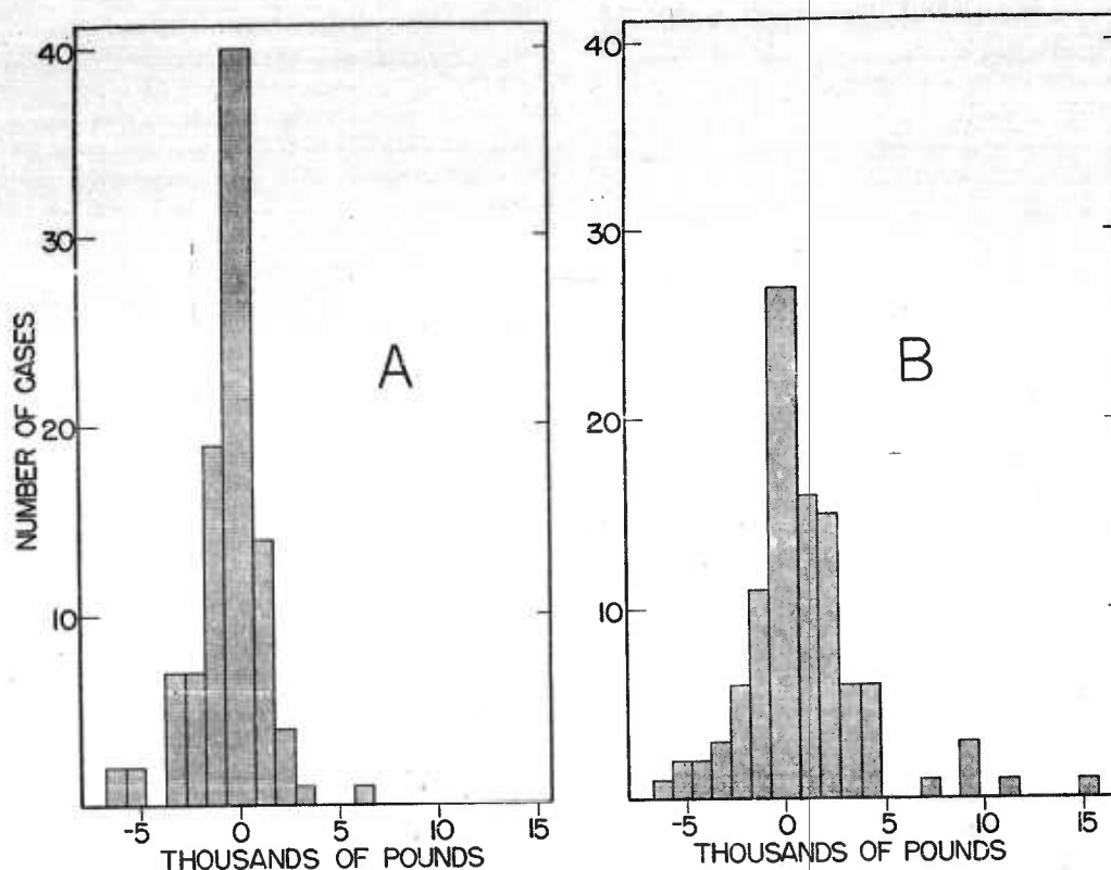
FIGURE 15. Frequency distribution of errors in bathythermograph predictions made by submarines in service.
