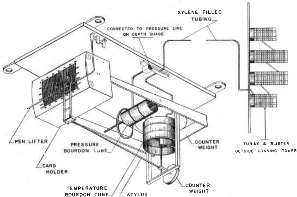
FIGURE 1. Diagram showing principles of construction of Type CTB bathythermograph.
