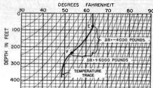
FIGURE 12. Example of temperature trace which crosses isoballast lines from right to left in descent, in which case buoyancy increases on increasing depth.
