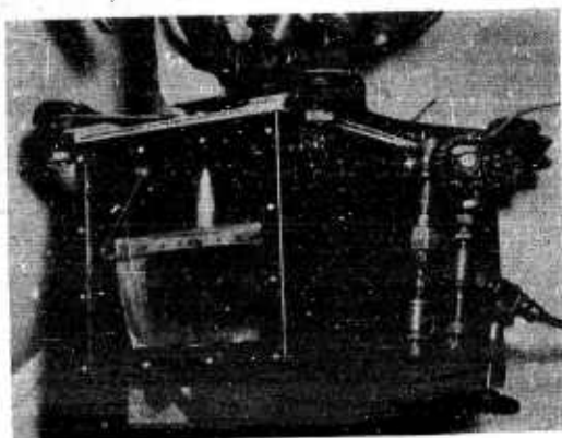
FIGURE 2. Type CTB bathythermograph installed.
