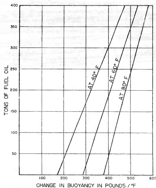
FIGURE 3. Relation between quantity of fuel oil carried and the change in buoyancy, as a result of cooling, of a submarine of 2,400 tons submerged displacement. Complete thermal equilibrium between the sea water and the contents of the ballast tanks is assumed.
