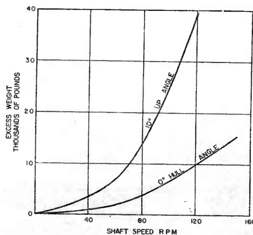
FIGURE 3. Effect of speed and hull angle in counterbalancing excess weight of a submerged fleet-type submarine, so as to permit control of depth of operation.
