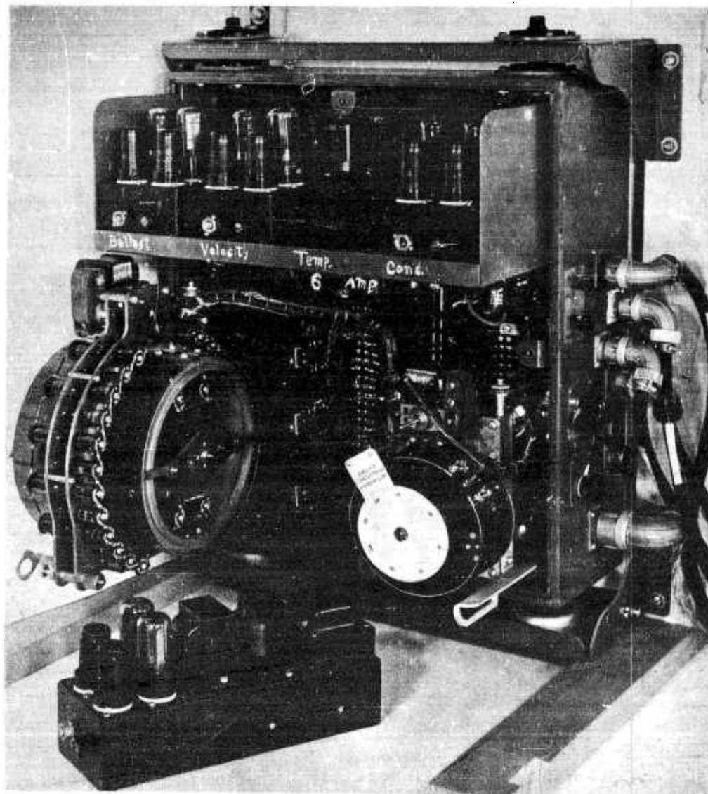
FIGURE 18. Model CXJC computing mechanism. The temperature bridge is swung out to give access to parts within. One amplifier has been removed.
