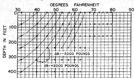
FIGURE 9. Method of constructing grid of isoballast lines on a bathythermograph chart. The example is for a submarine with compression of 2,500 lb per hundred feet.
