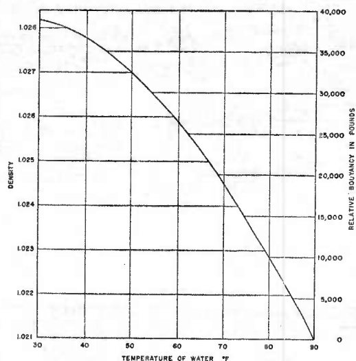
FIGURE 1. Effect of temperature on the density of sea water having a salinity of 35 ‰, and corresponding effect on buoyancy of a submarine of 2,400 tons submerged displacement.
