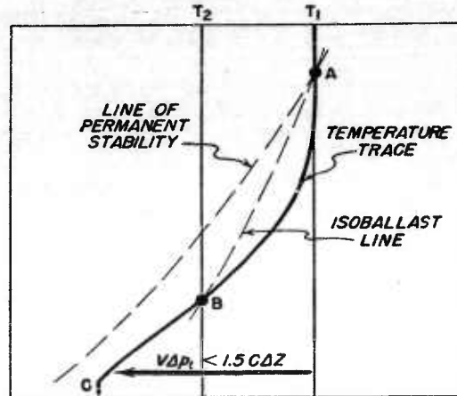
FIGURE 3. Diagram illustrating condition when permanent stability does not exist.
