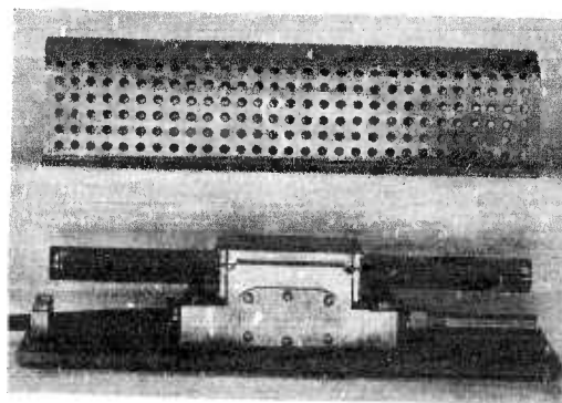
FIGURE 17. Measuring unit of model CXJC buoyancy recorder.
