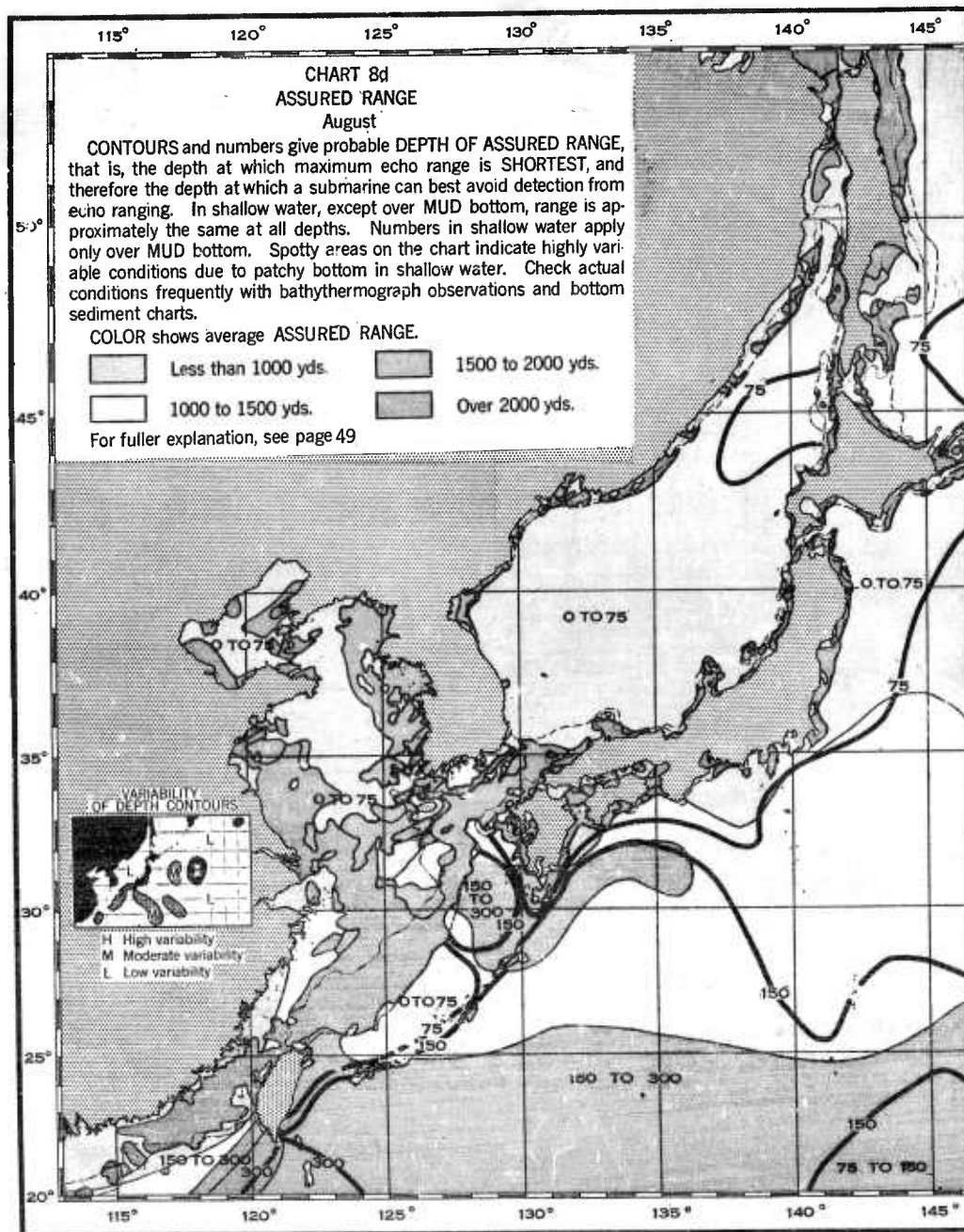
FIGURE 9. A part of Chart 8d from the Submarine Supplement to the Sailing Directions, Japanese Empire Area, H. O. Pub. No. 231, illustrating assured range.
