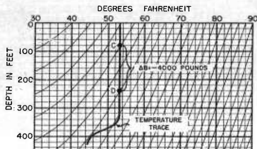
FIGURE 11. Example of temperature trace which crosses the isoballast lines from left to right on descent, in which case buoyancy decreases on increasing depth.
