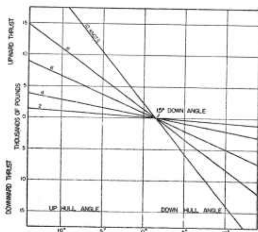
FIGURE 1. Vertical component of propeller thrust of a fleet-type submarine as a function of speed and of hull angle. It is assumed that the propeller shaft is inclined to the water line by 1.5 degrees.
