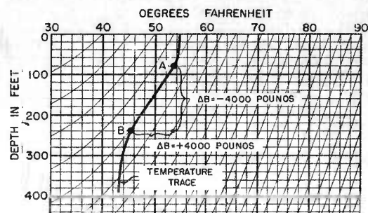
FIGURE 10. Example of temperature trace which follows an isoballast line, in which case no change in buoyancy occurs on changing depth.
