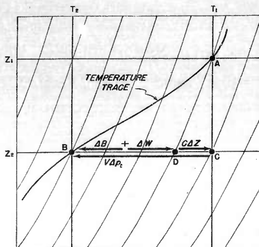
FIGURE 13. Graphical representation of factors affecting buoyancy with the aid of temperature trace drawn on isoballast line grid.
