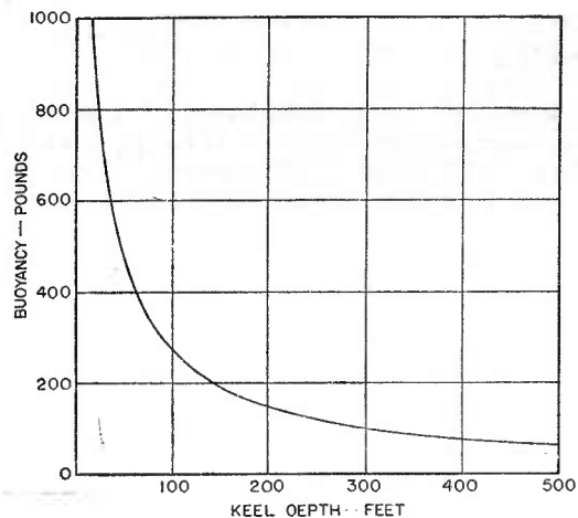
FIGURE 1. Effect of a volume of entrapped air, which at atmospheric pressure displaces 1,000 lb of sea water, on the buoyancy of a submarine at various keel depths.
