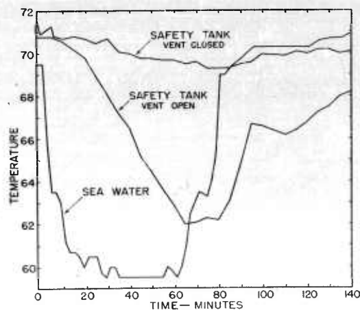
FIGURE 5. Temperature of ballast water in safety tanks, with vents open and closed, during deep submergence in a negative temperature gradient and after return to periscope depth.
