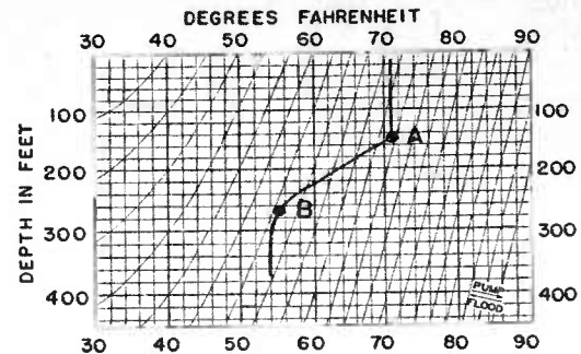
FIGURE 1. Temperature trace illustrating condition when immediate stability exists between depths A and B.
