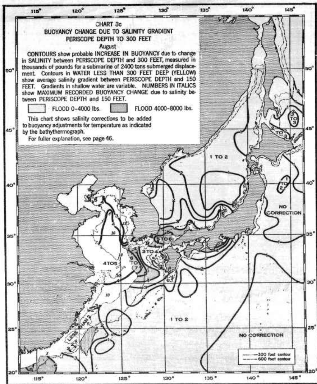
FIGURE 4. Chart 3c from the Submarine Supplement to the Sailing Directions, Japanese Empire Area, H. O. Pub. No. 231, illustrating buoyancy change due to salinity gradient between periscope depth and 300 feet.
