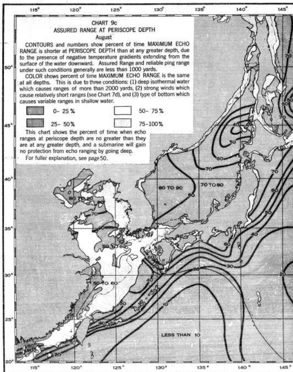
FIGURE 10. A part of Chart 9c from the Submarine Supplement to the Sailing Directions, Japanese Empire Area, H. O. Pub. No. 231, illustrating assured range at periscope depth.
