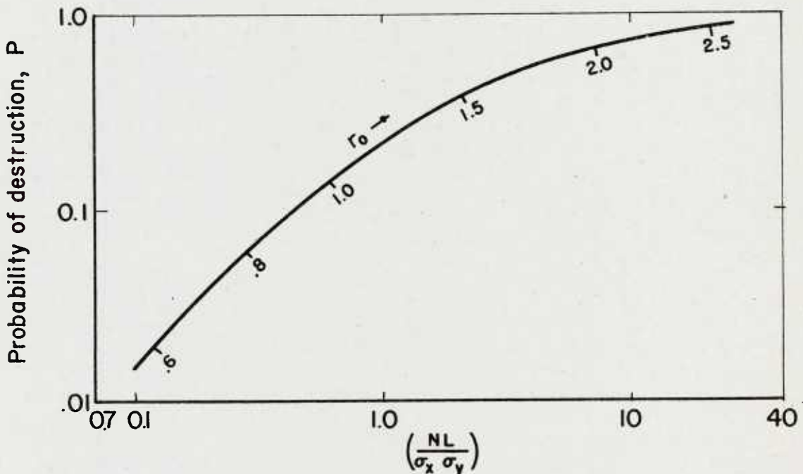
Figure 44. Probability of destruction and size of pattern as function of number of projectiles; two dimensions.
