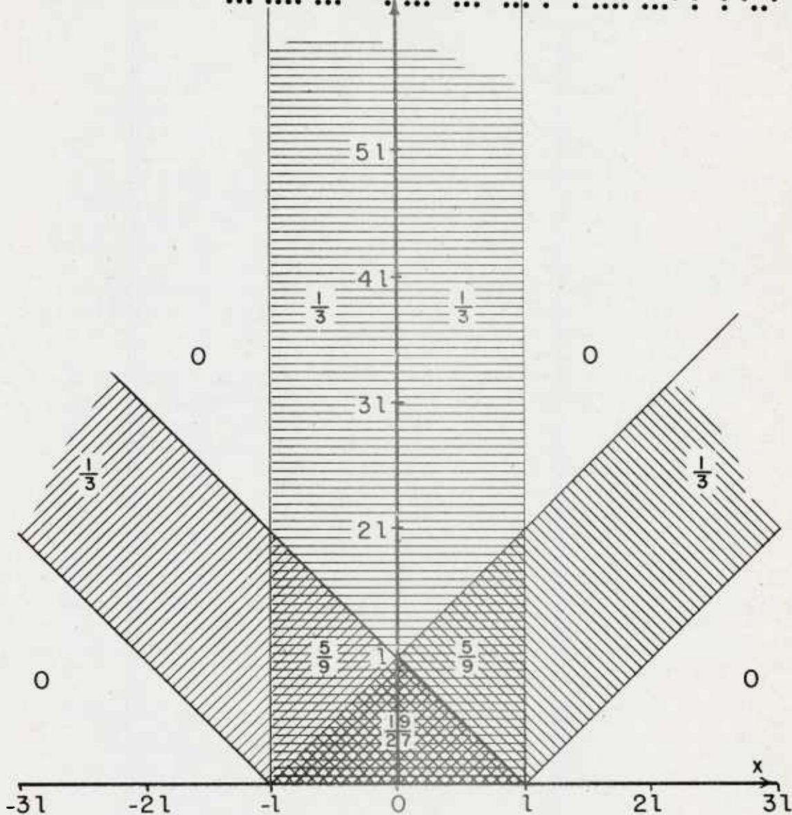
Figure 34. Damage function for spread of three torpedoes. No ballistic dispersion.
