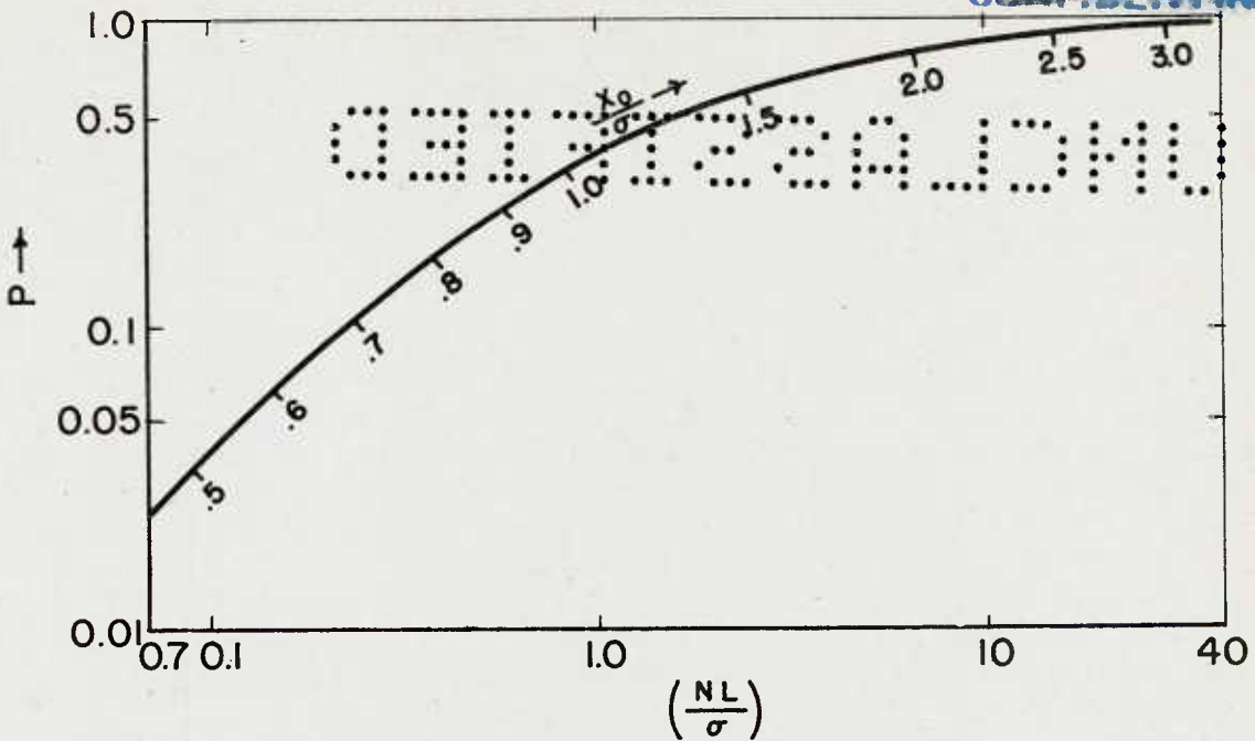
Figure 43. Probability of destruction and size of pattern as function of number of projectiles; one dimension.
