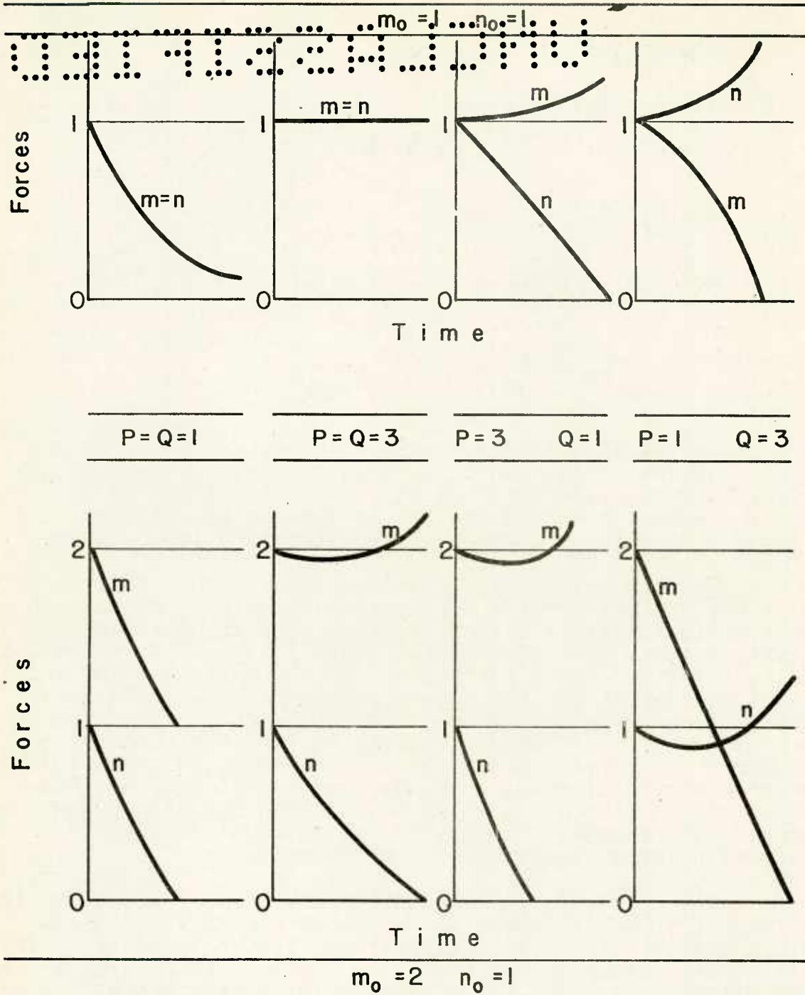
Figure 16. Solutions of the generalized Lanchester equations for a = b = 2 , c = d = 1 ; for different productive capacities P and Q , and different initial forces
