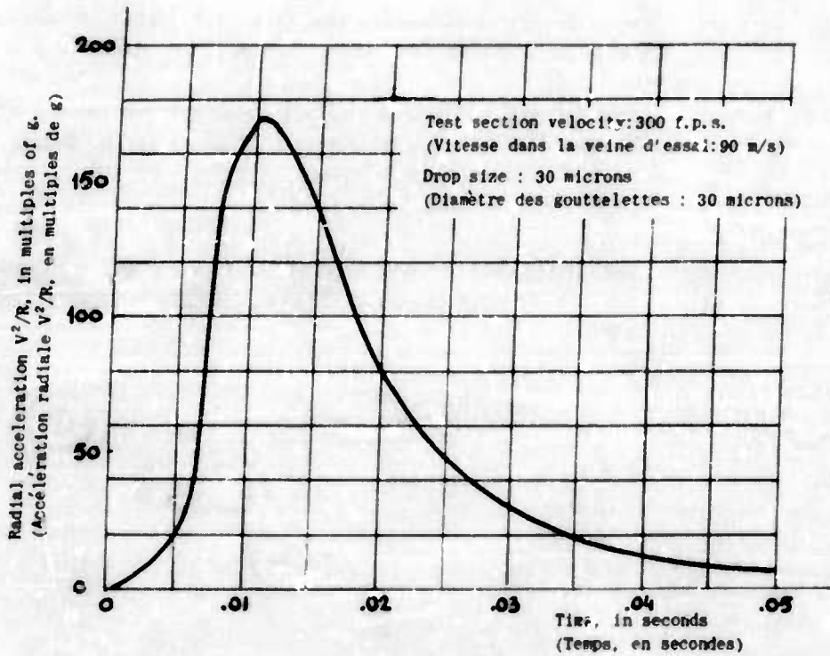
Fig. 1 Centrifugal acceleration of a drop versus time in traversing the inlet nozzle
