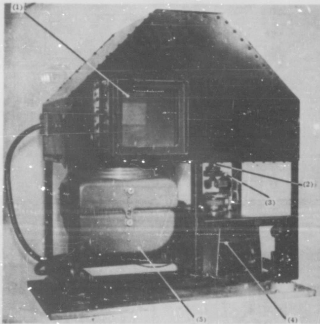
(1) Focusing Screen. (Ecran de mise au point) (4) Light Source. (Source d'éclairage) (2) Lens (Lentille) (5) Film Magazine. (Magasin à film) (3) Slide Holder. (Support de la lame)
