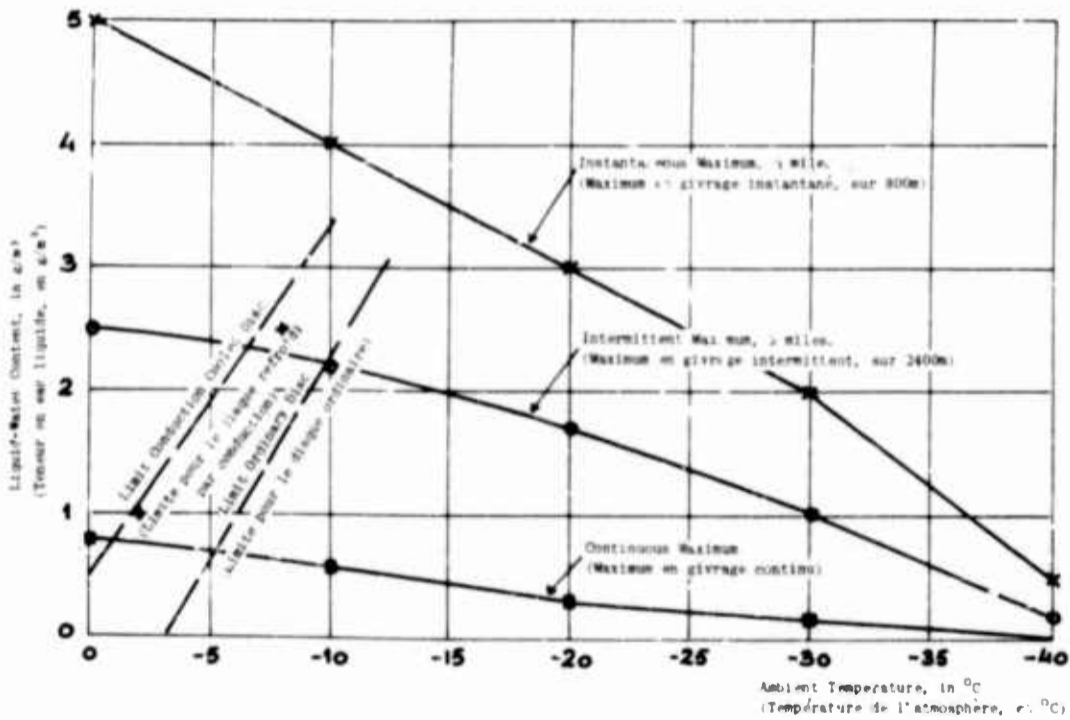
Fig. 19 Temperature and liquid-water content relationships, together with limits of rotating discs
