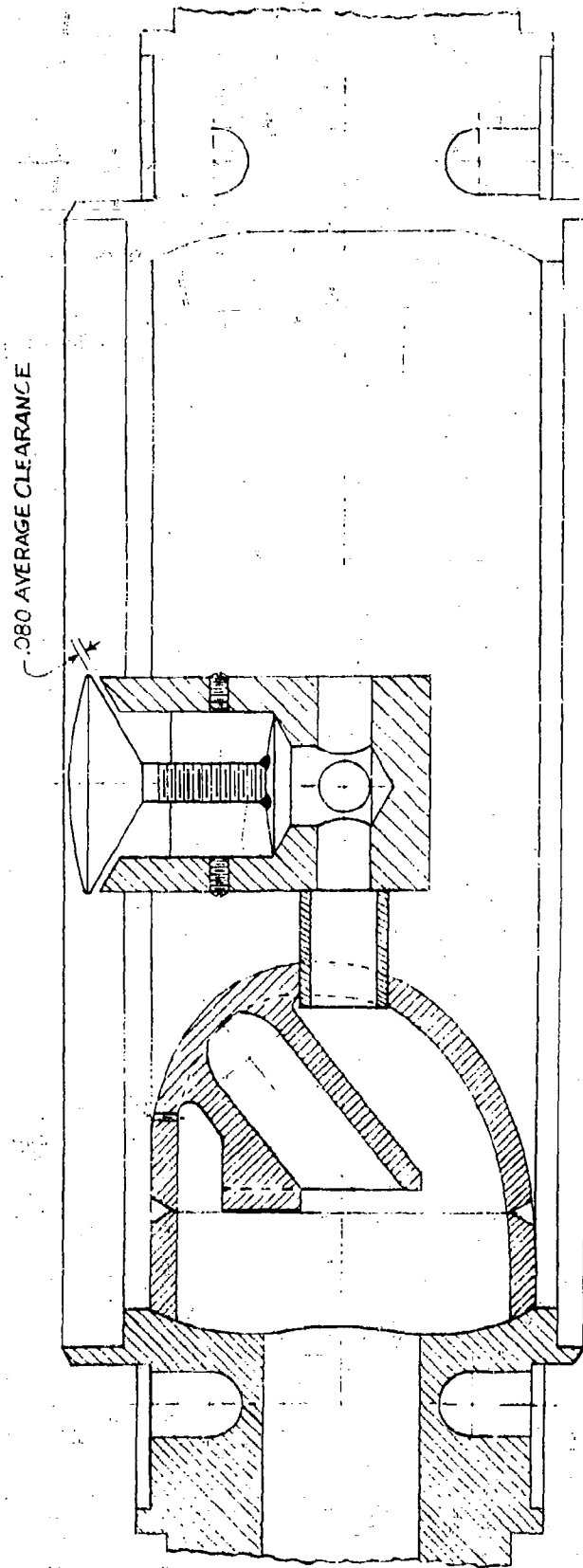
BECCO DESIGNED UMBRELLA TYPE SINGLE DILUENT WATER NOZZLE AS MOUNTED IN THE CC-12 CHAMBER FOR TEST RUNS #63-64-12B
