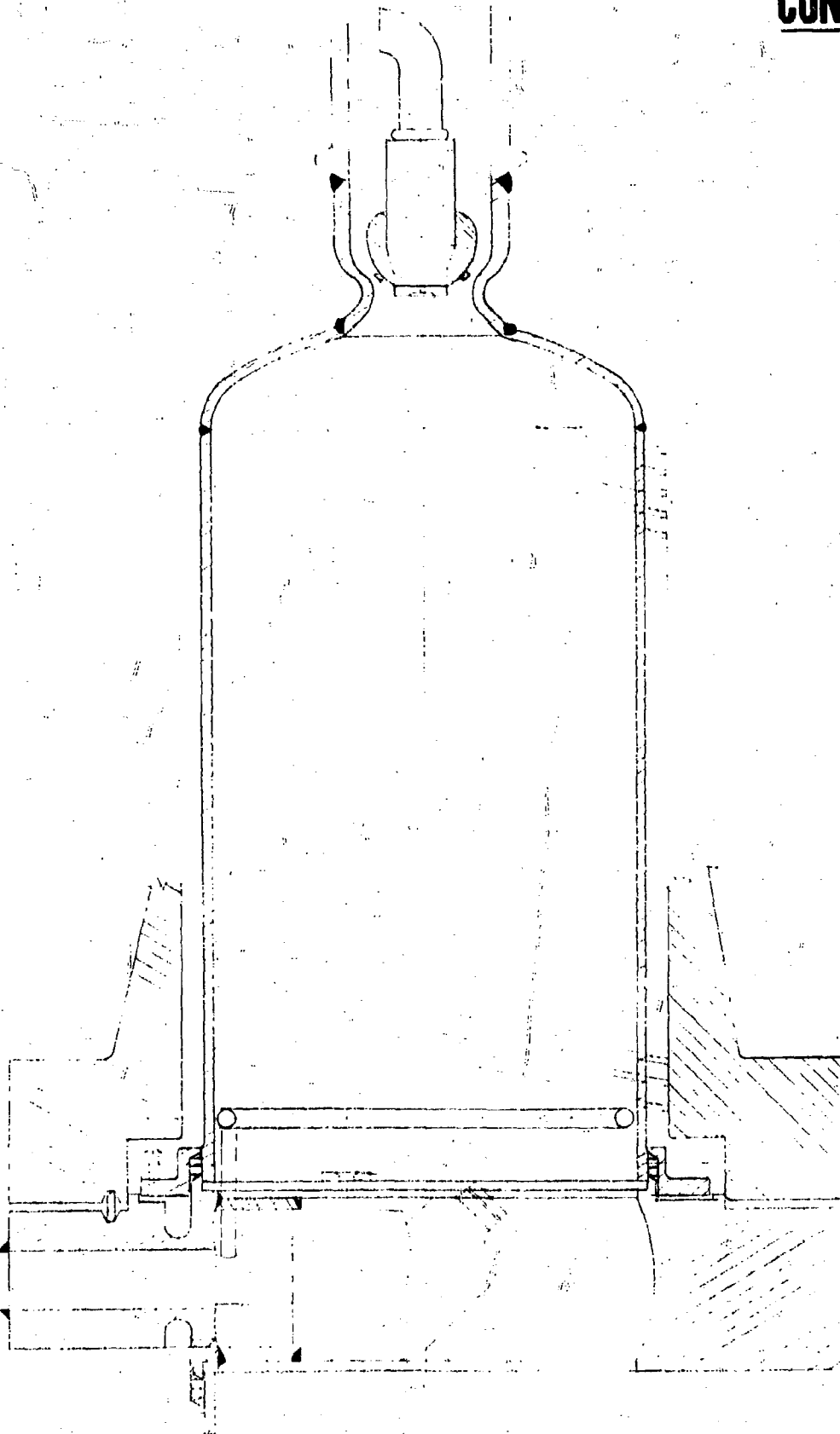
MODIFIED CC-12 COMBUSTION CHAMBER INCORPORATING A WATER SPRAY RING AT THE UNCOOLED LINER PACKING SECTION
