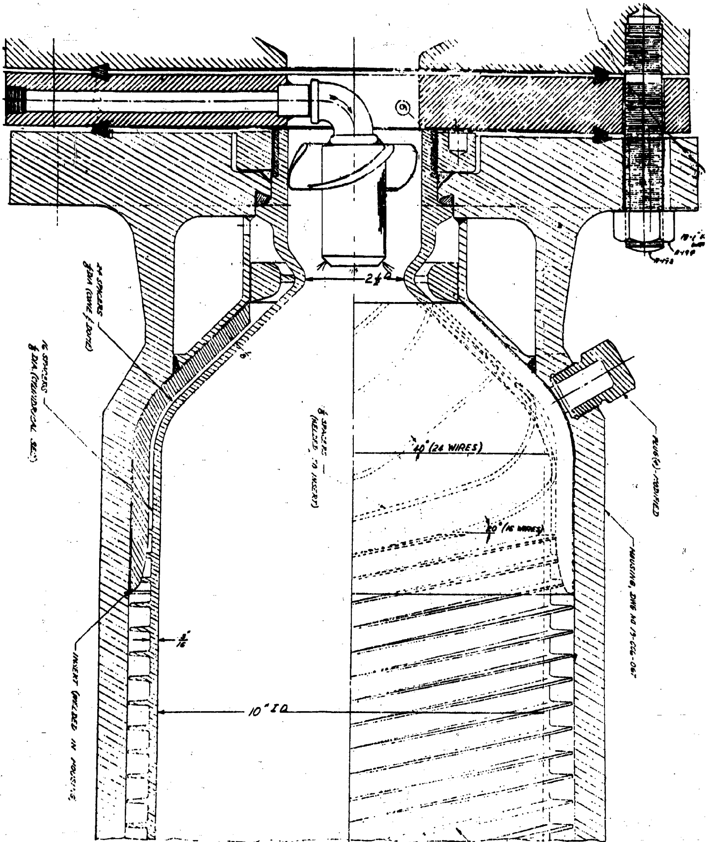
MODIFIED LINER IN ALLIS CHALMERS 10 x 16 COMBUSTION CHAMBER (CC-12 CHAMBER.)
