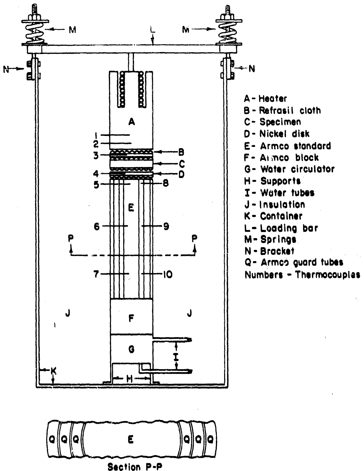
FIGURE 1. THERMAL-CONDUCTIVITY APPARATUS FOR TRANSPARENT SOLIDS
