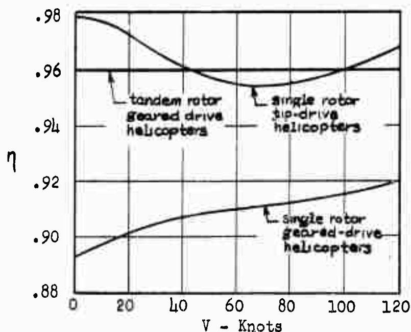
Figure 2-26: Propulsive Efficiency vs. V 40
