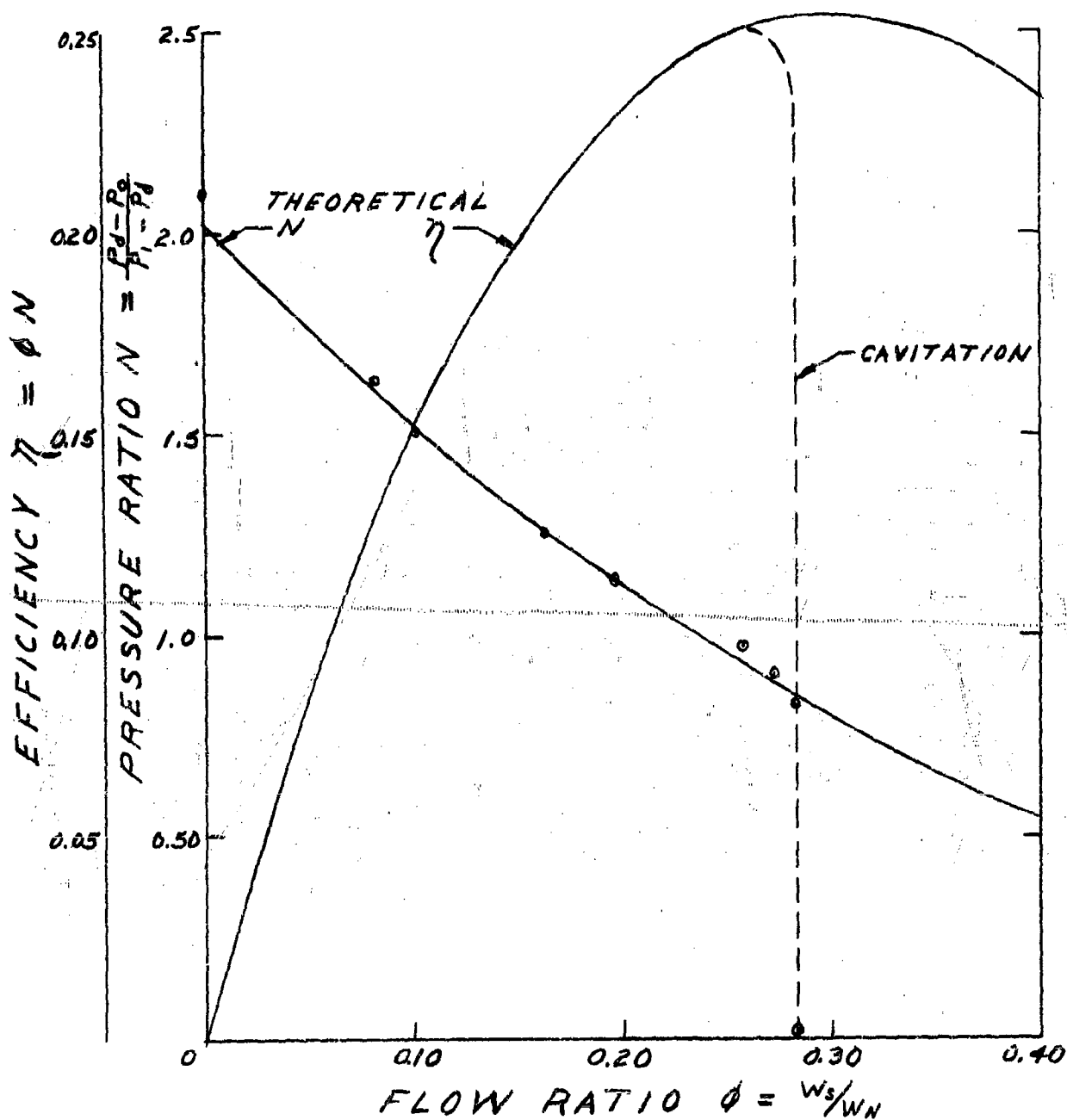
FIG. II EXPERIMENTAL N VALUES vs \phi , THEORY SHOWN AS SOLID LINE
